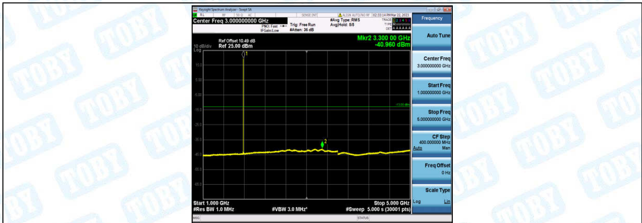
Band66-20MHz-16QAM-132572-1-0-High-1000-5000--40.96-PASS
