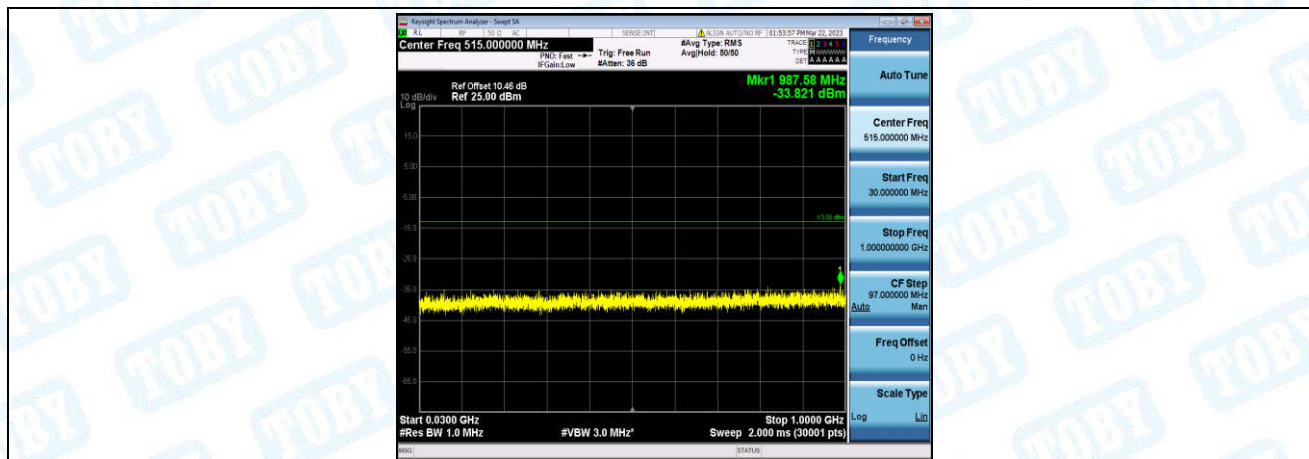
Band66-15MHz-16QAM-132047-1-0-Low-30-1000--33.82-PASS
