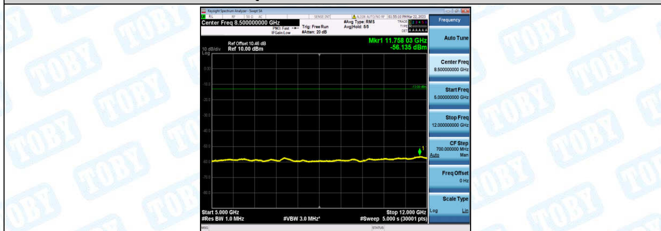
Band66-15MHz-16QAM-132047-1-0-Low-5000-12000--56.14-PASS
