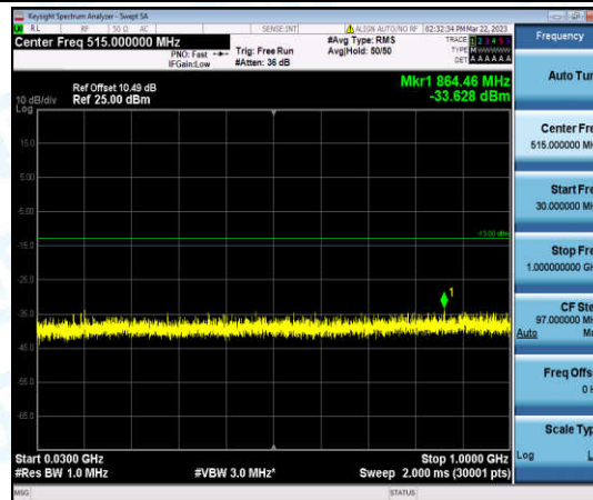
Band66-20MHz-16QAM-132572-1-0-High-30-1000--33.63-PASS
