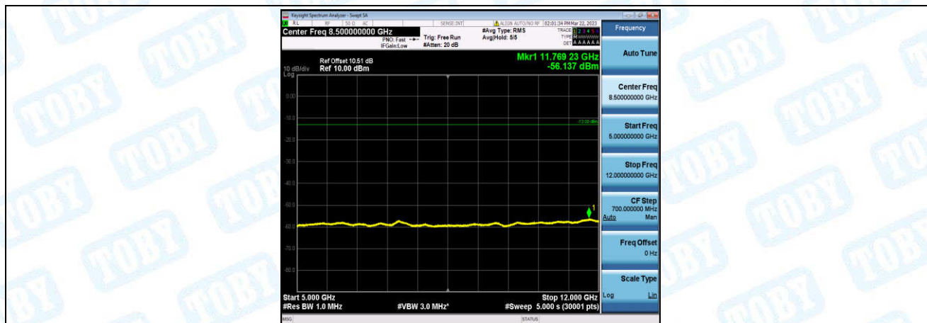
Band66-15MHz-16QAM-132322-1-0-Low-5000-12000--56.14-PASS
