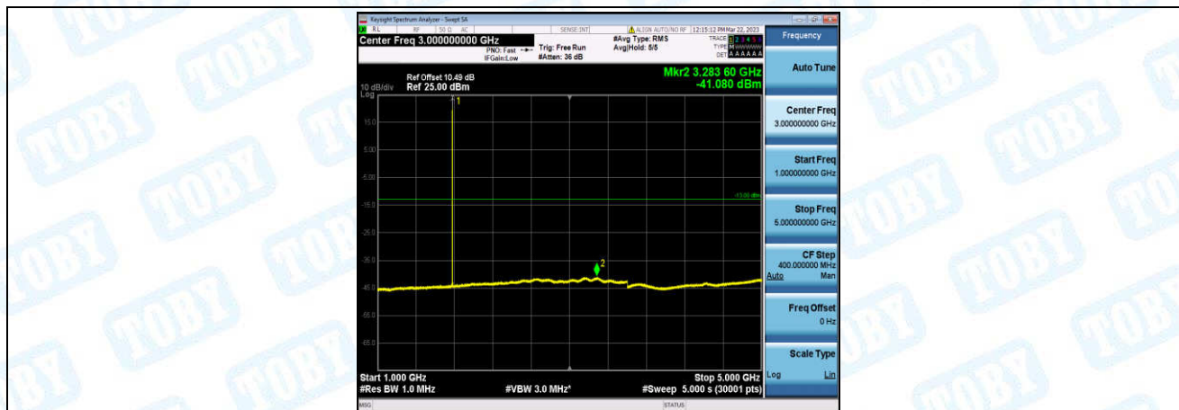
Band66-5MHz-QPSK-132647-1-0-High-1000-5000--41.08-PASS
