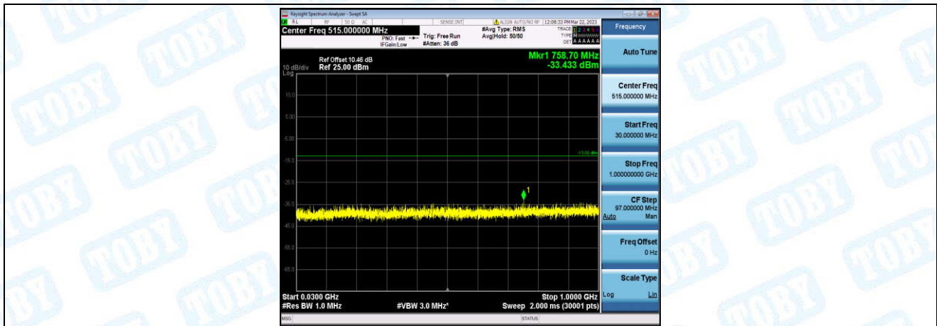
Band66-5MHz-16QAM-131997-1-0-Low-30-1000--33.43-PASS
