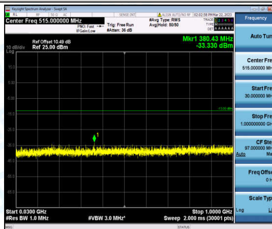
Band66-15MHz-QPSK-132597-1-0-High-30-1000--33.33-PASS
