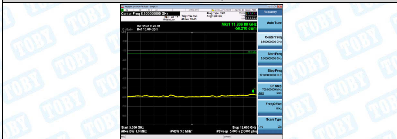
Band66-3MHz-16QAM-132657-1-0-High-5000-12000--56.21-PASS
