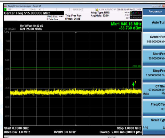
Band66-1.4MHz-16QAM-132665-1-0-High-30-1000--33.73-PASS
