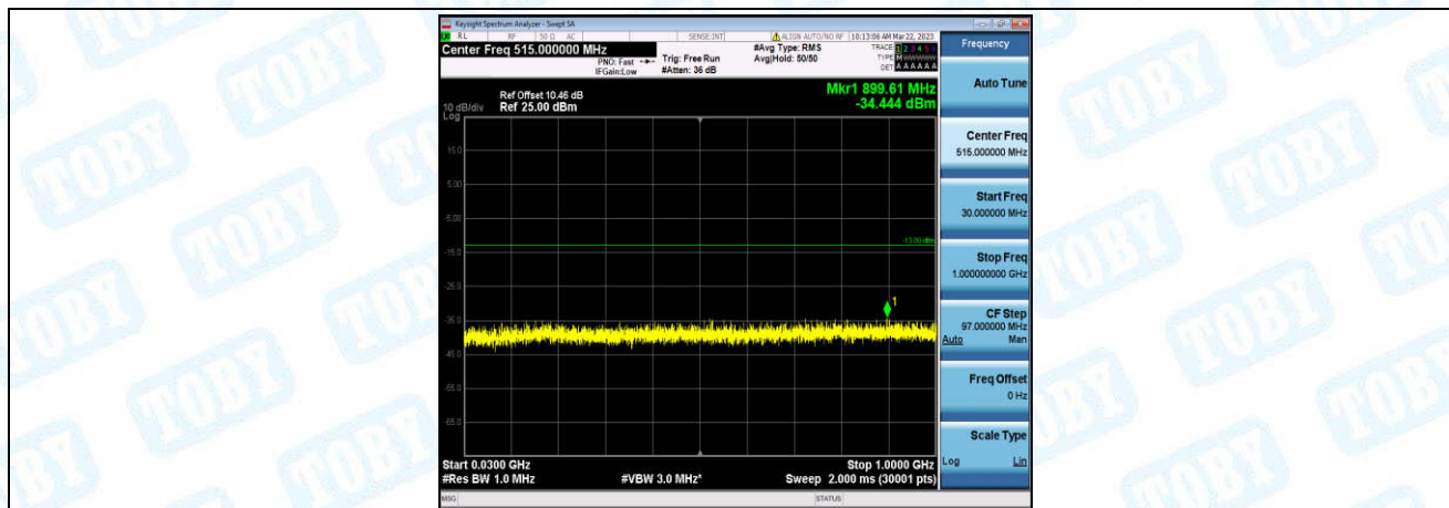
Band66-3MHz-16QAM-131987-1-0-Low-30-1000--34.44-PASS
