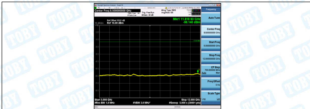
Band66-10MHz-QPSK-132322-1-0-Low-5000-12000--56.14-PASS
