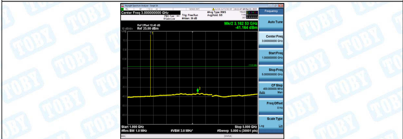
Band66-3MHz-QPSK-131987-1-0-Low-1000-5000--41.16-PASS
