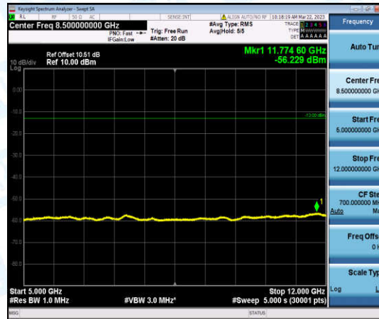
Band66-3MHz-16QAM-132322-1-0-Low-5000-12000--56.23-PASS
