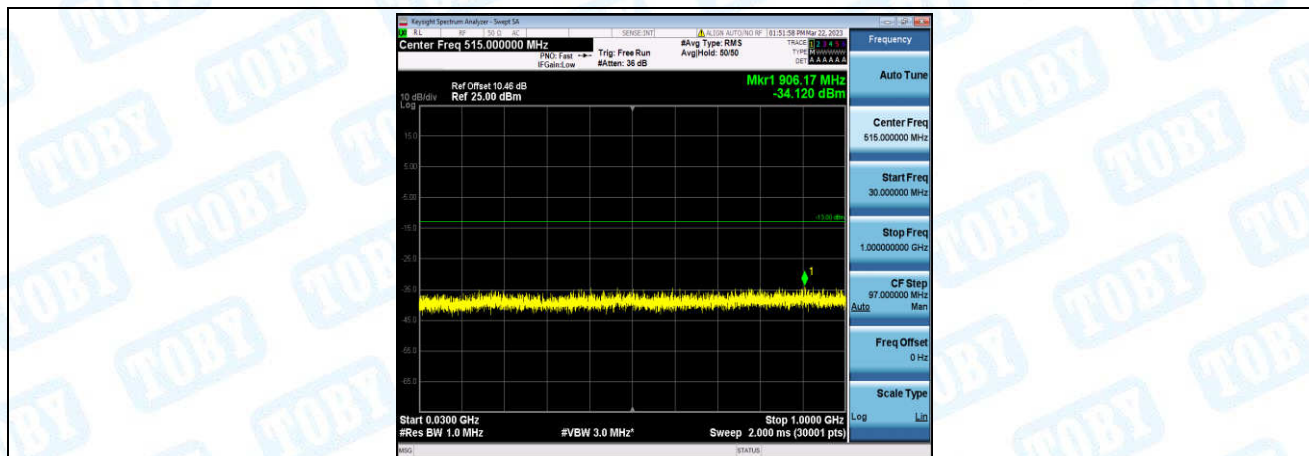
Band66-15MHz-QPSK-132047-1-0-Low-30-1000--34.12-PASS
