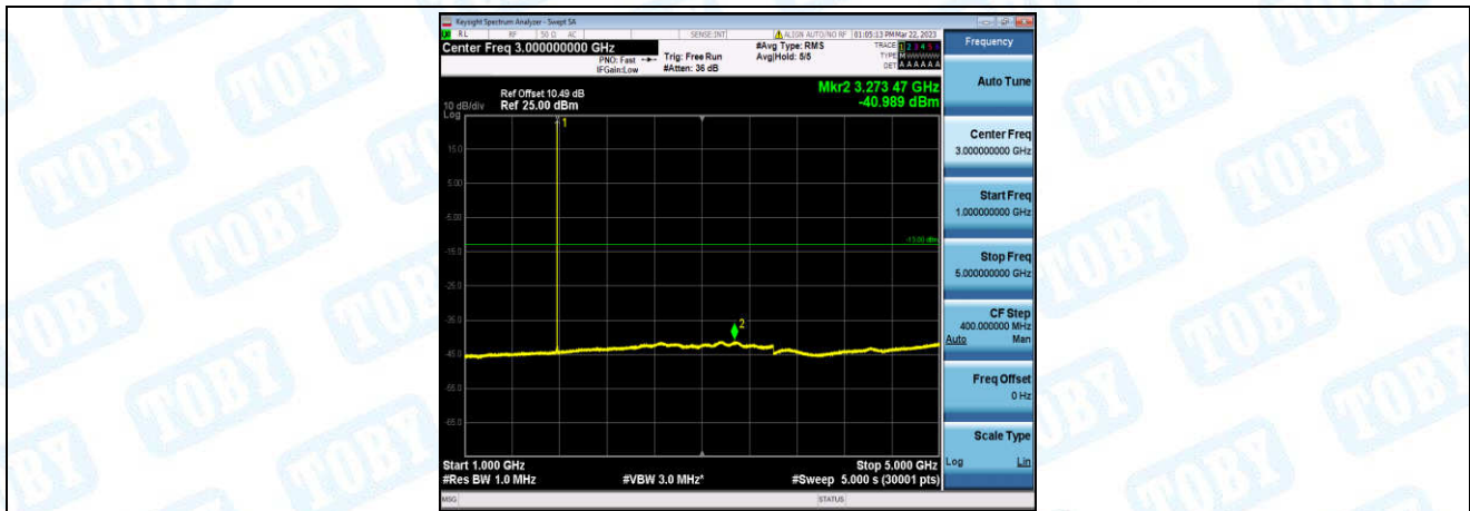
Band66-10MHz-16QAM-132622-1-0-High-1000-5000--40.99-PASS
