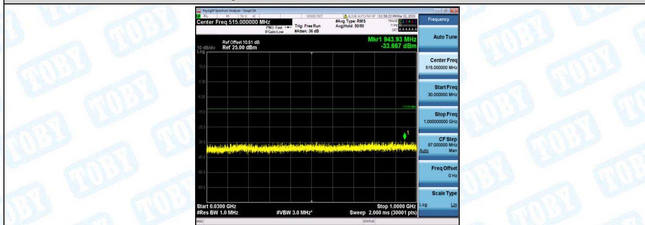
Band66-15MHz-QPSK-132322-1-0-Low-30-1000--33.67-PASS
