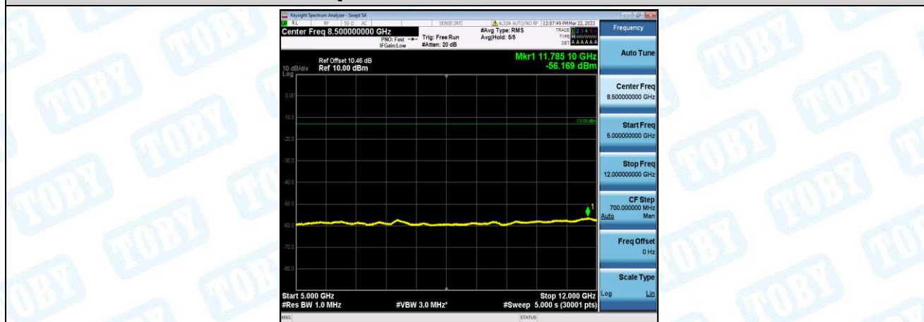
Band66-5MHz-QPSK-131997-1-0-Low-5000-12000--56.17-PASS
