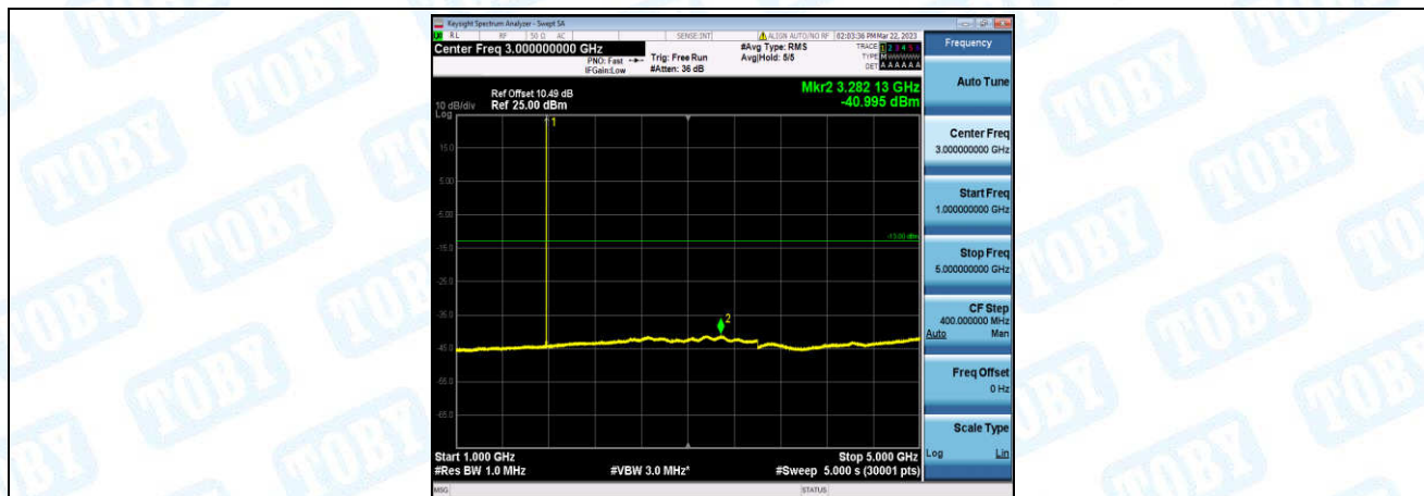
Band66-15MHz-QPSK-132597-1-0-High-1000-5000--41-PASS
