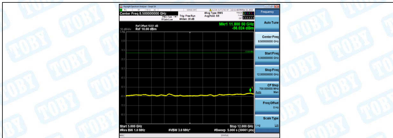
Band66-5MHz-QPSK-132322-1-0-Low-5000-12000--56.02-PASS
