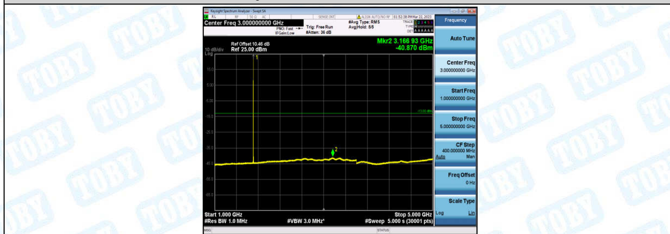
Band66-15MHz-QPSK-132047-1-0-Low-1000-5000--40.87-PASS
