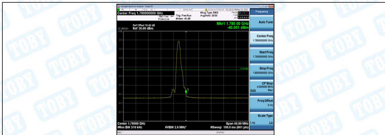
Band66-20MHz-QPSK-132572-1-0-High--40.05-PASS
