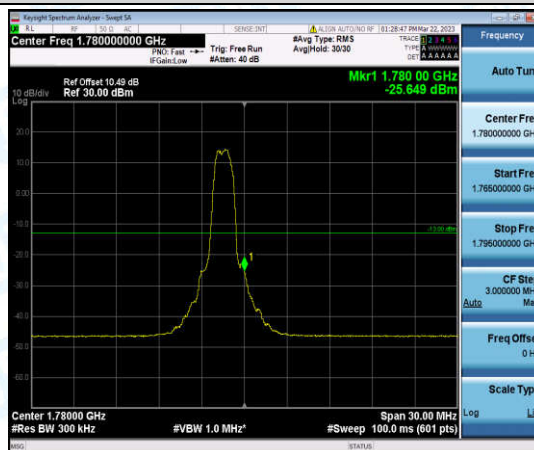
Band66-15MHz-QPSK-132597-6-0-High--25.65-PASS
