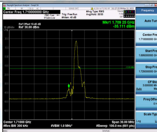
Band66-15MHz-16QAM-132047-1-0-Low--35.11-PASS
