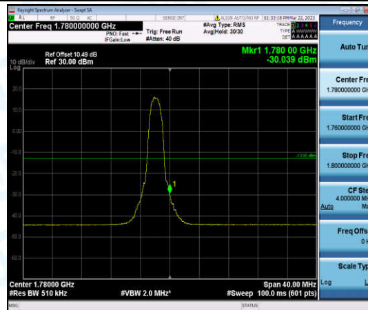
Band66-20MHz-16QAM-132572-6-0-High--30.04-PASS
