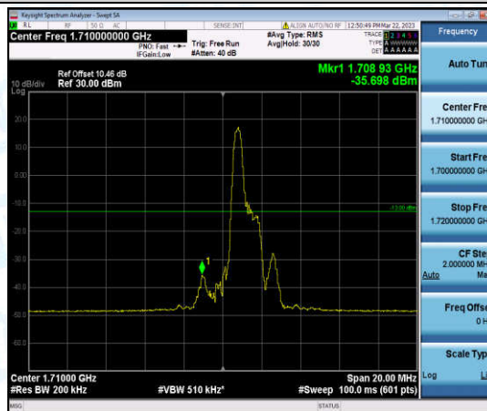
Band66-10MHz-16QAM-132022-1-0-Low--35.70-PASS
