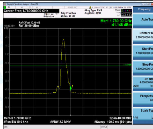
Band66-20MHz-16QAM-132572-1-0-High--41.15-PASS
