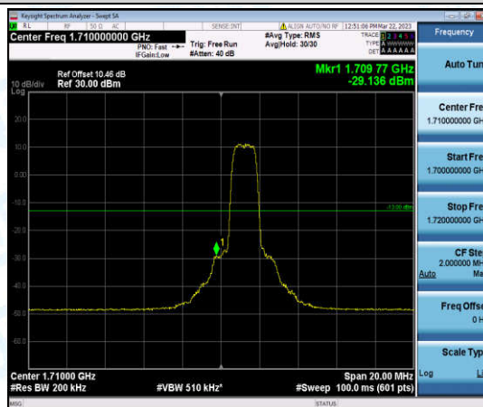
Band66-10MHz-16QAM-132022-6-0-Low--29.14-PASS
