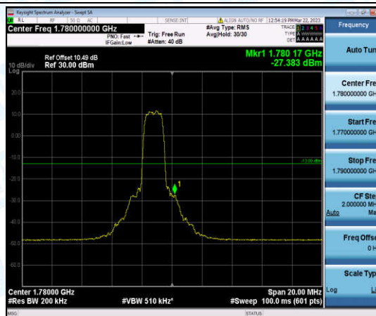
Band66-10MHz-QPSK-132622-6-0-High--27.38-PASS
