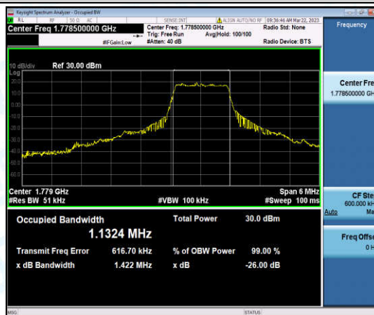
Band66-3MHz-QPSK-132657-6-0-High-1.1324-1.422-PASS
