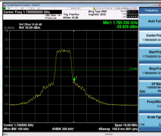
Band66-5MHz-QPSK-132647-6-0-High--25.93-PASS
