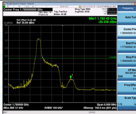
Band66-3MHz-16QAM-132657-1-0-High--39.36-PASS
