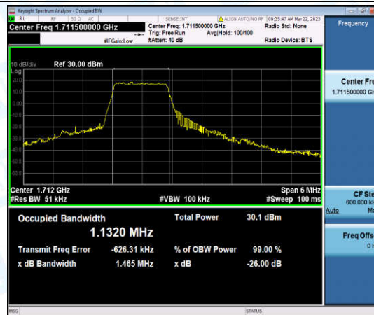
Band66-3MHz-16QAM-131987-6-0-Low-1.1320-1.465-PASS
