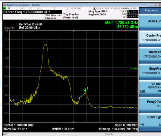
Band66-3MHz-QPSK-132657-1-0-High--37.73-PASS
