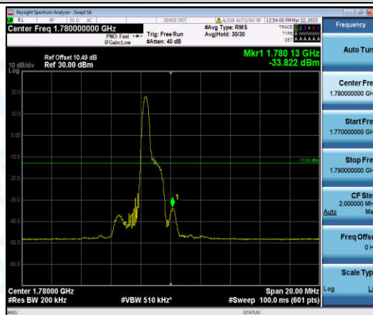
Band66-10MHz-QPSK-132622-1-0-High--33.82-PASS
