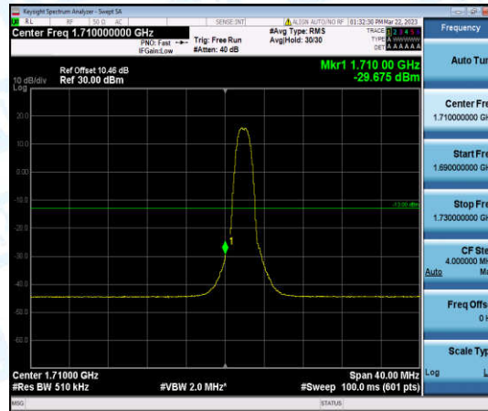
Band66-20MHz-16QAM-132072-6-0-Low--29.68-PASS
