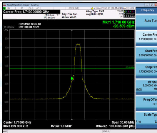
Band66-15MHz-16QAM-132047-6-0-Low--26.51-PASS
