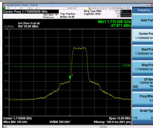
Band66-5MHz-QPSK-131997-6-0-Low--27.97-PASS
