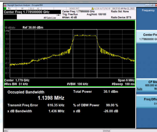
Band66-3MHz-16QAM-132657-6-0-High-1.1398-1.436-PASS
