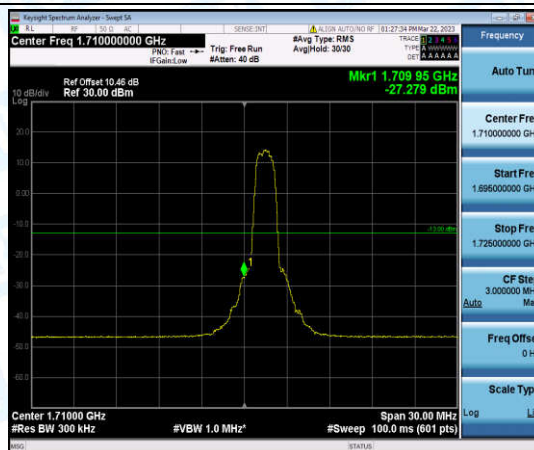
Band66-15MHz-QPSK-132047-6-0-Low--27.28-PASS
