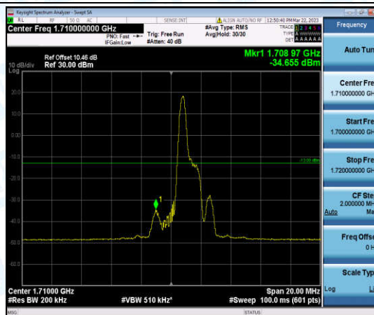
Band66-10MHz-QPSK-132022-1-0-Low--34.66-PASS
