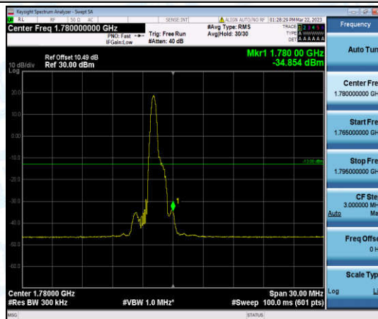
Band66-15MHz-QPSK-132597-1-0-High--34.85-PASS
