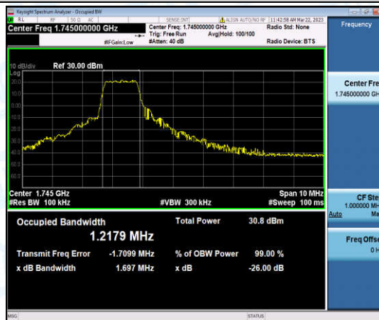
Band66-5MHz-16QAM-132322-6-0-Low-1.2179-1.697-PASS
