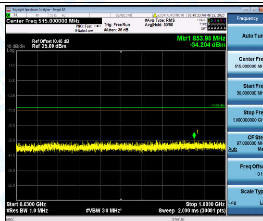
Band66-1.4MHz-QPSK-131979-1-0-Low-30-1000--34.2-PASS
