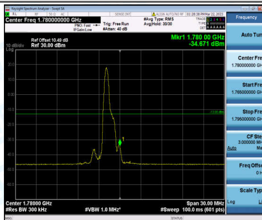
Band66-15MHz-16QAM-132597-1-0-High--34.67-PASS
