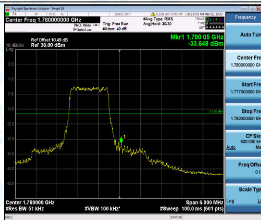
Band66-3MHz-16QAM-132657-6-0-High--33.65-PASS
