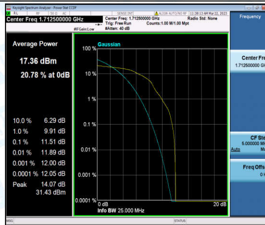
Band66-5MHz-16QAM-131997-1-0-Low-11.51-<=13-PASS
