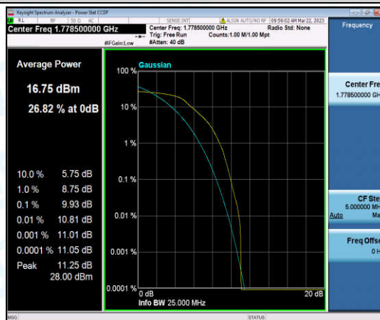
Band66-3MHz-16QAM-132657-6-0-High-9.93-<=13-PASS
