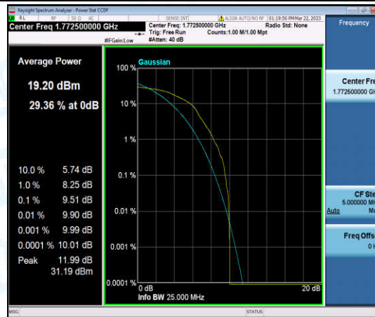
Band66-15MHz-16QAM-132597-1-0-High-9.51-=<=13-PASS
