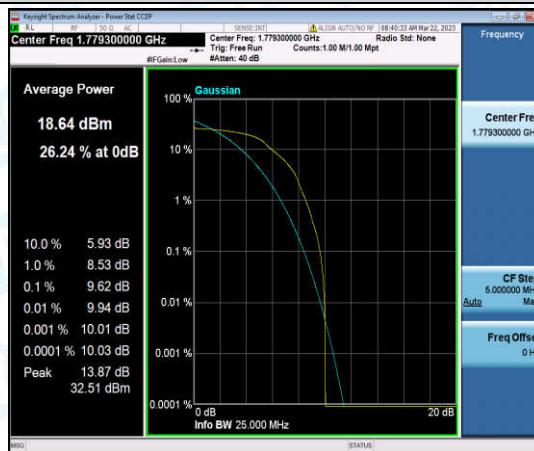
Band66-1.4MHz-QPSK-132665-1-0-High-9.62-<=13-PASS
