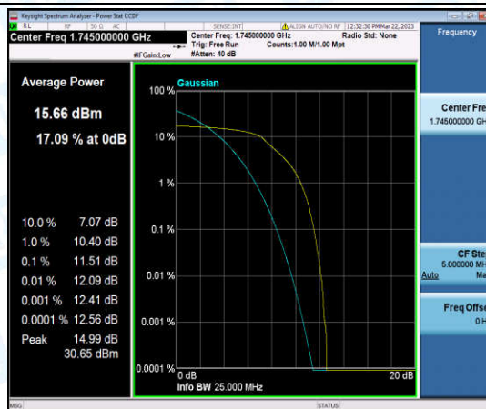
Band66-10MHz-QPSK-132322-6-0-Low-11.51-<=13-PASS
