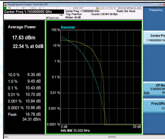
Band66-3MHz-16QAM-132322-1-0-Low-10.43-<=13-PASS
