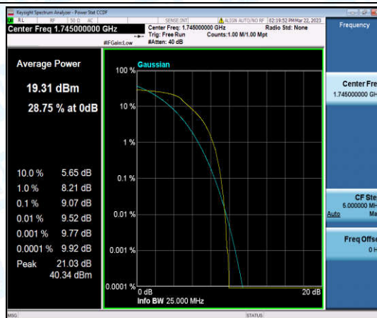
Band66-20MHz-16QAM-132322-6-0-Low-9.07-≤13-PASS
