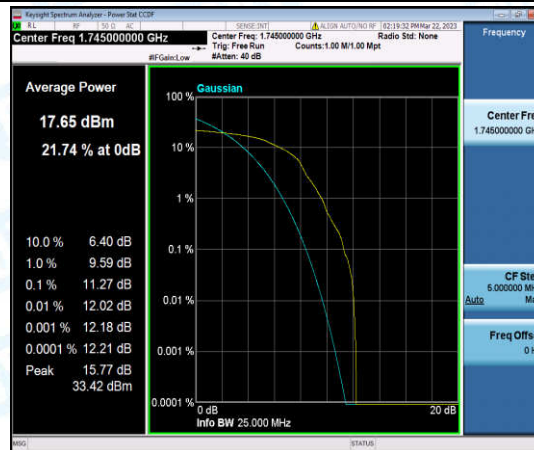
Band66-20MHz-16QAM-132322-1-0-Low-11.27-13-PASS
