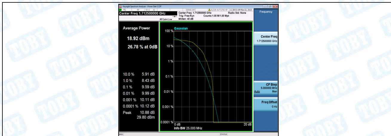
Band66-5MHz-QPSK-131997-1-0-Low-9.59-<=13-PASS
