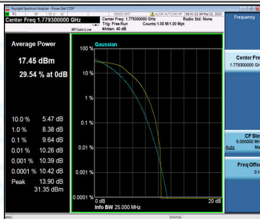
Band66-1.4MHz-16QAM-132665-6-0-High-9.64-<=13-PASS
