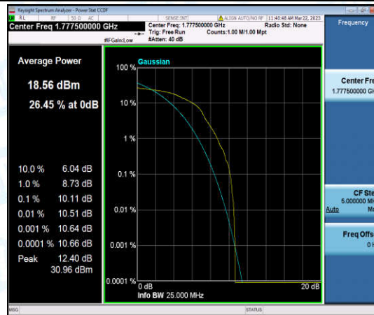
Band66-5MHz-16QAM-132647-1-0-High-10.11-<=13-PASS
