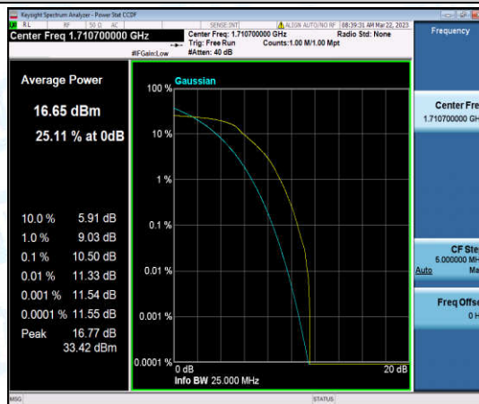
Band66-1.4MHz-16QAM-131979-6-0-Low-10.50-<=13-PASS
