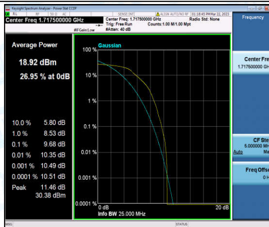
Band66-15MHz-16QAM-132047-6-0-Low-9.68-<=13-PASS
