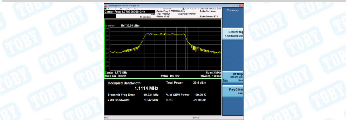
Band66-1.4MHz-QPSK-132665-6-0-High-1.1114-1.342-PASS
