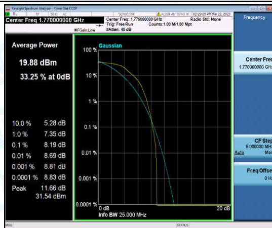
Band66-20MHz-QPSK-132572-1-0-High-8.19-<=13-PASS
