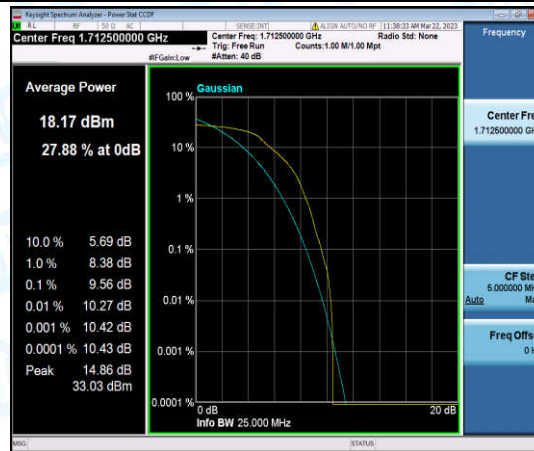
Band66-5MHz-16QAM-131997-6-0-Low-9.56-<=13-PASS
