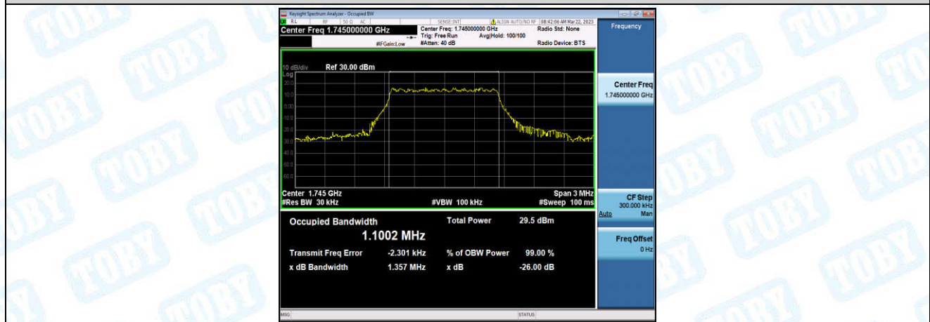
Band66-1.4MHz-QPSK-132322-6-0-Low-1.1002-1.357-PASS
