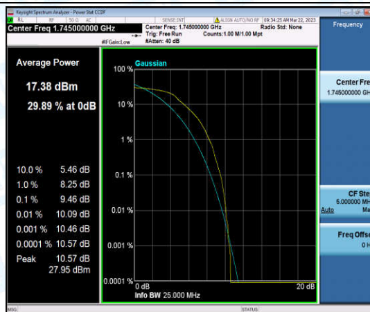
Band66-3MHz-16QAM-132322-6-0-Low-9.46-<=13-PASS
