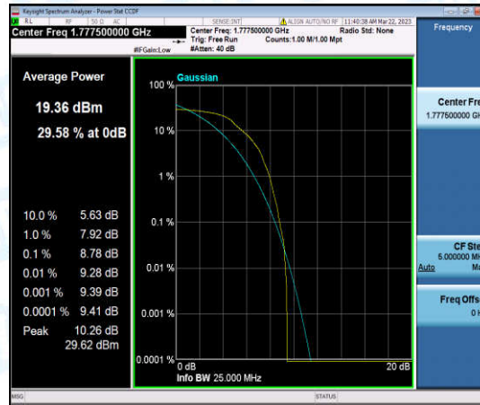
Band66-5MHz-QPSK-132647-1-0-High-8.78-<=13-PASS
