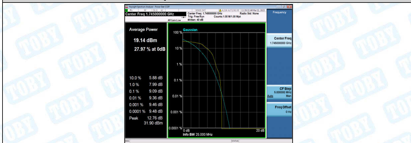
Band66-5MHz-QPSK-132322-1-0-Low-9.09-<=13-PASS
