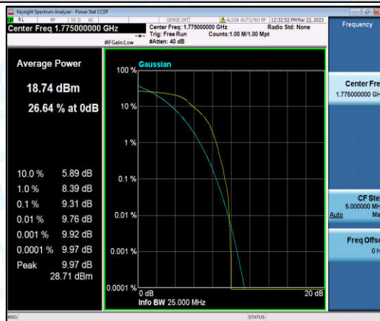
Band66-10MHz-QPSK-132622-1-0-High-9.31-<=13-PASS
