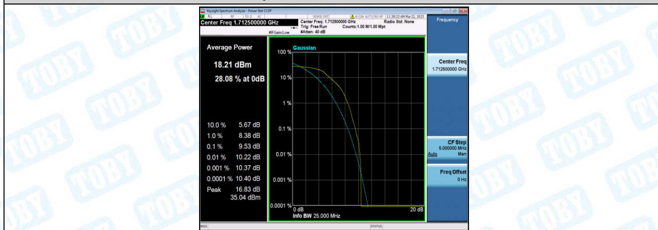
Band66-5MHz-QPSK-131997-6-0-Low-9.53-<=13-PASS
