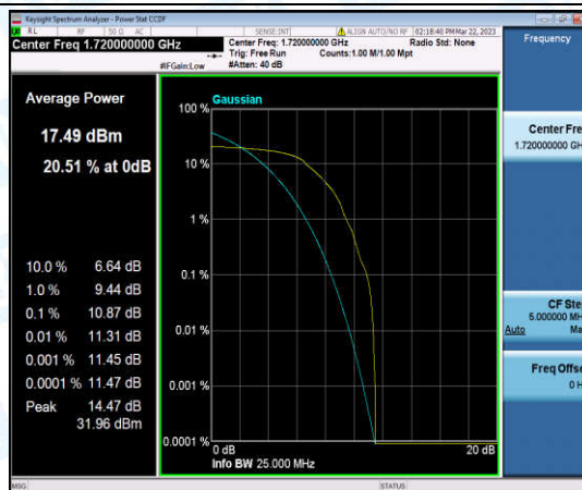
Band66-20MHz-QPSK-132072-1-0-Low-10.87-<=13-PASS
