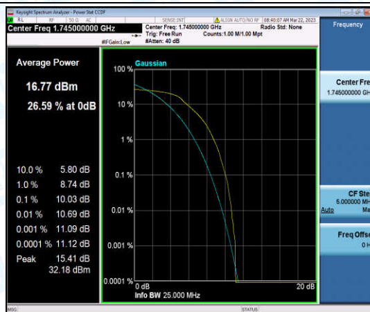
Band66-1.4MHz-QPSK-132322-6-0-Low-10.03-<=13-PASS
