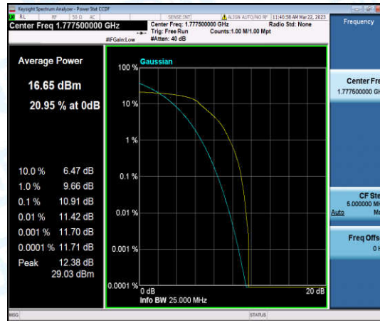
Band66-5MHz-QPSK-132647-6-0-High-10.91-<=13-PASS
