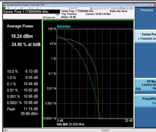
Band66-20MHz-16QAM-132572-1-0-High-10.46-≤13-PASS
