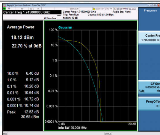
Band66-15MHz-QPSK-132322-1-0-Low-10.28-<=13-PASS
