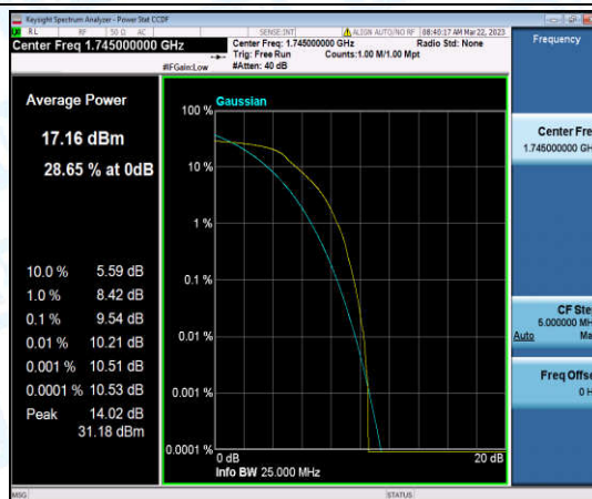
Band66-1.4MHz-16QAM-132322-6-0-Low-9.54-<=13-PASS
