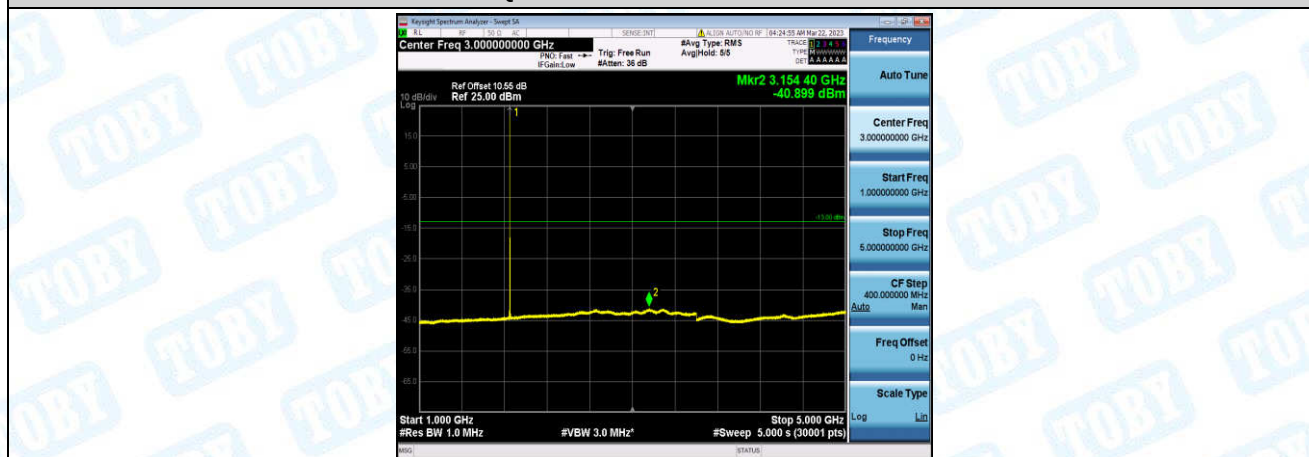
Band25-10MHz-QPSK-26090-1-0-Low-1000-5000--40.9-PASS
