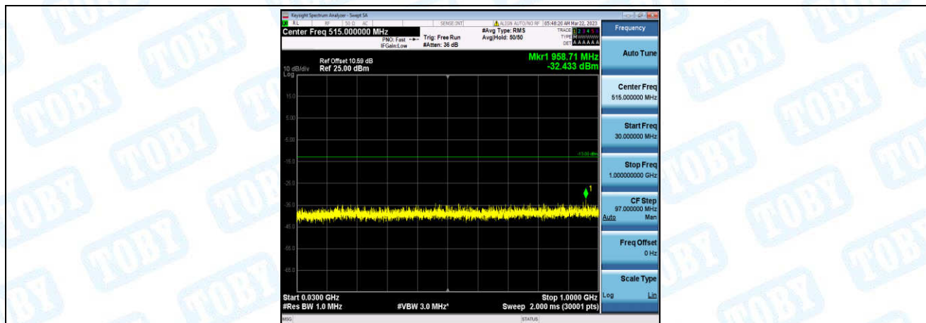
Band25-3MHz-16QAM-26365-1-0-Low-30-1000--32.43-PASS
