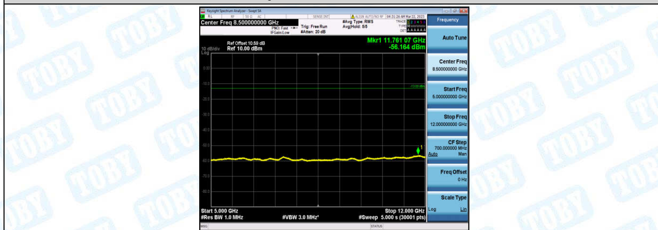
Band25-10MHz-16QAM-26365-1-0-Low-5000-12000--56.16-PASS
