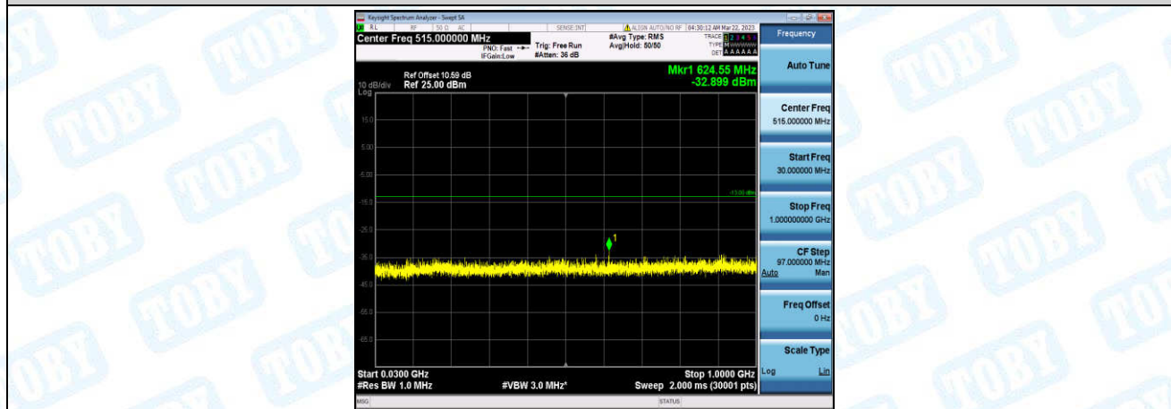
Band25-10MHz-16QAM-26365-1-0-Low-30-1000--32.9-PASS
