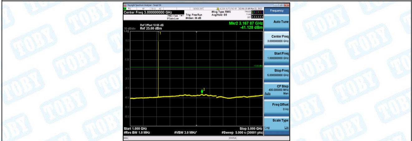
Band25-3MHz-QPSK-26055-1-0-Low-1000-5000--41.13-PASS
