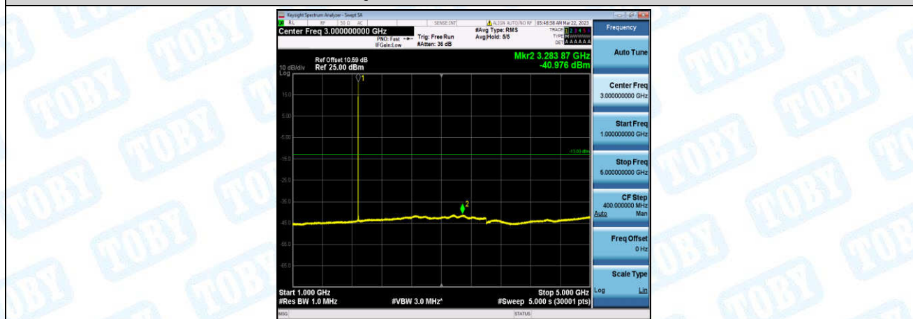
Band25-3MHz-16QAM-26365-1-0-Low-1000-5000--40.98-PASS
