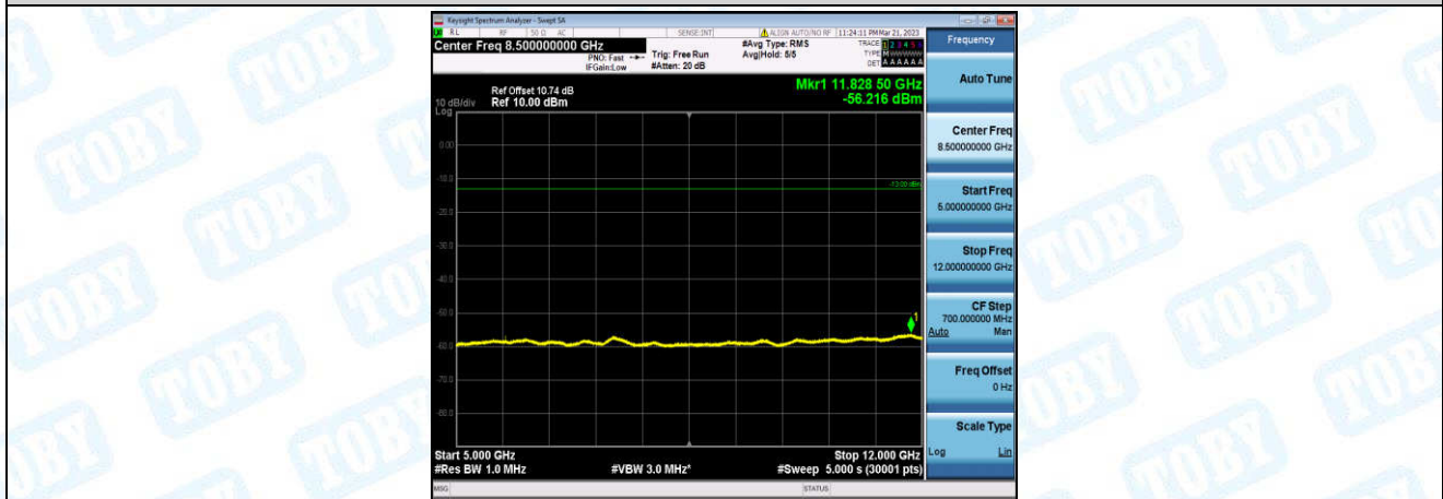
Band25-1.4MHz-QPSK-26683-1-0-High-5000-12000--56.22-PASS
