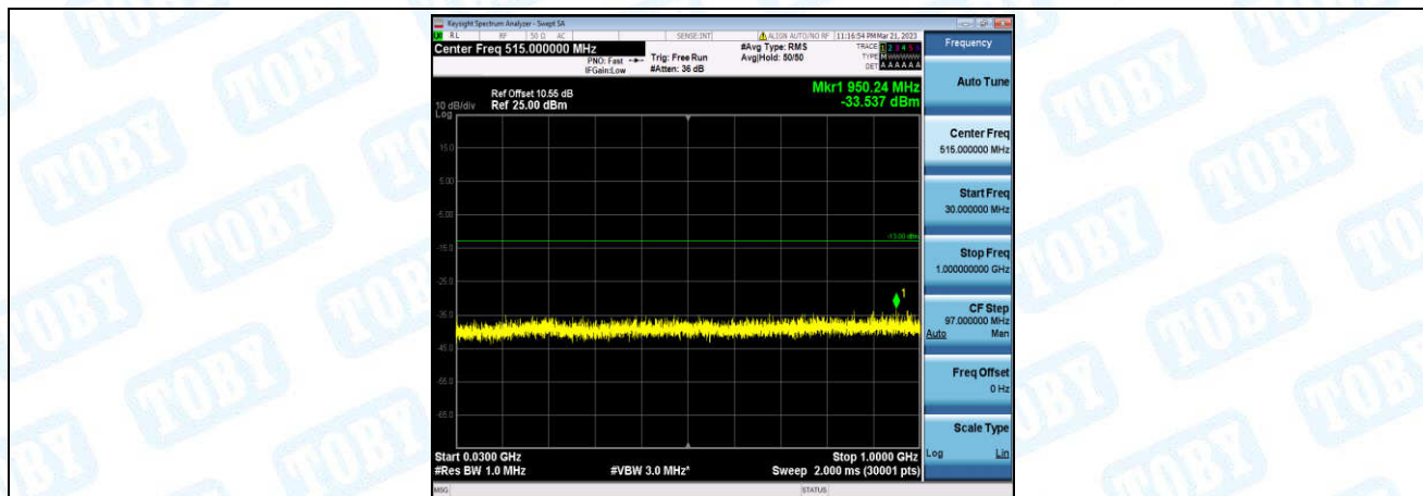
Band25-1.4MHz-16QAM-26047-1-0-Low-30-1000--33.54-PASS
