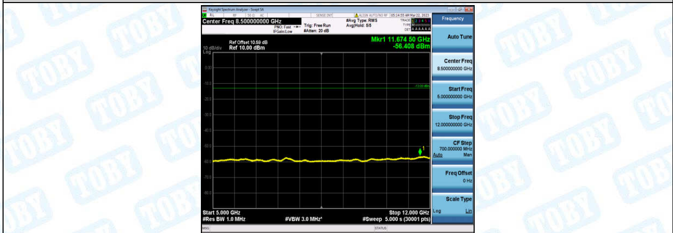
Band25-15MHz-QPSK-26365-1-0-Low-5000-12000--56.41-PASS
