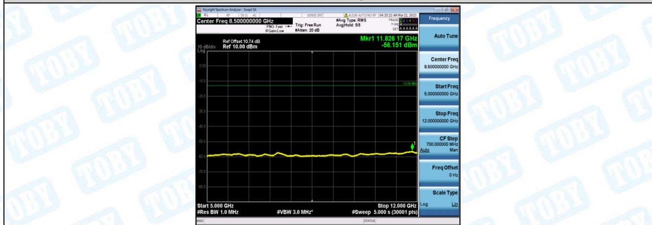
Band25-10MHz-16QAM-26640-1-0-High-5000-12000--56.15-PASS
