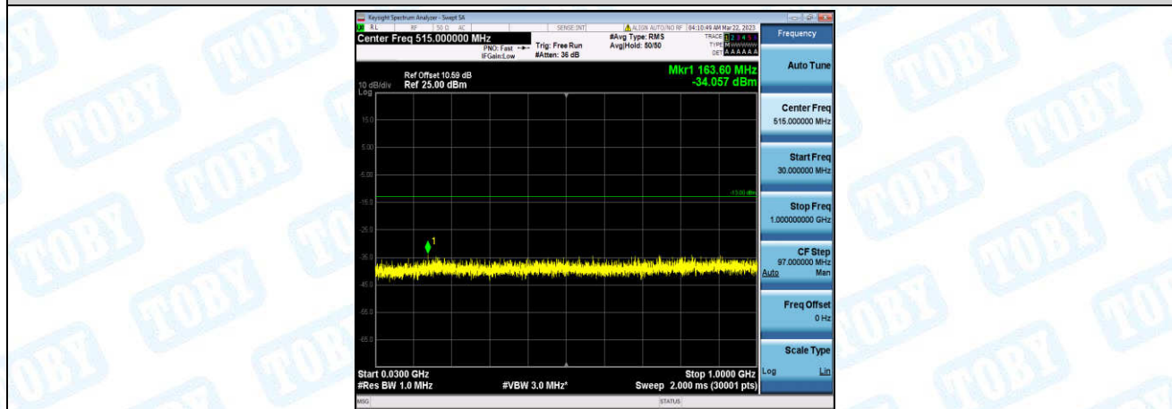
Band25-5MHz-16QAM-26365-1-0-Low-30-1000--34.06-PASS
