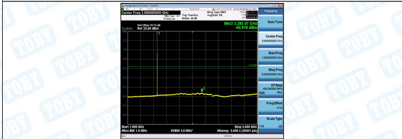
Band25-10MHz-16QAM-26640-1-0-High-1000-5000--40.92-PASS
