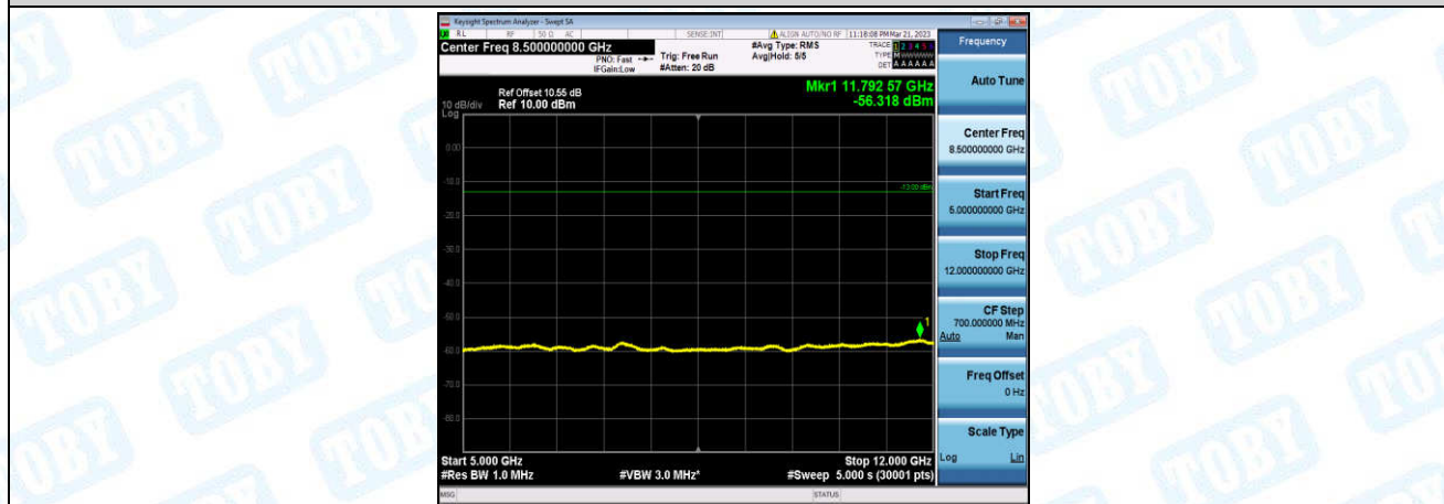
Band25-1.4MHz-16QAM-26047-1-0-Low-5000-12000--56.32-PASS
