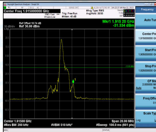
Band25-10MHz-QPSK-26640-1-0-High--31.33-PASS
