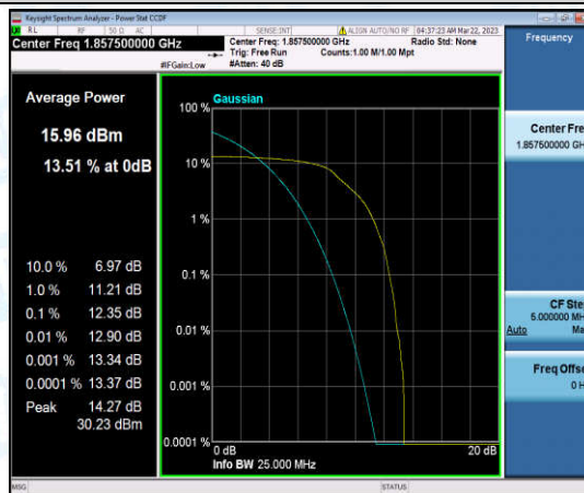
Band25-15MHz-16QAM-26115-6-0-Low-12.35-<=13-PASS
