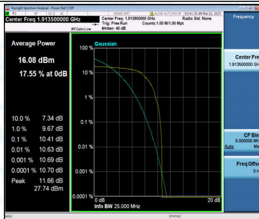
Band25-3MHz-QPSK-26675-1-0-High-10.41-<=13-PASS
