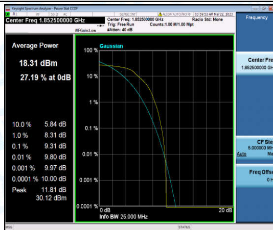
Band25-5MHz-16QAM-26065-6-0-Low-9.31-<=13-PASS
