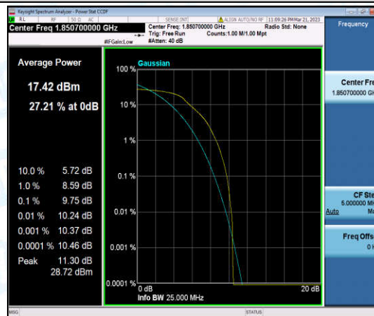
Band25-1.4MHz-16QAM-26047-6-0-Low-9.75-<=13-PASS
