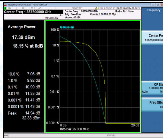
Band25-15MHz-QPSK-26115-1-0-Low-10.99-<=13-PASS
