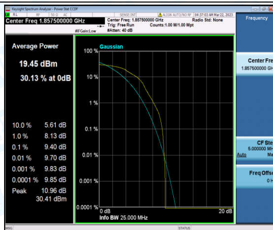
Band25-15MHz-16QAM-26115-1-0-Low-9.40-<=13-PASS
