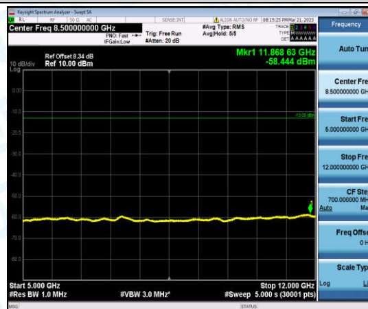
Band12-1.4MHz-QPSK-23017-1-0-Low-5000-12000--58.44-PASS
