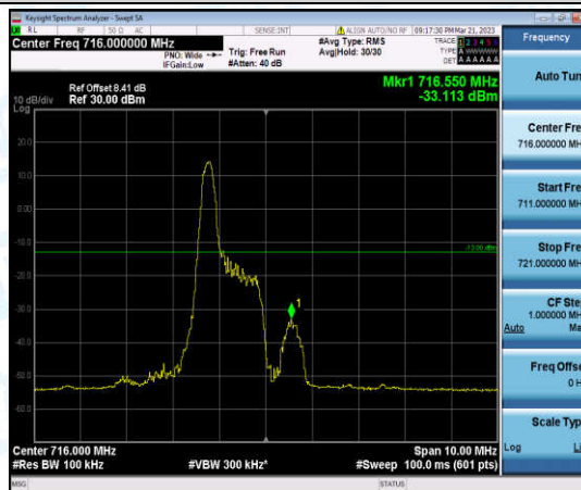
Band12-5MHz-16QAM-23155-1-0-High--33.11-PASS
