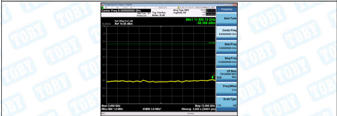
Band12-5MHz-QPSK-23155-1-0-High-5000-12000--58.39-PASS
