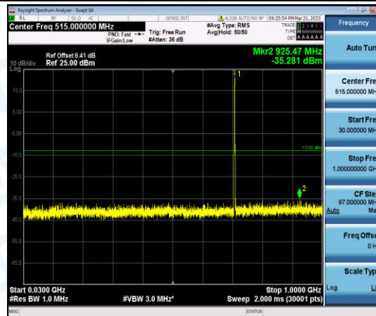
Band12-5MHz-QPSK-23155-1-0-High-30-1000--35.28-PASS
