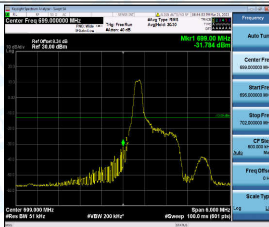
Band12-3MHz-16QAM-23025-1-0-Low--31.78-PASS
