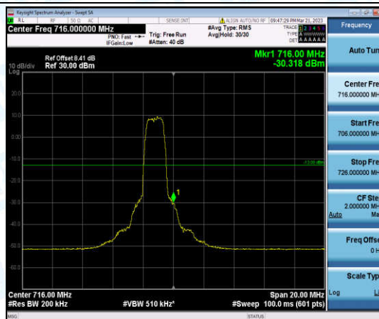
Band12-10MHz-QPSK-23130-6-0-High--30.32-PASS
