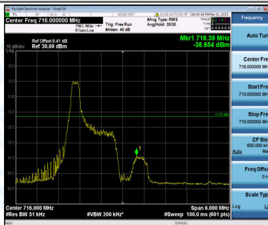
Band12-3MHz-16QAM-23165-1-0-High--38.65-PASS
