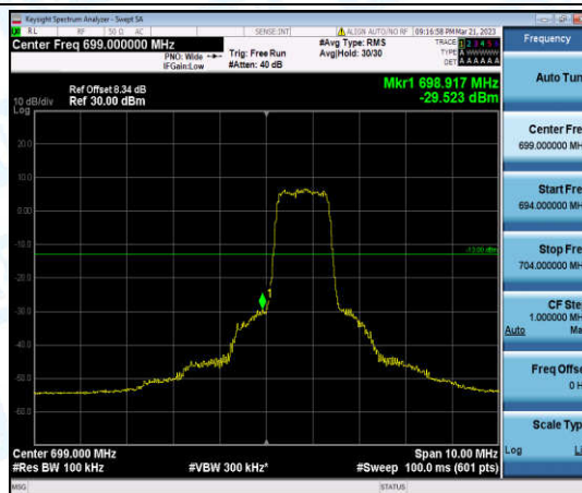
Band12-5MHz-16QAM-23035-6-0-Low--29.52-PASS
