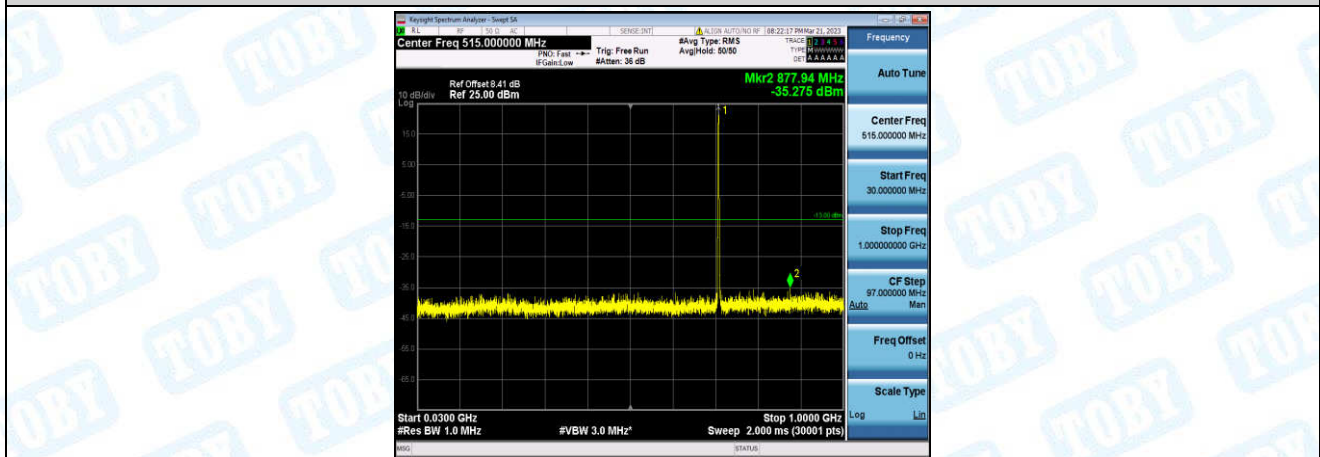
Band12-1.4MHz-QPSK-23173-1-0-High-30-1000--35.28-PASS
