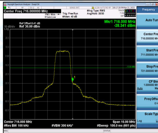
Band12-5MHz-QPSK-23155-6-0-High--28.34-PASS
