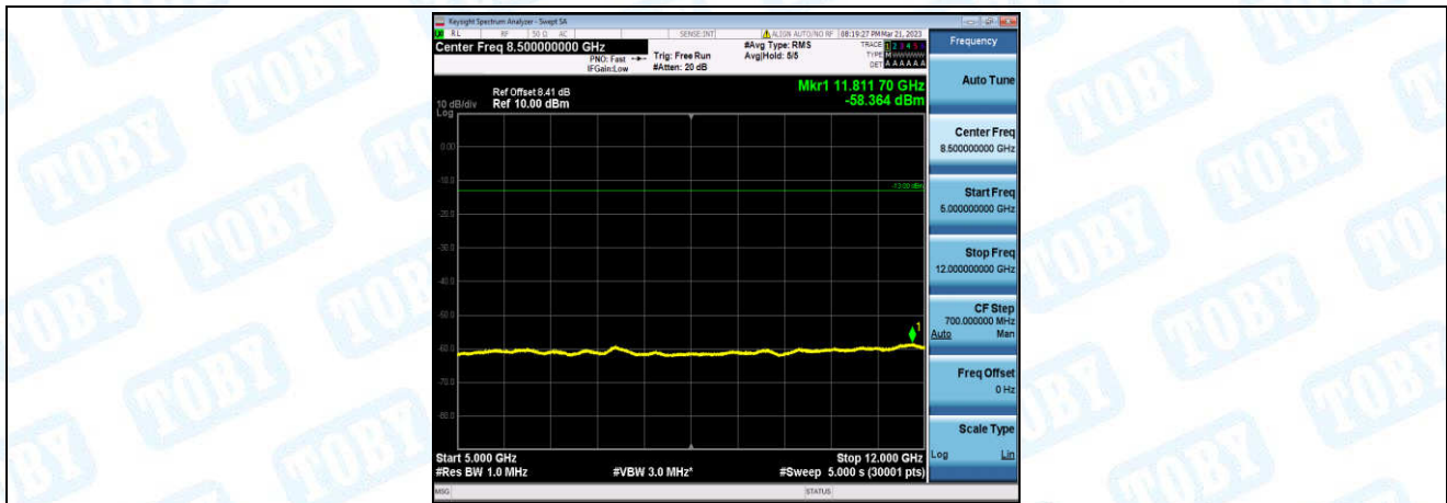
Band12-1.4MHz-QPSK-23095-1-0-Low-5000-12000--58.36-PASS
