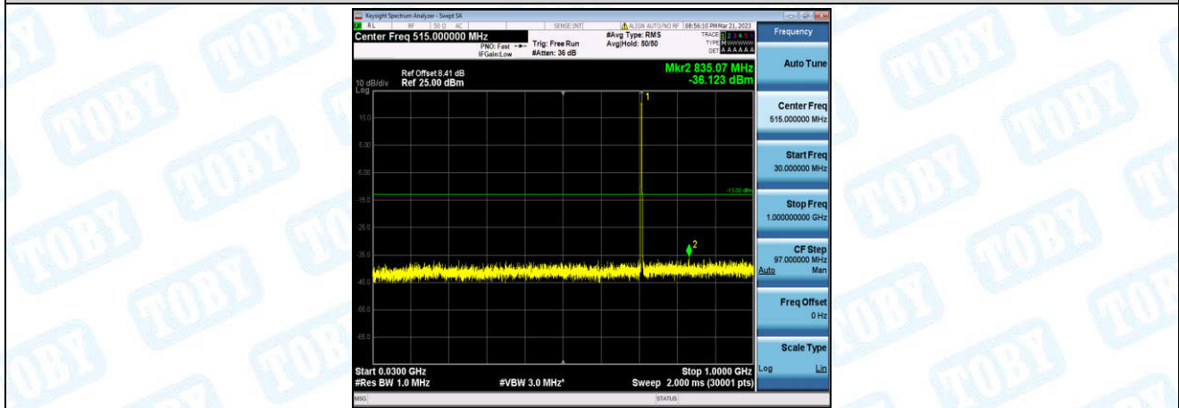
Band12-3MHz-16QAM-23165-1-0-High-30-1000--36.12-PASS
