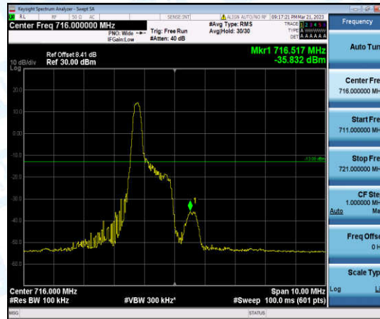
Band12-5MHz-QPSK-23155-1-0-High--35.83-PASS
