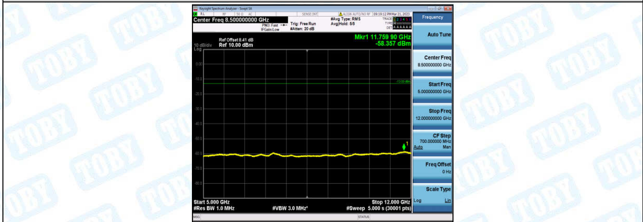
Band12-5MHz-QPSK-23035-1-0-Low-5000-12000--58.36-PASS
