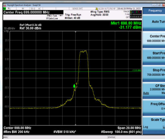
Band12-10MHz-QPSK-23060-6-0-Low--31.18-PASS
