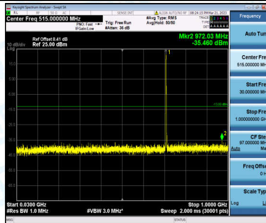
Band12-1.4MHz-16QAM-23173-1-0-High-30-1000--35.46-PASS
