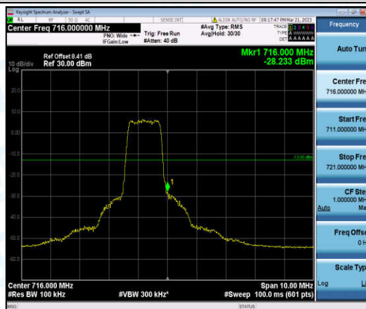
Band12-5MHz-16QAM-23155-6-0-High--28.23-PASS
