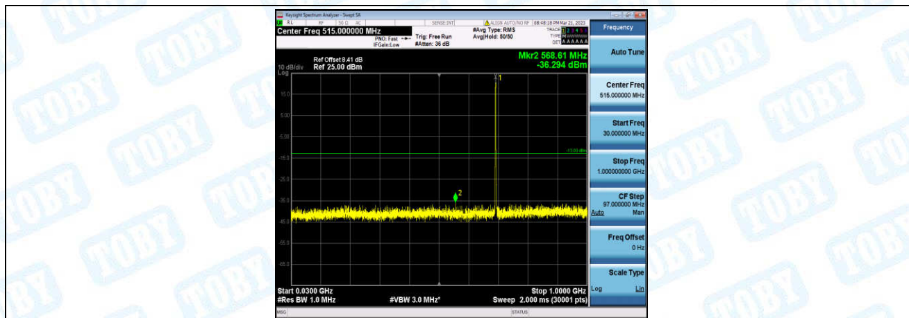
Band12-3MHz-16QAM-23025-1-0-Low-30-1000--36.29-PASS
