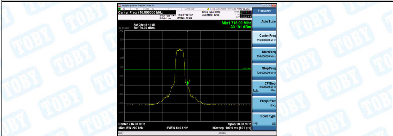
Band12-10MHz-16QAM-23130-6-0-High--30.19-PASS
