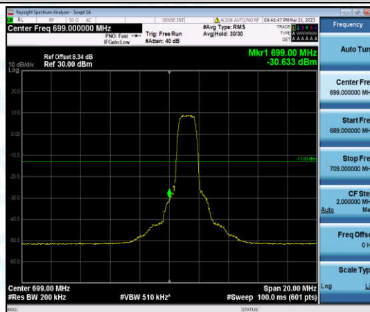
Band12-10MHz-16QAM-23060-6-0-Low--30.63-PASS
