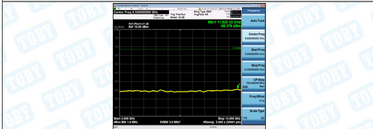
Band12-3MHz-QPSK-23025-1-0-Low-5000-12000--58.38-PASS
