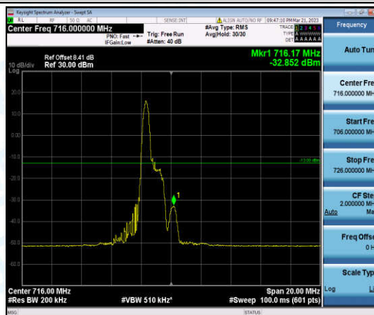
Band12-10MHz-QPSK-23130-1-0-High--32.85-PASS
