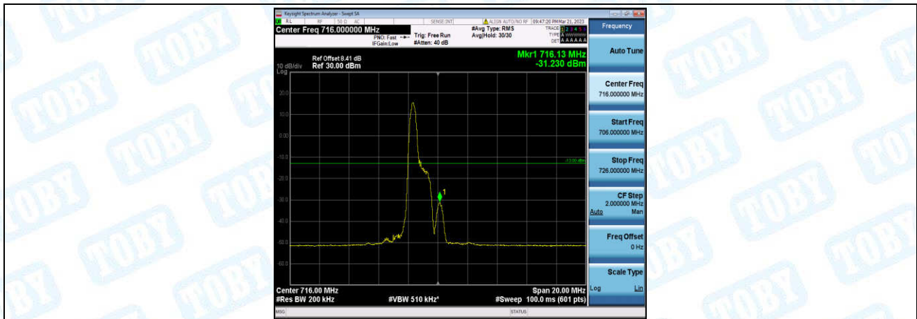
Band12-10MHz-16QAM-23130-1-0-High--31.23-PASS
