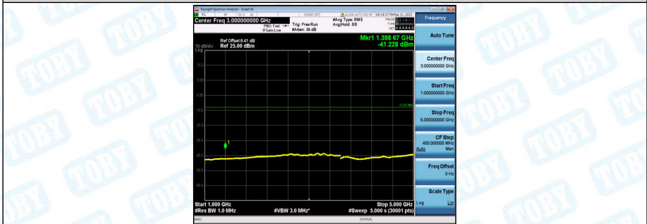
Band12-5MHz-QPSK-23035-1-0-Low-1000-5000--41.23-PASS
