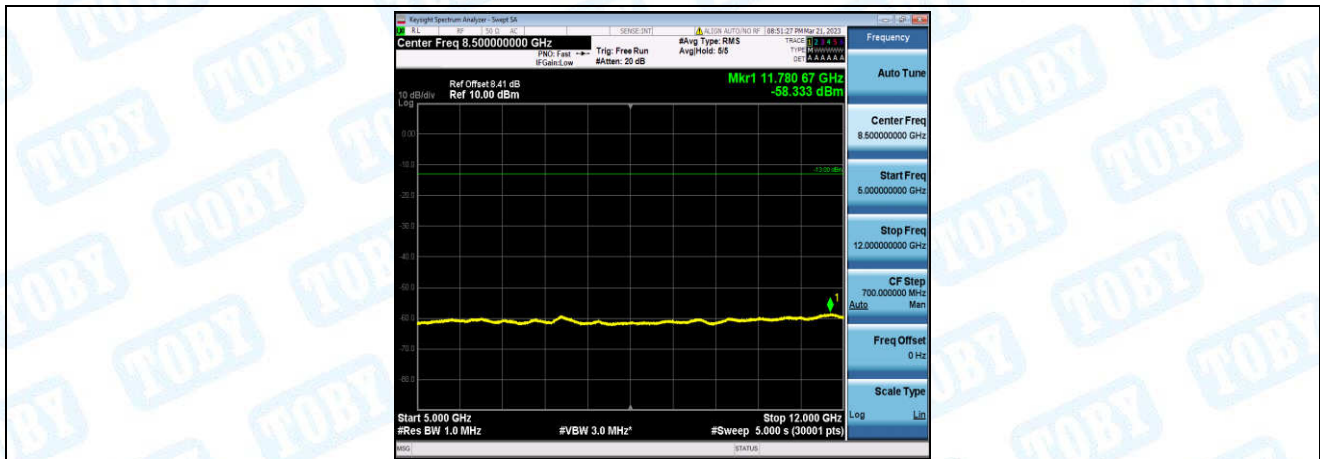
Band12-3MHz-QPSK-23095-1-0-Low-5000-12000--58.33-PASS
