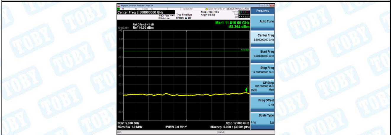
Band12-1.4MHz-16QAM-23173-1-0-High-5000-12000--58.36-PASS
