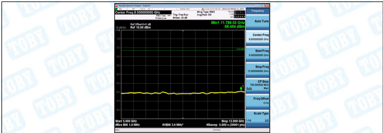
Band12-3MHz-16QAM-23095-1-0-Low-5000-12000--58.45-PASS
