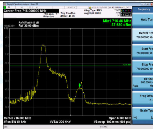
Band12-3MHz-QPSK-23165-1-0-High--37.68-PASS
