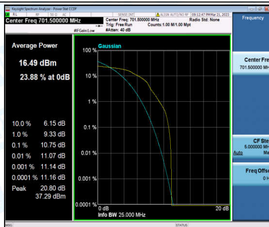
Band12-5MHz-16QAM-23035-1-0-Low-10.75-<=13-PASS
