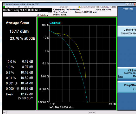
Band12-5MHz-16QAM-23035-6-0-Low-10.18-<=13-PASS
