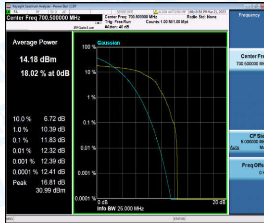
Band12-3MHz-16QAM-23025-1-0-Low-11.83-<=13-PASS
