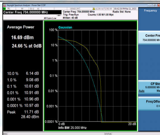
Band12-10MHz-16QAM-23060-1-0-Low-10.61-<=13-PASS
