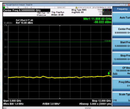
Band5-5MHz-16QAM-20425-1-0-Low-5000-12000--58.02-PASS
