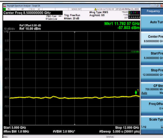
Band5-5MHz-QPSK-20625-1-0-High-5000-12000--57.8-PASS
