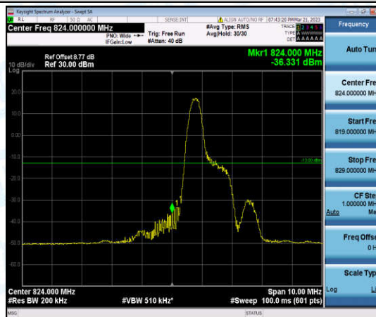
Band5-10MHz-16QAM-20450-1-0-Low--36.33-PASS
