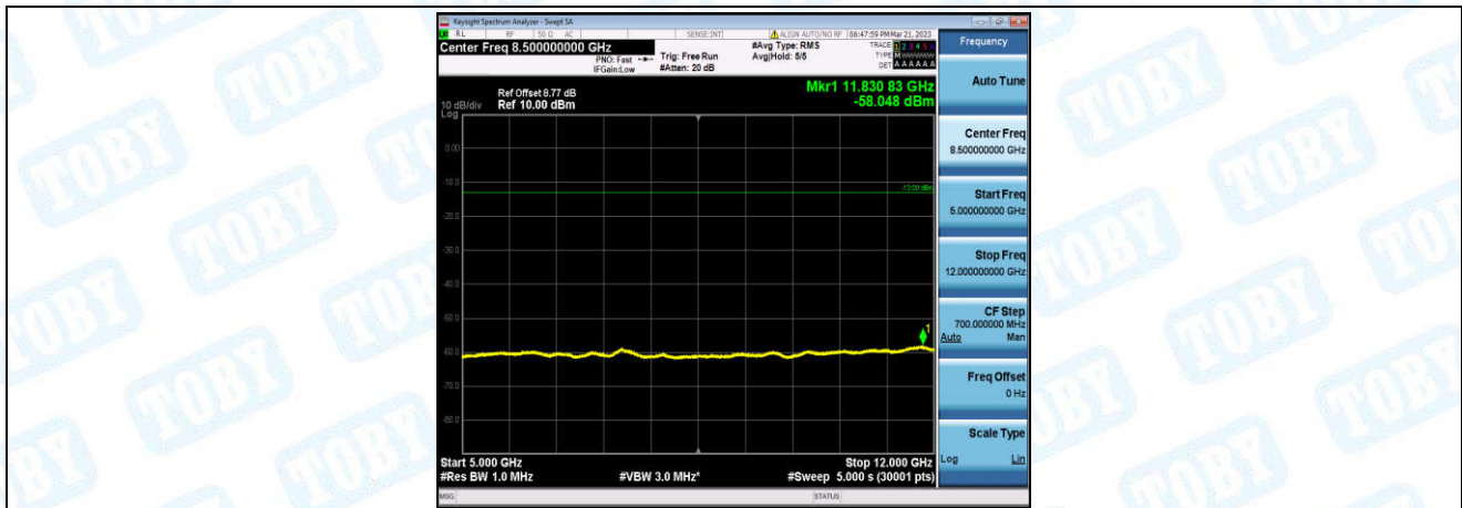
Band5-3MHz-QPSK-20525-1-0-Low-5000-12000--58.05-PASS
