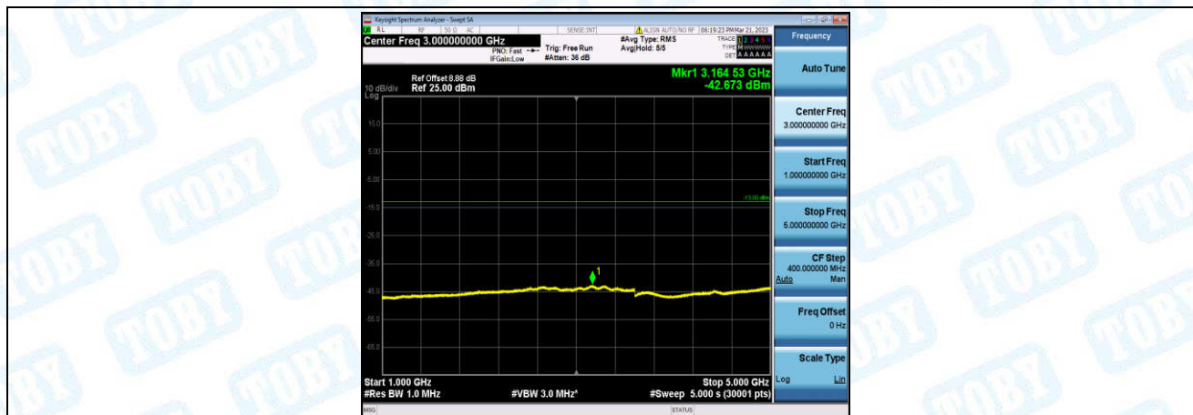
Band5-1.4MHz-QPSK-20643-1-0-High-1000-5000--42.67-PASS
