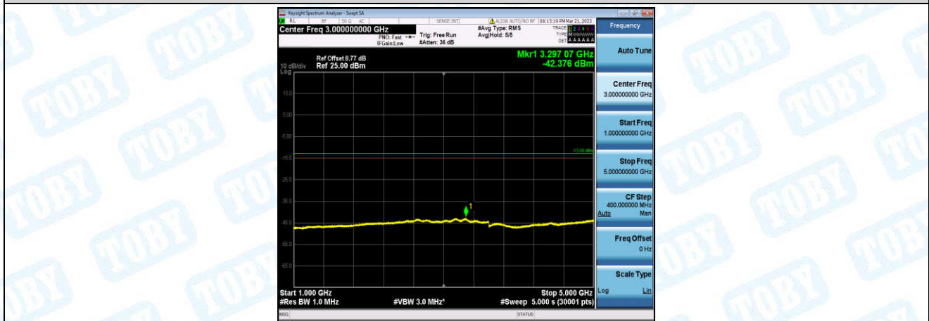
Band5-1.4MHz-16QAM-20407-1-0-Low-1000-5000--42.38-PASS
