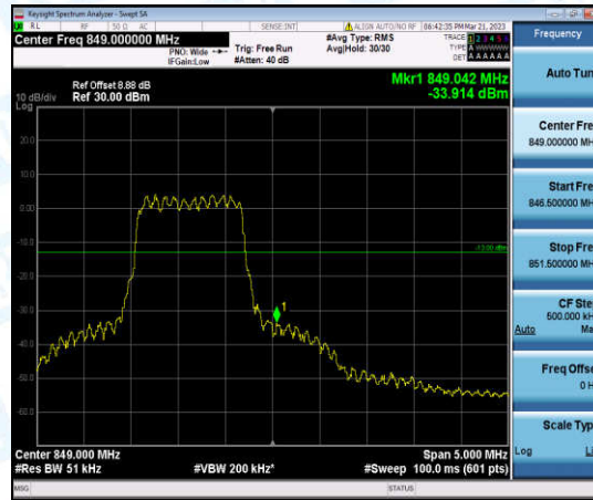
Band5-3MHz-16QAM-20635-6-0-High--33.91-PASS
