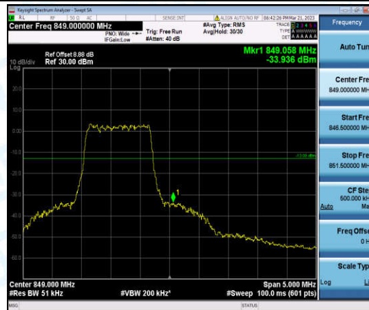
Band5-3MHz-QPSK-20635-6-0-High--33.94-PASS
