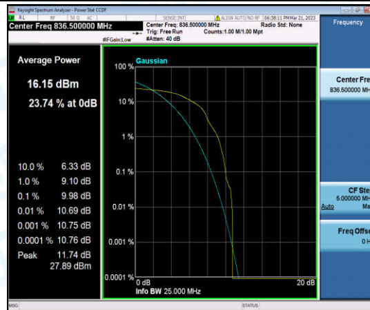
Band5-3MHz-16QAM-20525-1-0-Low-9.98-<=13-PASS
