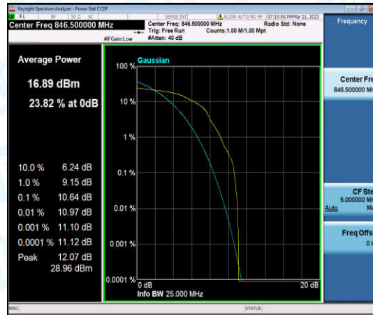
Band5-5MHz-16QAM-20625-1-0-High-10.64-<=13-PASS
