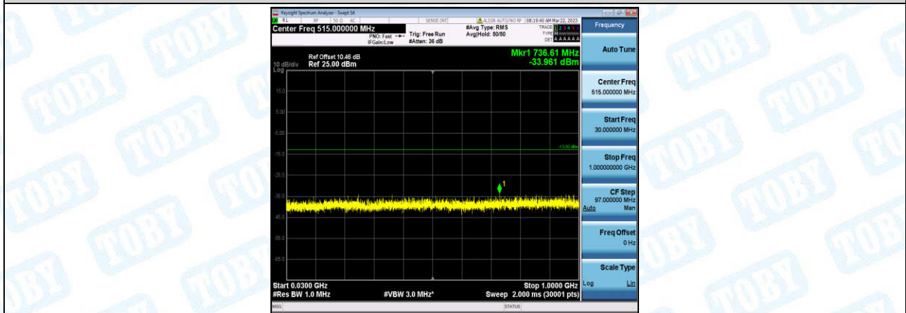
Band4-20MHz-QPSK-20175-1-0-Low-30-1000--33.96-PASS
