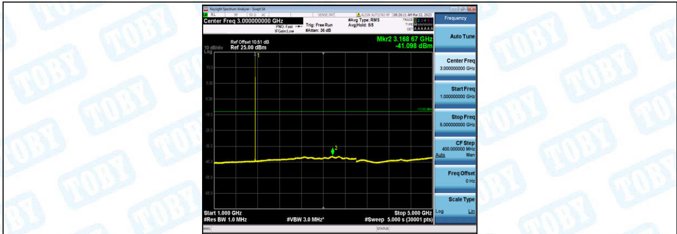
Band4-20MHz-16QAM-20300-1-0-High-1000-5000--41.1-PASS
