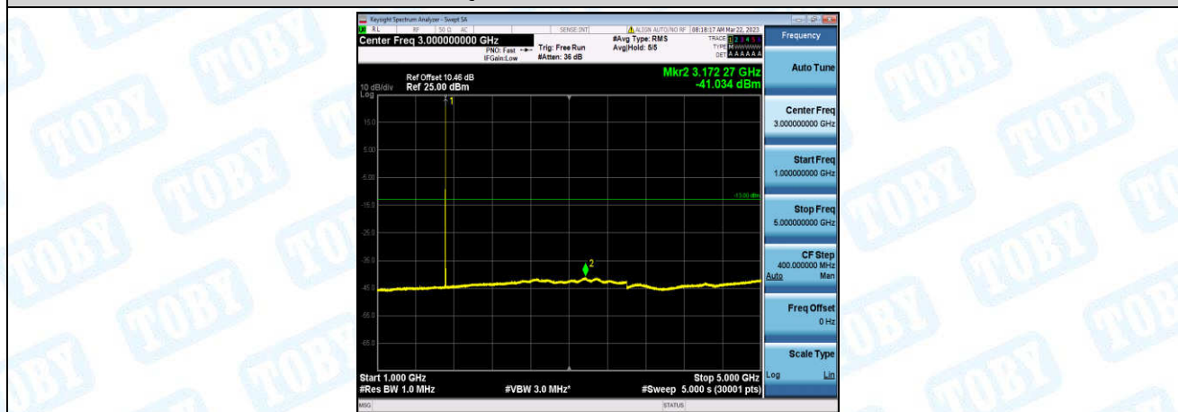
Band4-20MHz-16QAM-20050-1-0-Low-1000-5000--41.03-PASS
