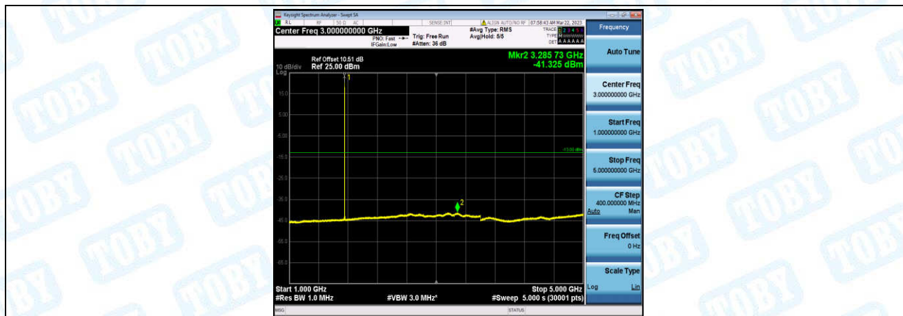
Band4-15MHz-16QAM-20325-1-0-High-1000-5000--41.33-PASS
