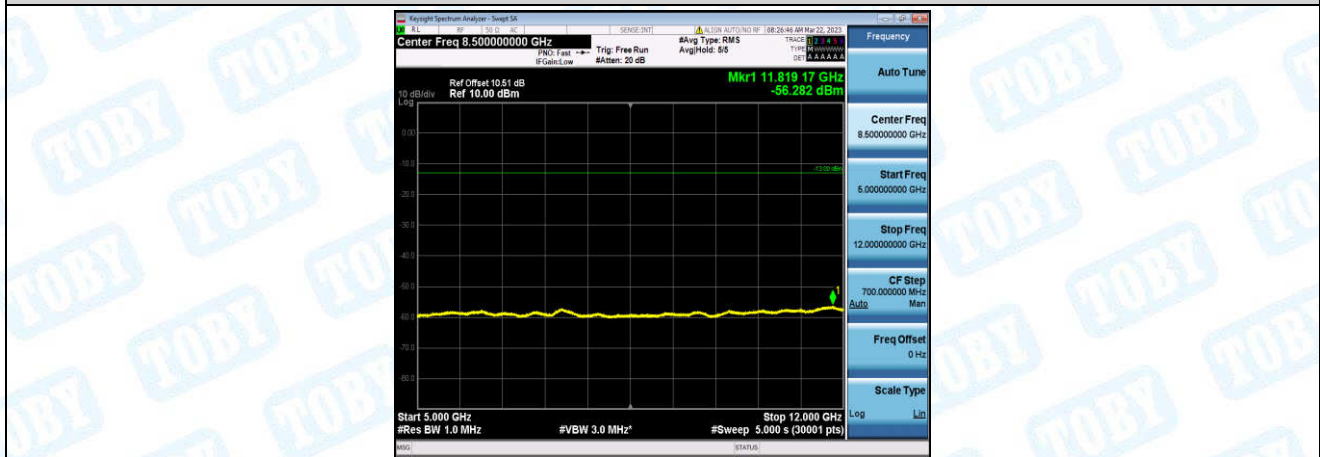
Band4-20MHz-16QAM-20300-1-0-High-5000-12000--56.28-PASS
