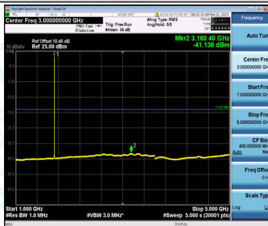
Band4-20MHz-16QAM-20175-1-0-Low-1000-5000--41.14-PASS
