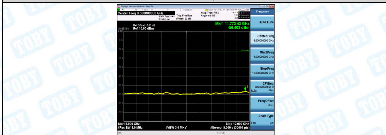
Band4-15MHz-16QAM-20325-1-0-High-5000-12000--56.4-PASS
