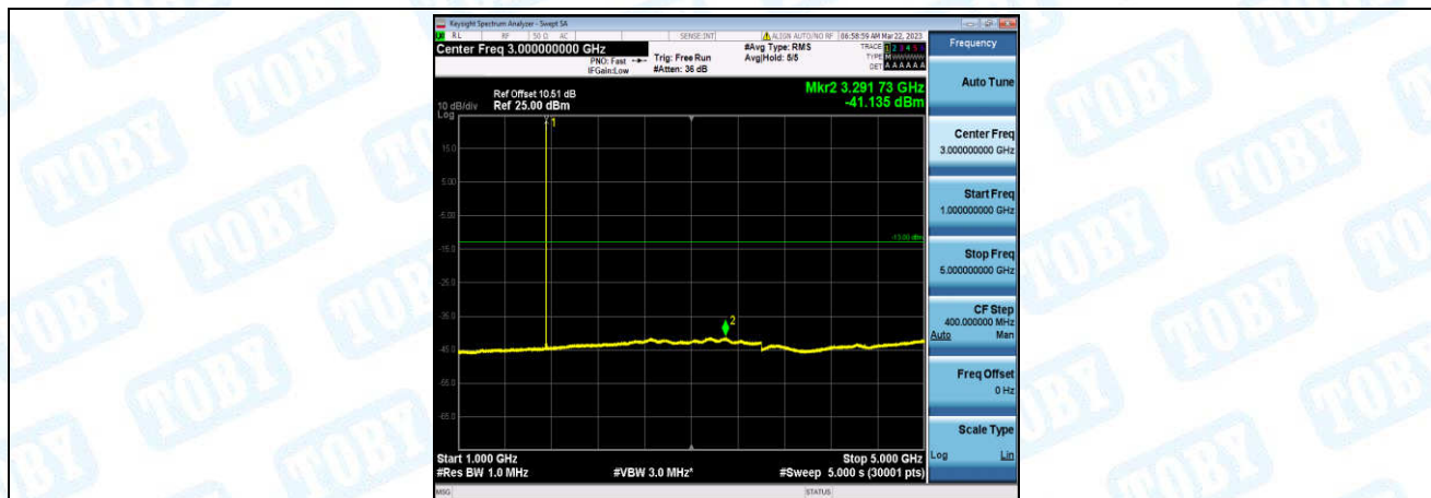
Band4-5MHz-16QAM-20375-1-0-High-1000-5000--41.14-PASS
