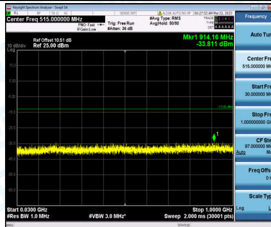
Band4-3MHz-16QAM-20385-1-0-High-30-1000--33.81-PASS
