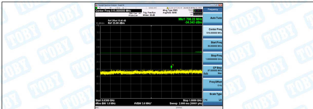
Band4-5MHz-QPSK-19975-1-0-Low-30-1000--34.34-PASS
