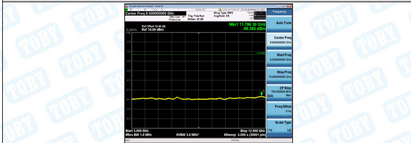
Band4-15MHz-QPSK-20025-1-0-Low-5000-12000--56.39-PASS
