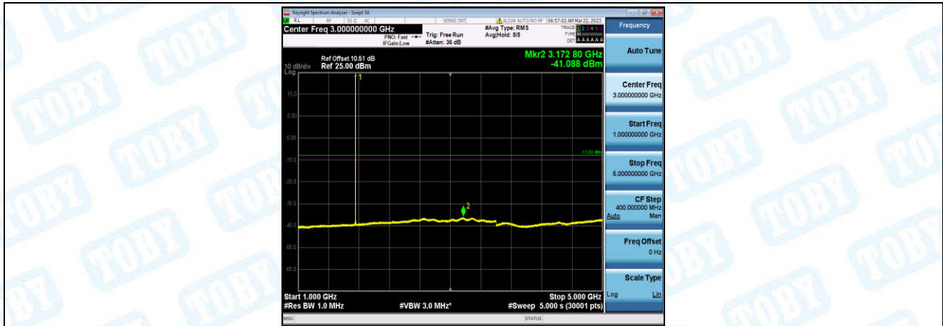
Band4-5MHz-QPSK-20375-1-0-High-1000-5000--41.09-PASS
