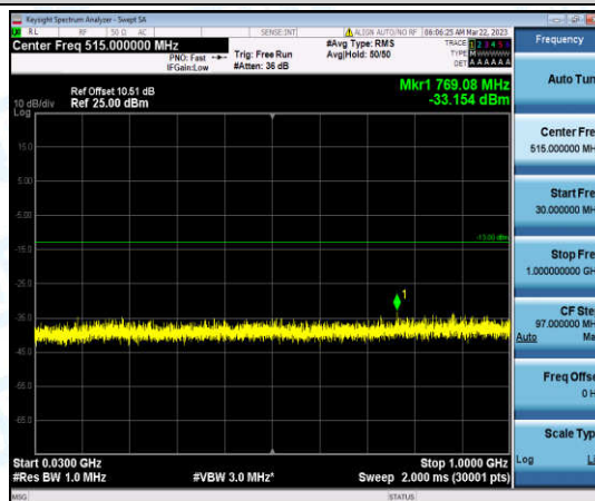
Band4-1.4MHz-QPSK-20393-1-0-High-30-1000--33.15-PASS
