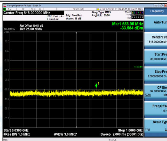
Band4-3MHz-QPSK-20385-1-0-High-30-1000--33.58-PASS
