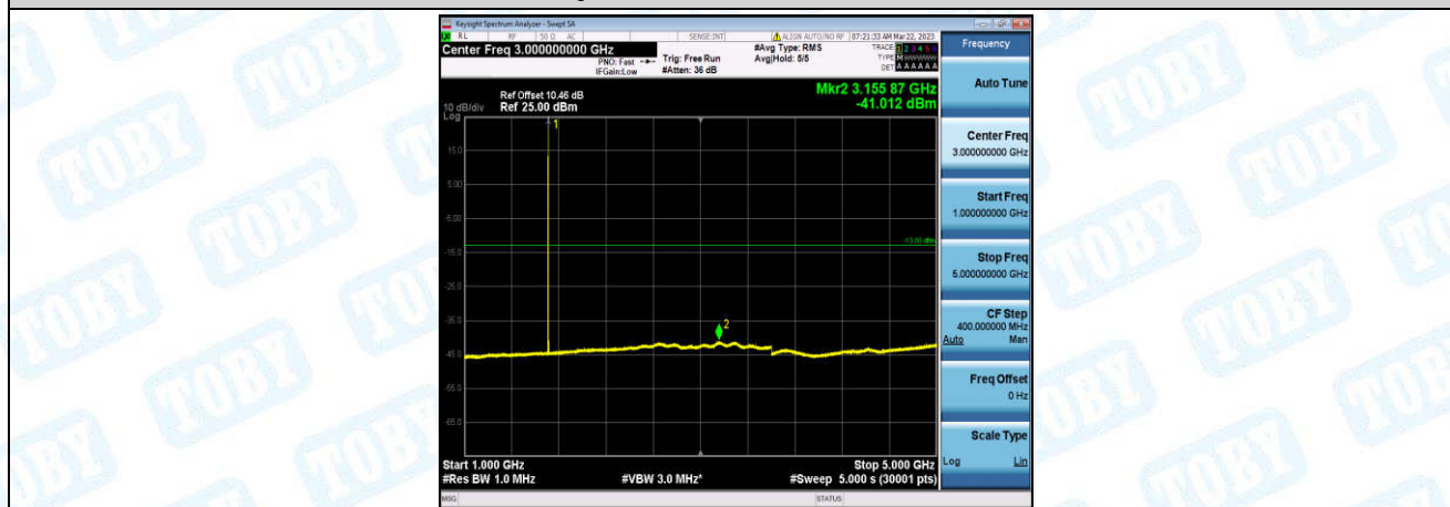
Band4-10MHz-16QAM-20000-1-0-Low-1000-5000--41.01-PASS
