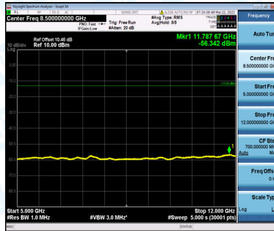
Band4-10MHz-QPSK-20175-1-0-Low-5000-12000--56.34-PASS
