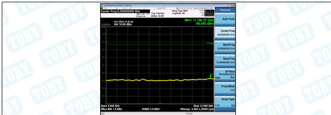
Band4-1.4MHz-16QAM-20175-1-0-Low-5000-12000--56.5-PASS
