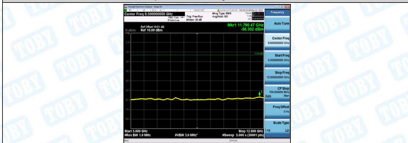
Band4-5MHz-16QAM-20375-1-0-High-5000-12000--56.3-PASS
