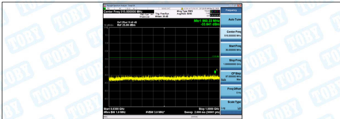
Band4-10MHz-16QAM-20000-1-0-Low-30-1000--33.64-PASS
