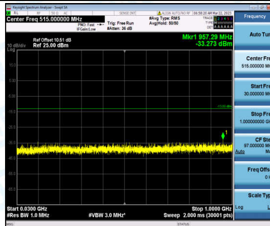
Band4-5MHz-16QAM-20375-1-0-High-30-1000--33.27-PASS
