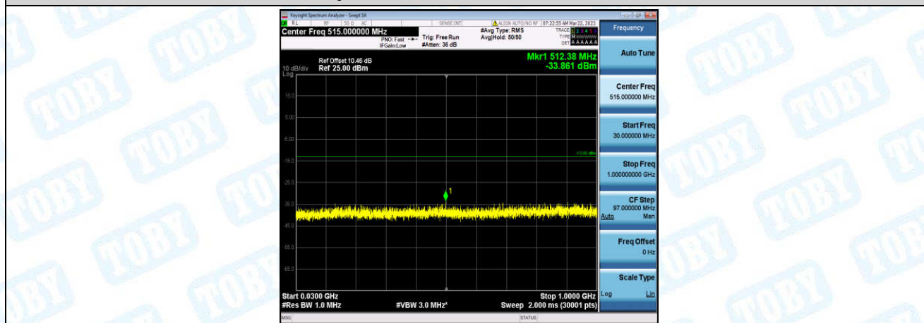
Band4-10MHz-QPSK-20175-1-0-Low-30-1000--33.86-PASS
