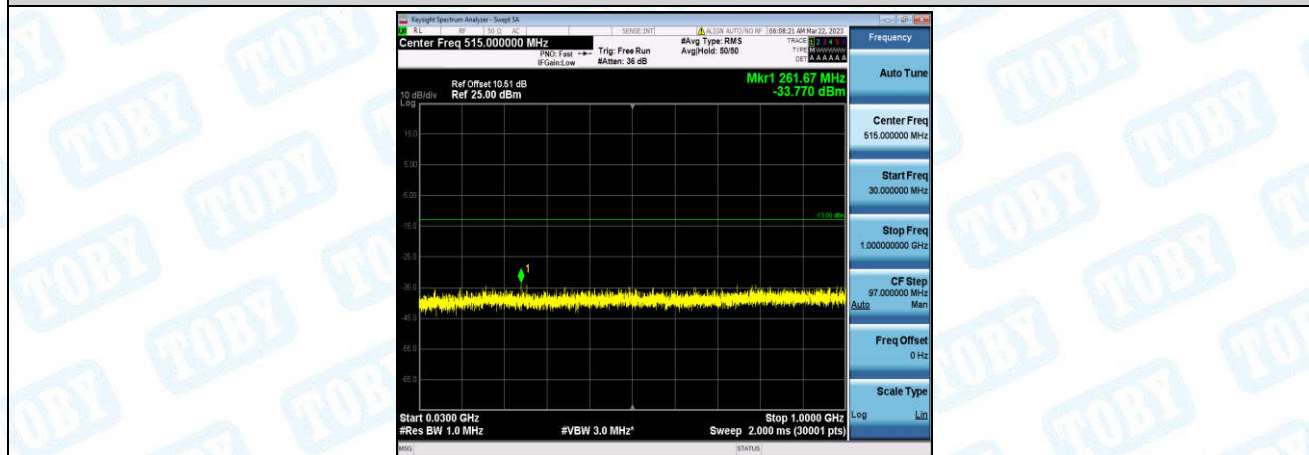
Band4-1.4MHz-16QAM-20393-1-0-High-30-1000--33.77-PASS
