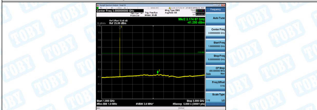
Band4-15MHz-QPSK-20025-1-0-Low-1000-5000--41.25-PASS
