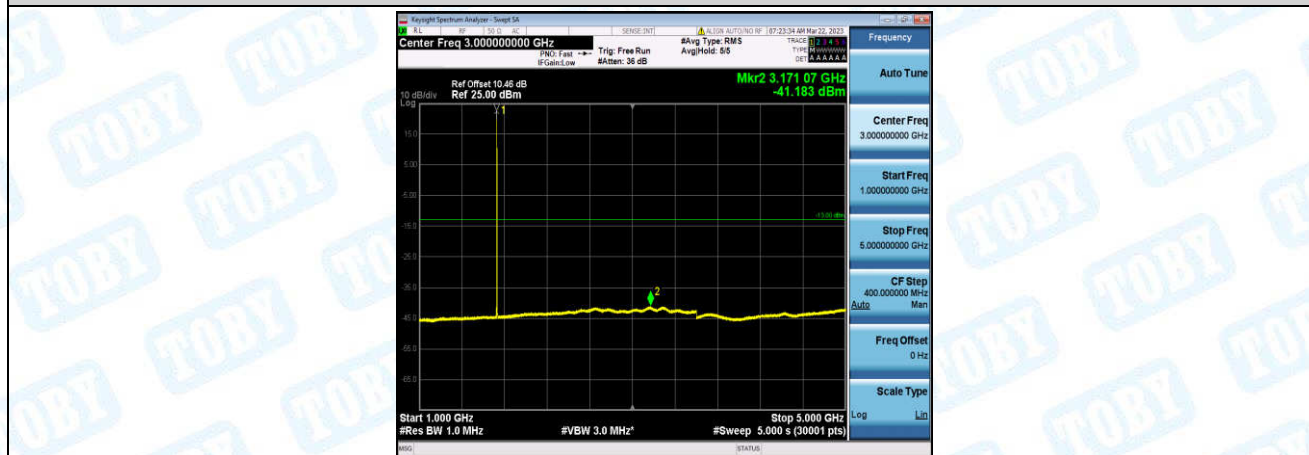
Band4-10MHz-QPSK-20175-1-0-Low-1000-5000--41.18-PASS
