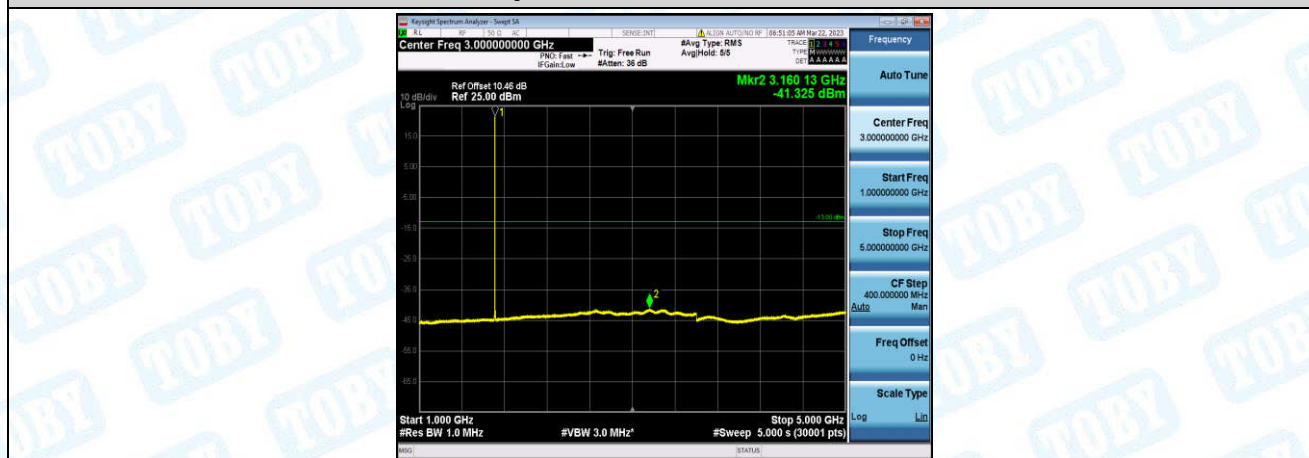
Band4-5MHz-16QAM-19975-1-0-Low-1000-5000--41.33-PASS
