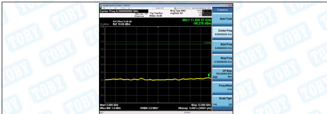
Band4-5MHz-QPSK-20175-1-0-Low-5000-12000--56.28-PASS
