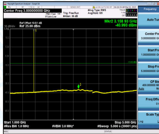
Band4-3MHz-QPSK-20385-1-0-High-1000-5000--40.99-PASS
