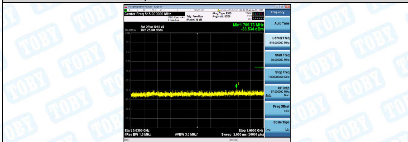
Band4-5MHz-QPSK-20375-1-0-High-30-1000--33.53-PASS
