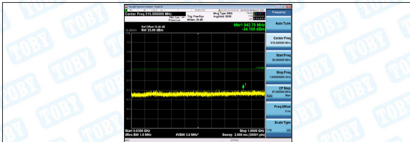
Band4-1.4MHz-16QAM-19957-1-0-Low-30-1000--34.11-PASS
