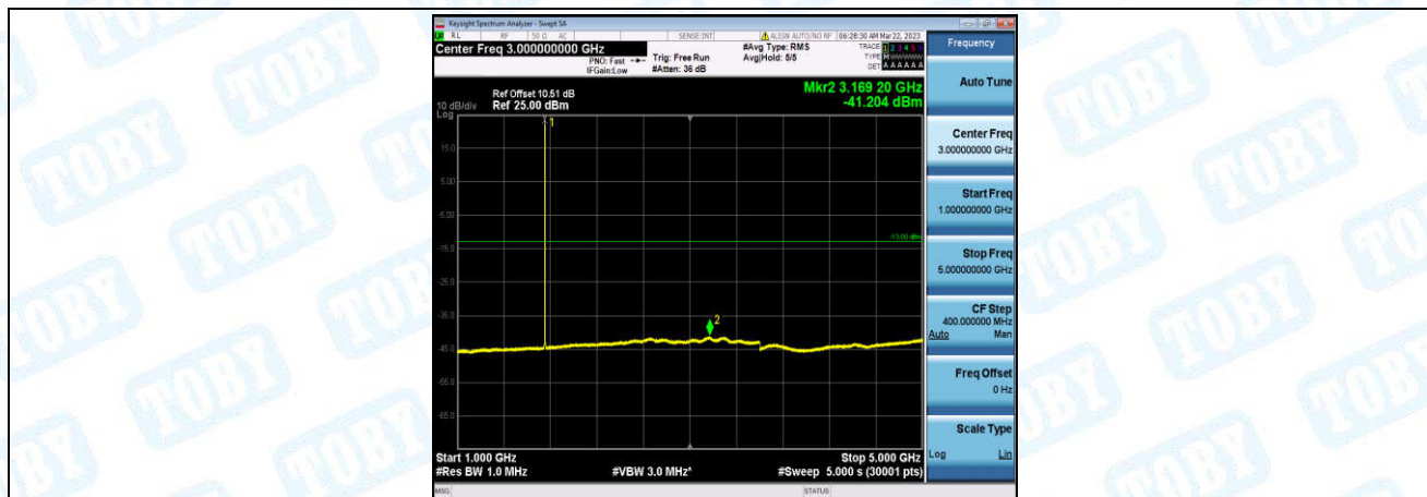
Band4-3MHz-16QAM-20385-1-0-High-1000-5000--41.2-PASS
