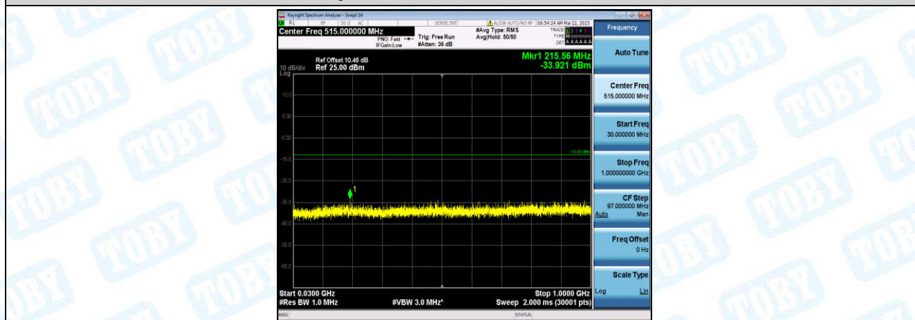
Band4-5MHz-16QAM-20175-1-0-Low-30-1000--33.92-PASS
