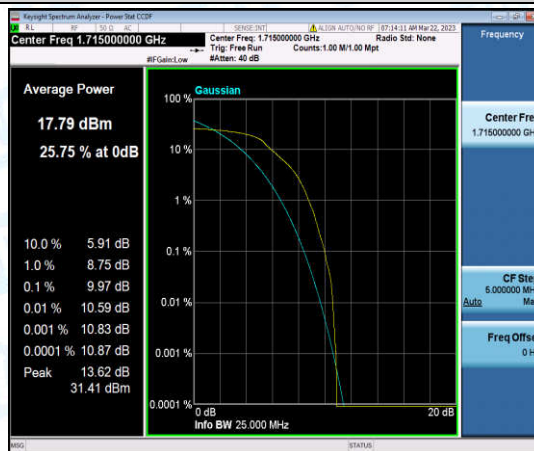
Band4-10MHz-16QAM-20000-6-0-Low-9.97-<=13-PASS
