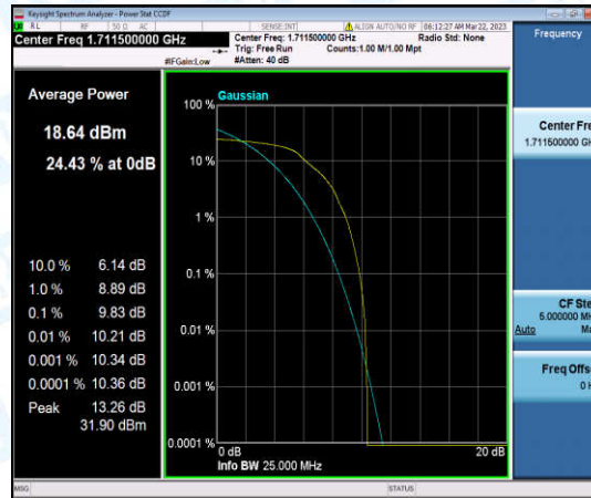
Band4-3MHz-QPSK-19965-1-0-Low-9.83-<=13-PASS
