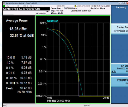
Band4-1.4MHz-QPSK-19957-6-0-Low-9.03-<=13-PASS
