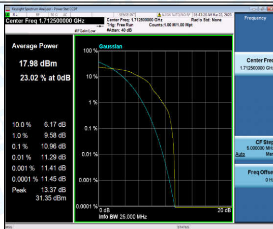
Band4-5MHz-16QAM-19975-1-0-Low-10.96-<=13-PASS
