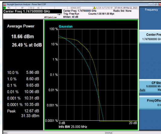
Band4-15MHz-QPSK-20325-6-0-High-9.65-<=13-PASS
