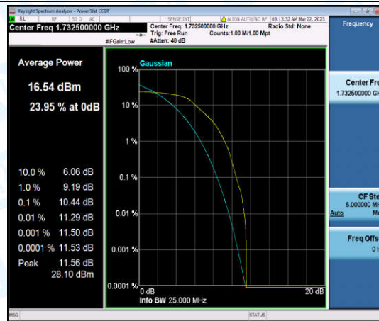
Band4-3MHz-QPSK-20175-6-0-High-10.44-<=13-PASS
