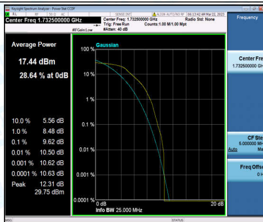
Band4-3MHz-16QAM-20175-6-0-Low-9.62-<=13-PASS
