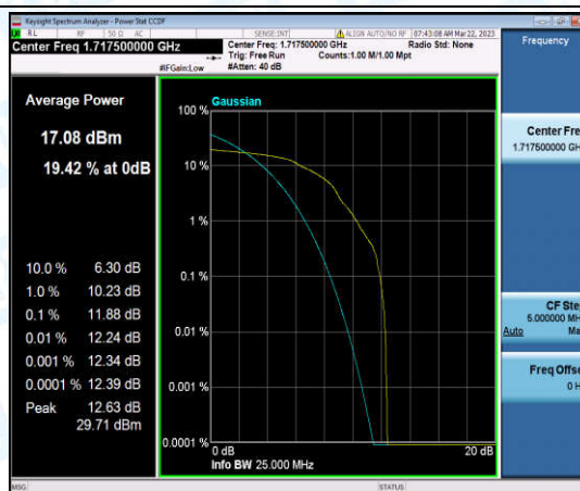
Band4-15MHz-16QAM-20025-1-0-Low-11.88-<=13-PASS
