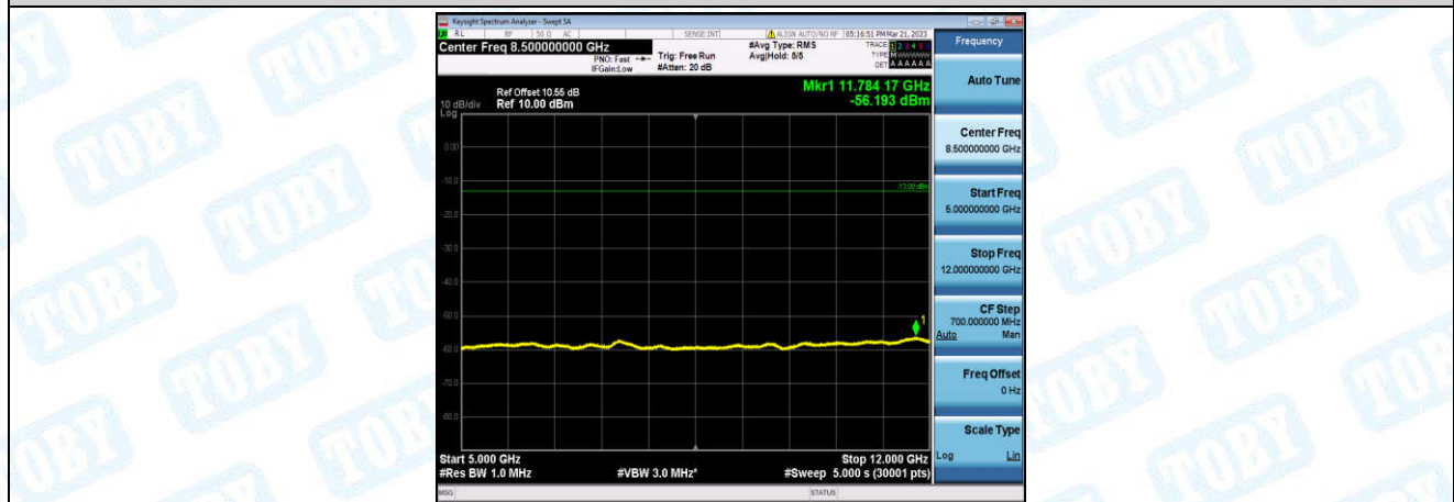
Band2-15MHz-16QAM-18675-1-0-Low-5000-12000--56.19-PASS
