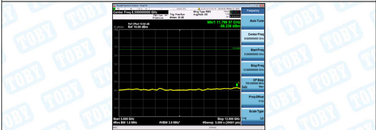
Band2-20MHz-16QAM-18700-1-0-Low-5000-12000--56.24-PASS
