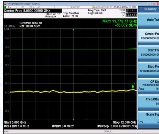
Band2-1.4MHz-QPSK-18900-1-0-Low-5000-12000--56-PASS
