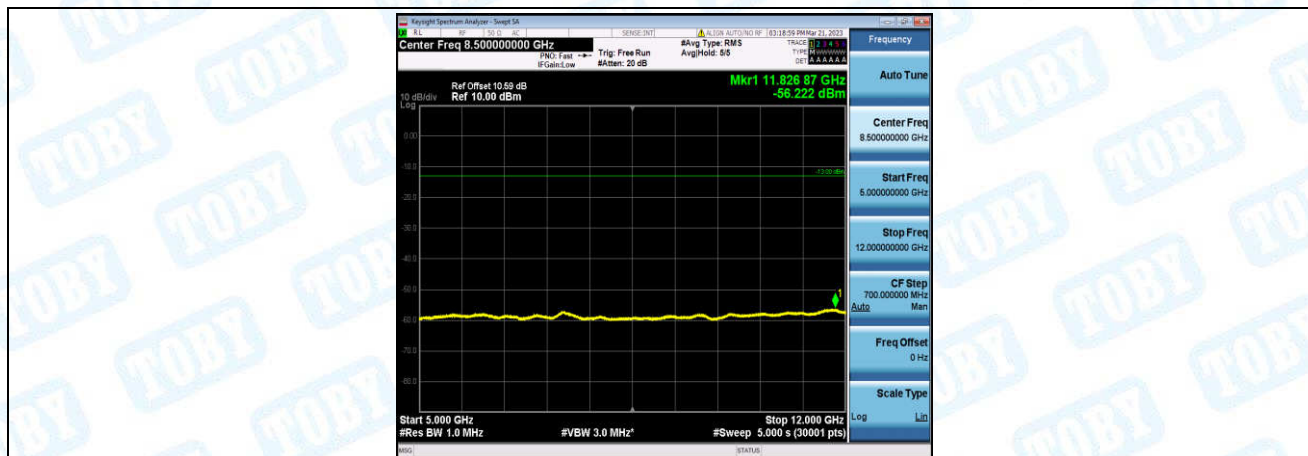
Band2-1.4MHz-16QAM-18900-1-0-Low-5000-12000--56.22-PASS
