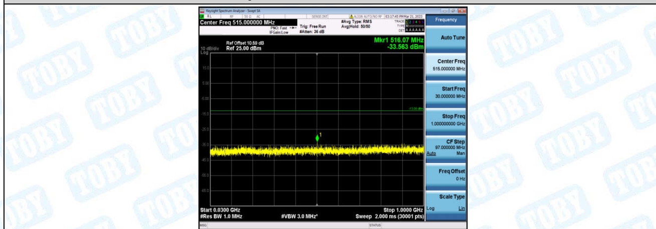
Band2-1.4MHz-16QAM-18900-1-0-Low-30-1000--33.56-PASS
