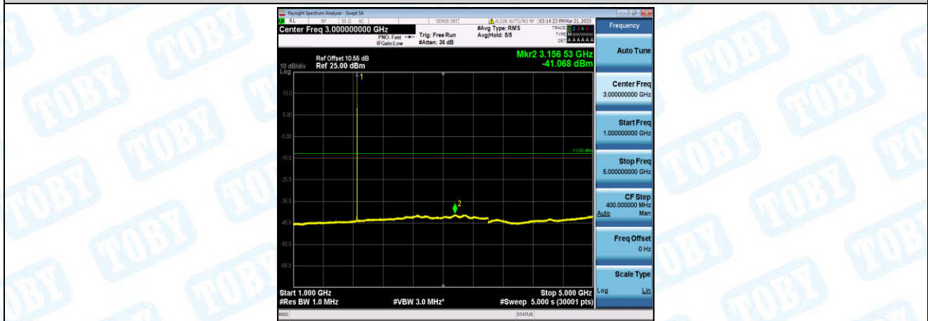
Band2-1.4MHz-16QAM-18607-1-0-Low-1000-5000--41.07-PASS
