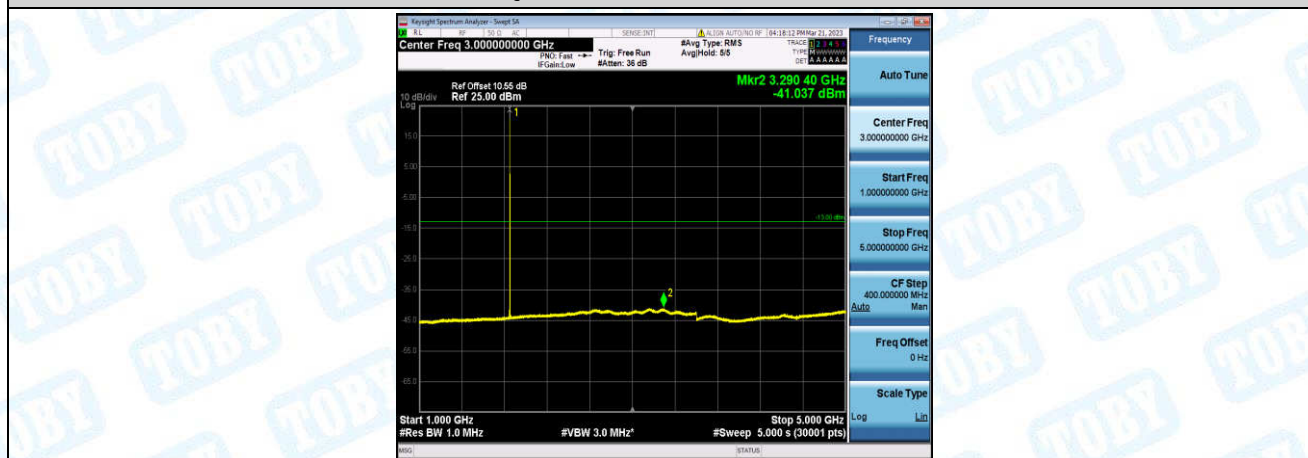
Band2-5MHz-16QAM-18625-1-0-Low-1000-5000--41.04-PASS
