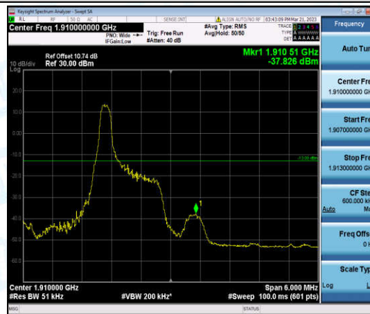
Band2-3MHz-QPSK-19185-1-0-High--37.83-PASS
