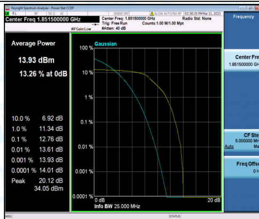
Band2-3MHz-QPSK-18615-6-0-Low-12.76-<=13-PASS
