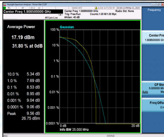
Band2-3MHz-16QAM-19185-6-0-High-8.53-<=13-PASS
