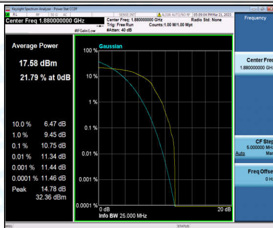
Band2-15MHz-16QAM-18900-1-0-Low-10.75-<=13-PASS
