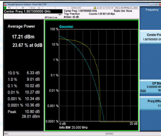
Band2-5MHz-16QAM-19175-1-0-High-10.02-<=13-PASS
