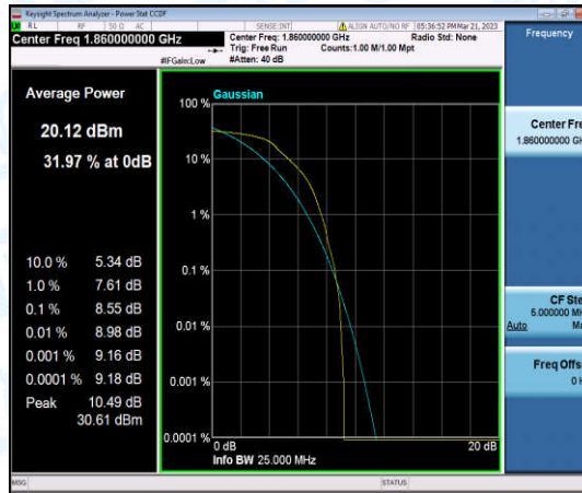
Band2-20MHz-16QAM-18700-6-0-Low-8.55-<=13-PASS
