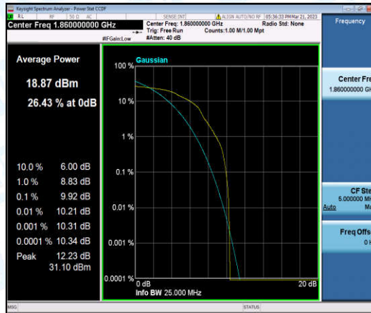
Band2-20MHz-16QAM-18700-1-0-Low-9.92-<=13-PASS
