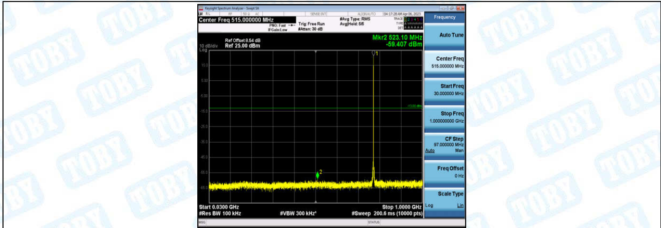
Band13-Stand-Alone-NaN-BPSK-23181-1@11-15kHz-30-1000-30~1000MHz@-59.41dBm--13-PASS
