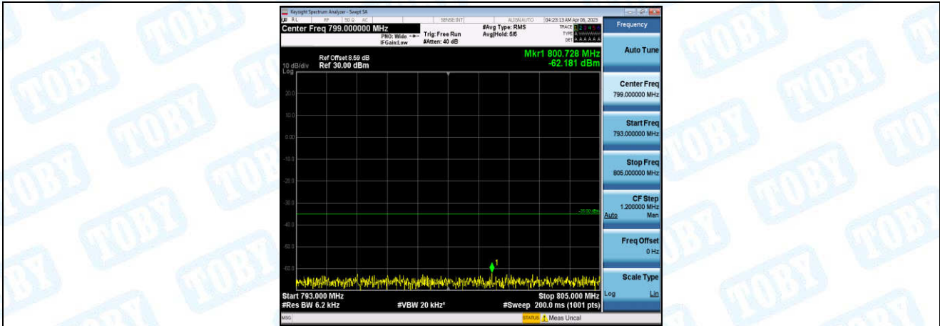
Band13-Stand-Alone-NaN-BPSK-23279-1@11-15kHz-793-805-793-805MHz@-62.18dBm--35-PASS
