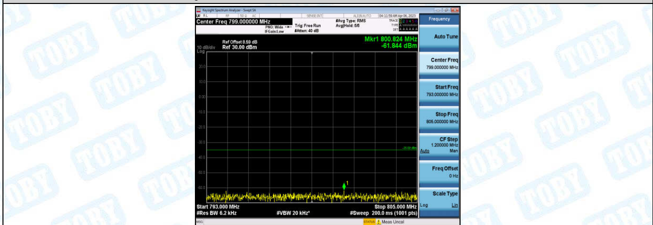
Band13-Stand-Alone-NaN-QPSK-23230-12@0-15kHz-793-805-793~805MHz@-61.84dBm--35-PASS
