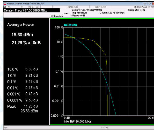
Band12-Stand-Alone-NaN-BPSK-23095-3@3-15kHz-9.43-<=13-PASS
