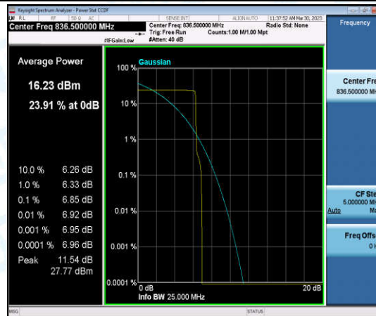
Band5-Stand-Alone-NaN-QPSK-20525-1@11-15kHz-6.85-<=13-PASS
