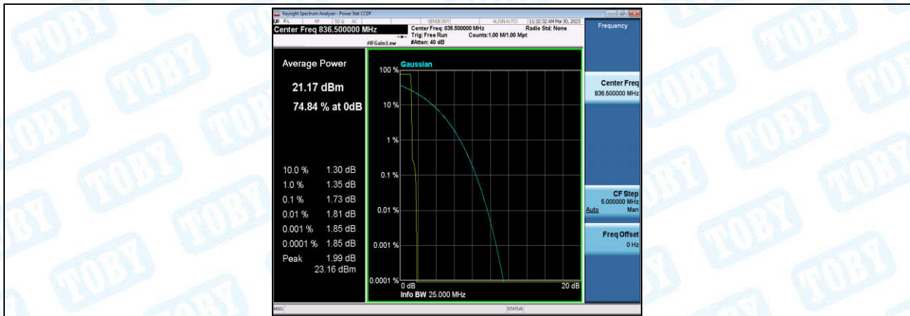
Band5-Stand-Alone-NaN-BPSK-20525-1@0-3.75kHz-1.73-<=13-PASS
