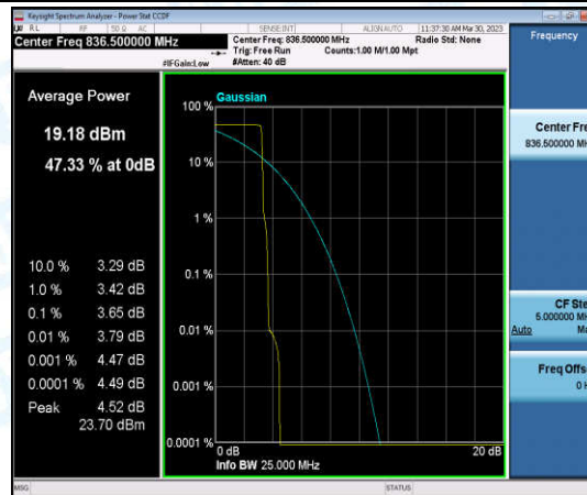
Band5-Stand-Alone-NaN-BPSK-20525-1@11-15kHz-3.65-<=13-PASS
