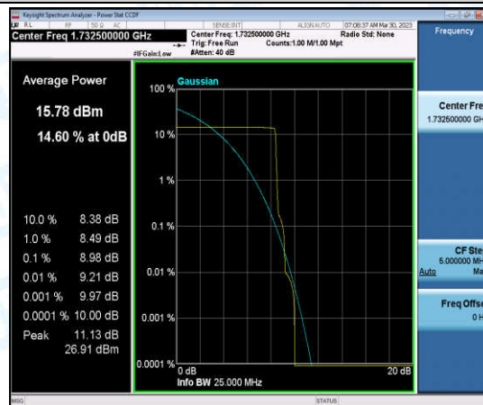
Band4-Stand-Alone-NaN-QPSK-20175-1@11-15kHz-8.98-<=13-PASS
