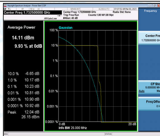
Band4-Stand-Alone-NaN-QPSK-20175-1@0-15kHz-10.23-<=13-PASS
