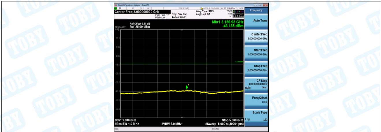
Band12-1.4MHz-QPSK-23173-1-0-High-1000-5000--43.14-PASS
