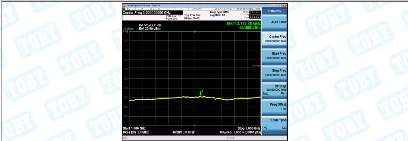
Band12-5MHz-16QAM-23095-1-0-Low-1000-5000--43.07-PASS
