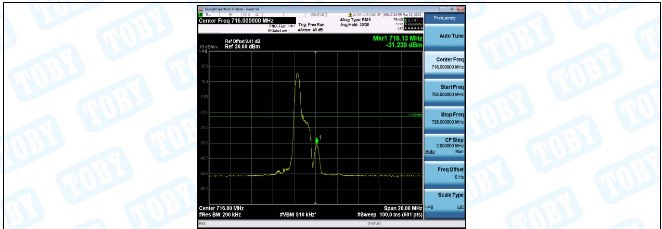
Band12-10MHz-16QAM-23130-1-0-High--31.23-PASS
