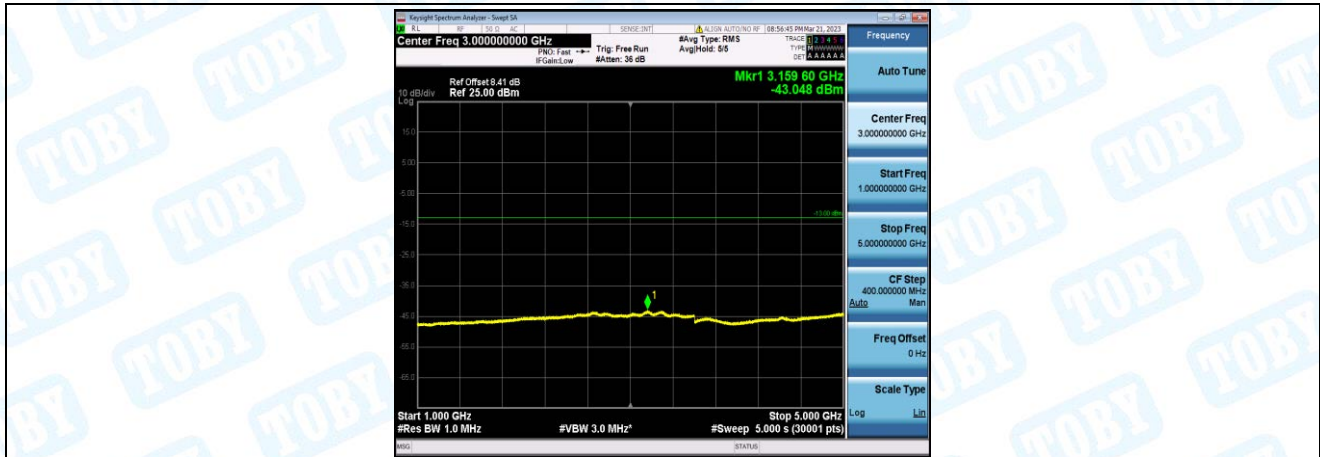
Band12-3MHz-16QAM-23165-1-0-High-1000-5000--43.05-PASS
