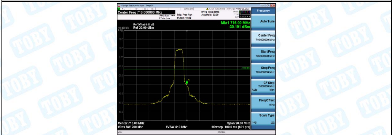
Band12-10MHz-16QAM-23130-6-0-High--30.19-PASS
