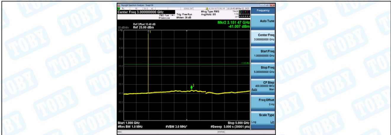
Band66-3MHz-QPSK-132657-1-0-High-1000-5000--41.01-PASS
