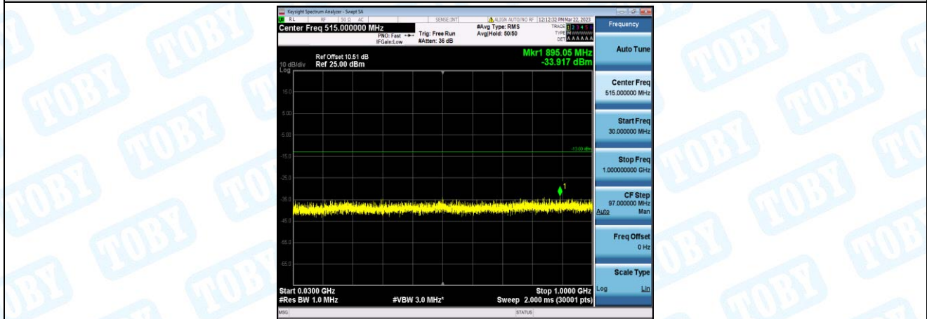
Band66-5MHz-16QAM-132322-1-0-Low-30-1000--33.92-PASS
