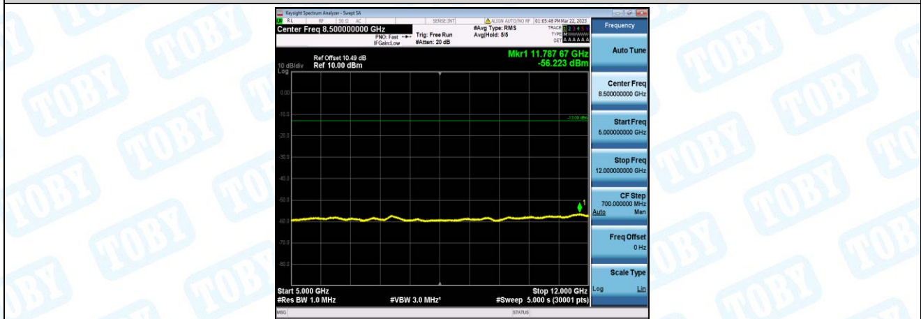
Band66-10MHz-16QAM-132622-1-0-High-5000-12000--56.22-PASS
