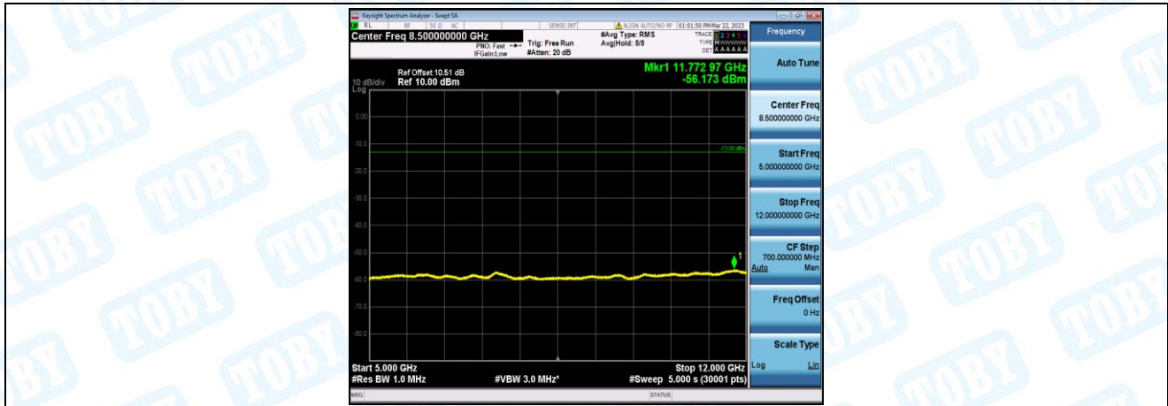
Band66-10MHz-16QAM-132322-1-0-Low-5000-12000--56.17-PASS
