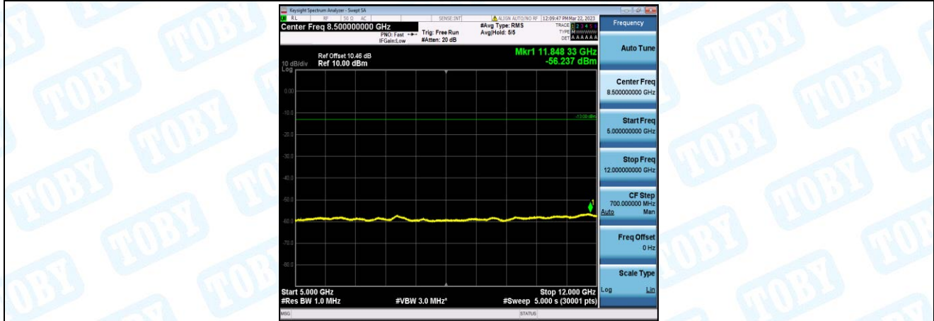
Band66-5MHz-16QAM-131997-1-0-Low-5000-12000--56.24-PASS
