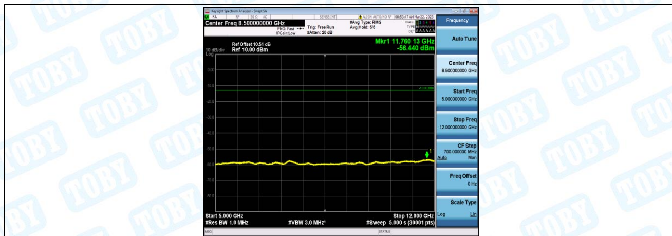
Band66-1.4MHz-QPSK-132322-1-0-Low-5000-12000--56.44-PASS
