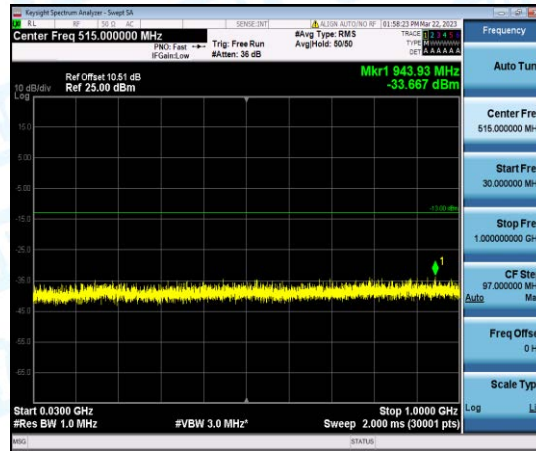
Band66-15MHz-QPSK-132322-1-0-Low-30-1000--33.67-PASS
