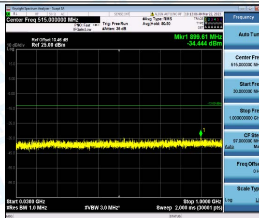
Band66-3MHz-16QAM-131987-1-0-Low-30-1000--34.44-PASS
