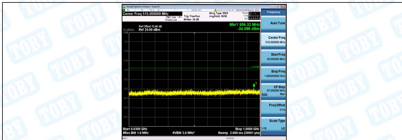
Band66-1.4MHz-16QAM-131979-1-0-Low-30-1000--34.1-PASS
