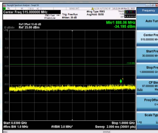
Band66-3MHz-16QAM-132657-1-0-High-30-1000--34.2-PASS
