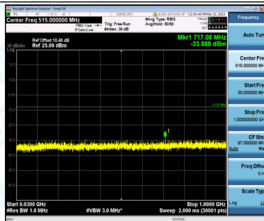
Band66-10MHz-QPSK-132022-1-0-Low-30-1000--33.89-PASS
