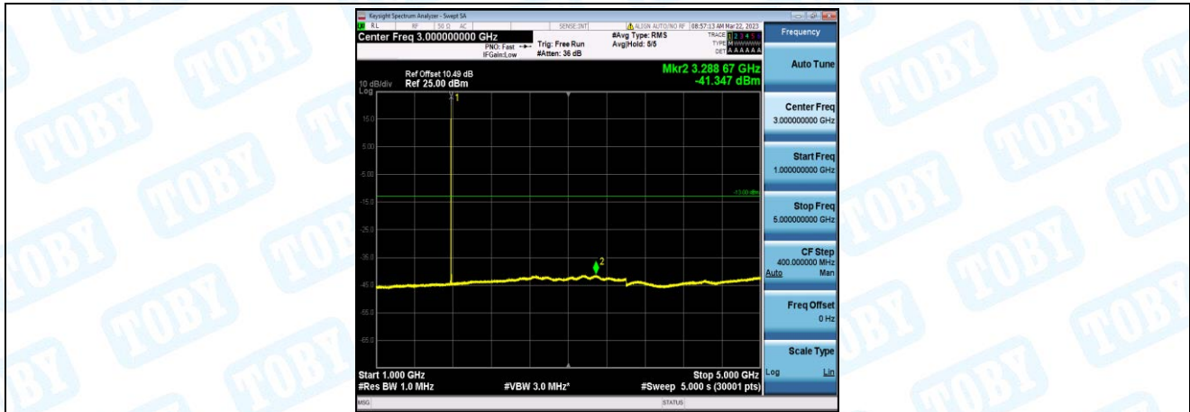
Band66-1.4MHz-QPSK-132665-1-0-High-1000-5000--41.35-PASS
