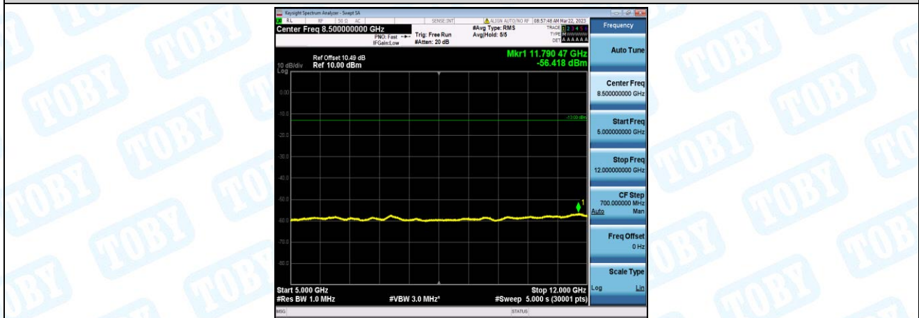
Band66-1.4MHz-QPSK-132665-1-0-High-5000-12000--56.42-PASS
