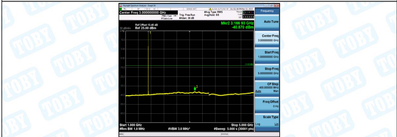
Band66-15MHz-QPSK-132047-1-0-Low-1000-5000--40.87-PASS
