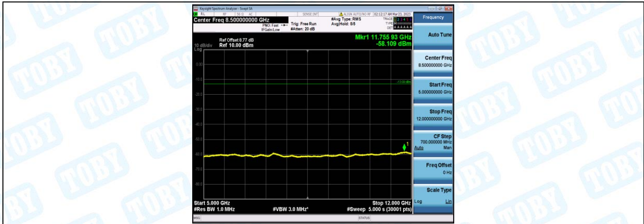
Band26-1.4MHz-16QAM-26915-1-0-Low-5000-12000--58.11-PASS
