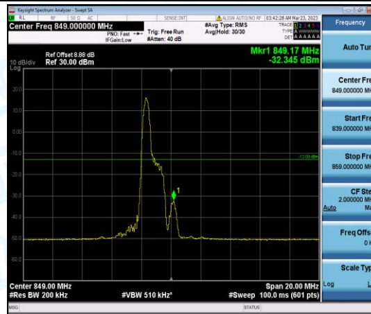
Band26-10MHz-16QAM-26990-1-0-High--32.34-PASS
