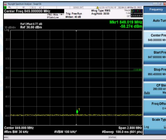
Band26-1.4MHz-16QAM-26915-6-0-Low--58.27-PASS
