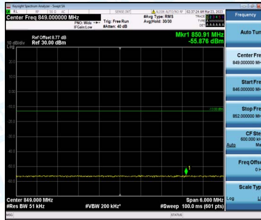
Band26-3MHz-QPSK-26915-6-0-Low--55.88-PASS
