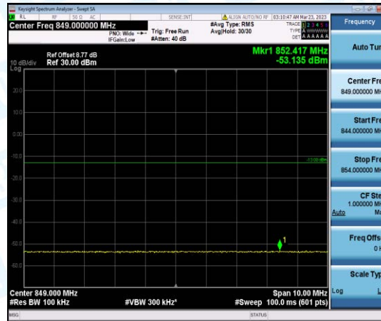
Band26-5MHz-16QAM-26915-6-0-Low--53.13-PASS
