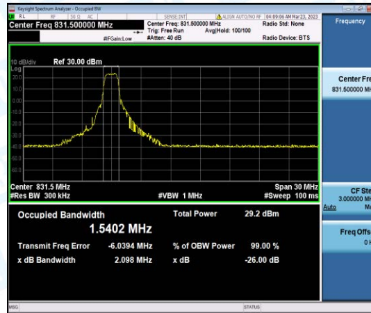
Band26-15MHz-QPSK-26865-6-0-Low-1.5402-2.098-PASS
