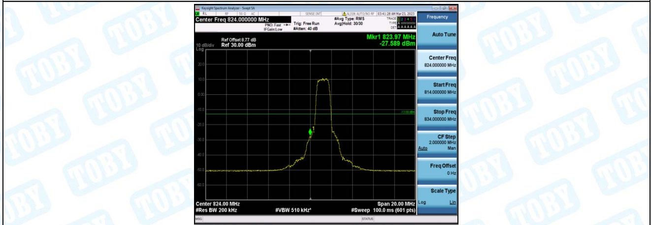
Band26-10MHz-16QAM-26840-6-0-Low--27.59-PASS
