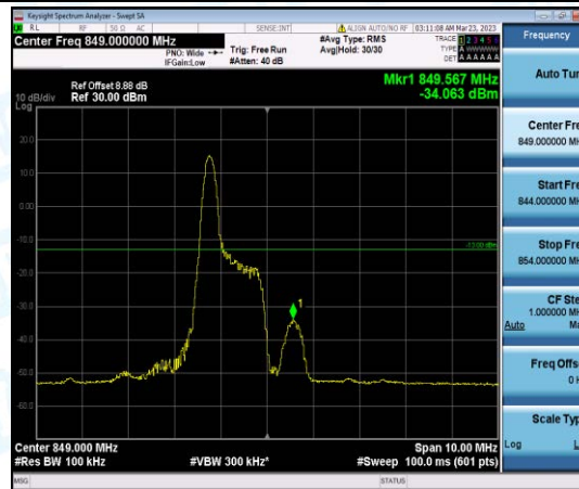
Band26-5MHz-16QAM-27015-1-0-High--34.06-PASS
