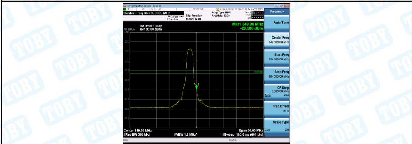
Band26-15MHz-16QAM-26965-6-0-High--29.58-PASS
