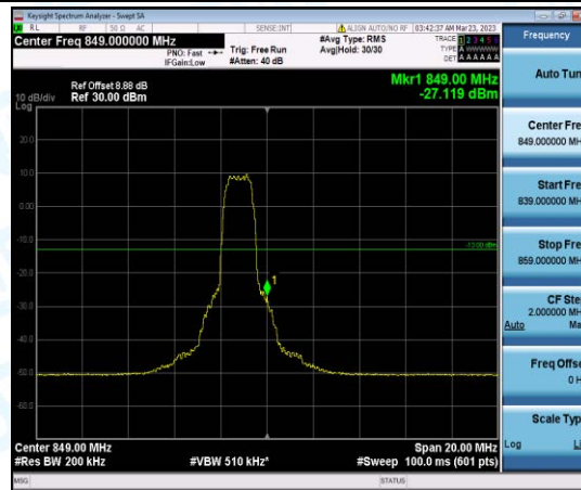
Band26-10MHz-QPSK-26990-6-0-High--27.12-PASS
