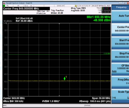
Band26-15MHz-QPSK-26915-1-0-Low--48.51-PASS
