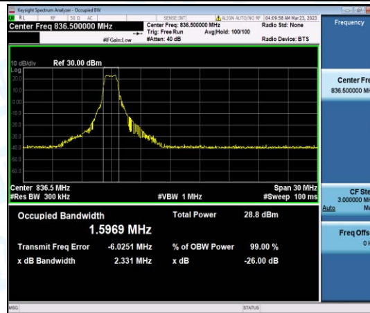
Band26-15MHz-16QAM-26915-6-0-Low-1.5969-2.331-PASS
