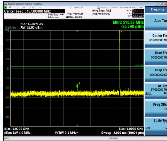
Band26-1.4MHz-16QAM-26797-1-0-Low-30-1000--35.79-PASS
