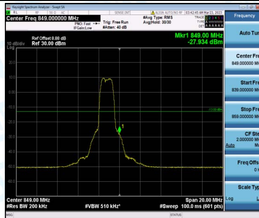
Band26-10MHz-16QAM-26990-6-0-High--27.93-PASS
