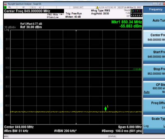
Band26-3MHz-16QAM-26915-1-0-Low--55.88-PASS
