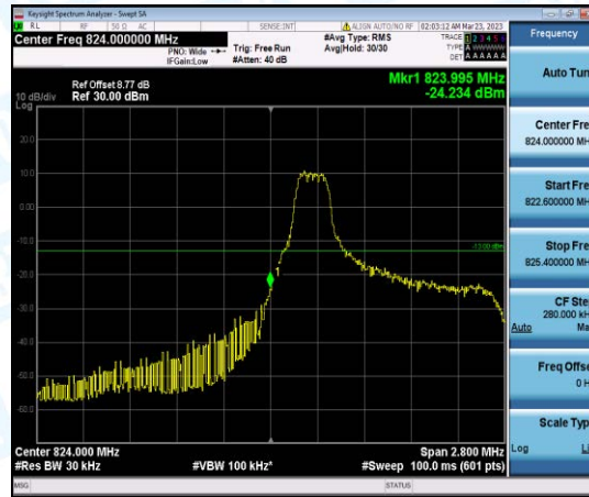
Band26-1.4MHz-16QAM-26797-1-0-Low--24.23-PASS
