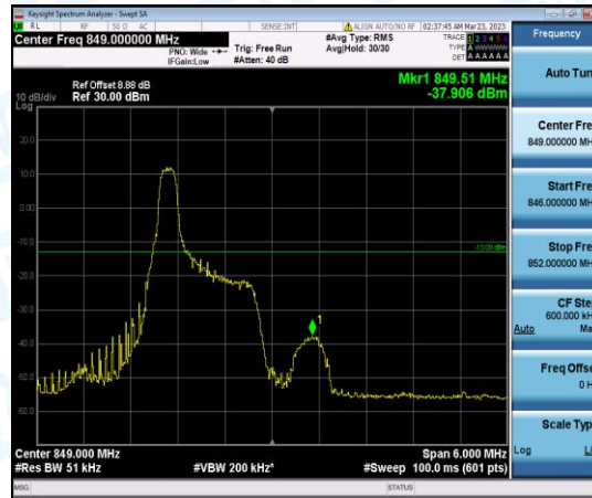
Band26-3MHz-QPSK-27025-1-0-High--37.91-PASS
