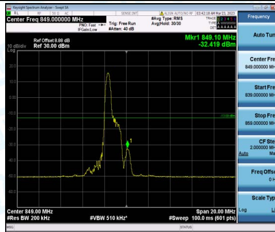
Band26-10MHz-QPSK-26990-1-0-High--32.42-PASS
