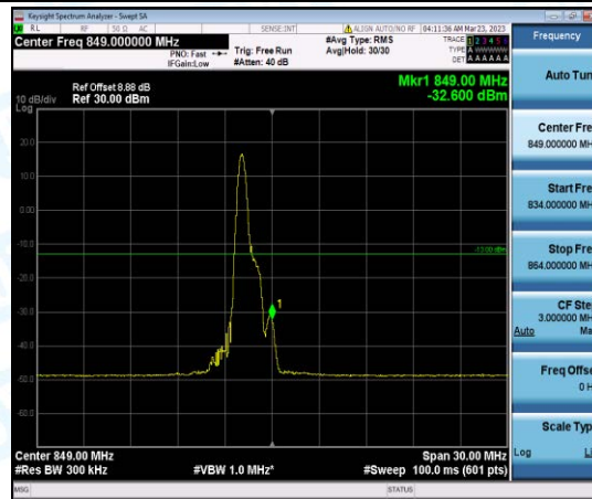
Band26-15MHz-QPSK-26965-1-0-High--32.60-PASS
