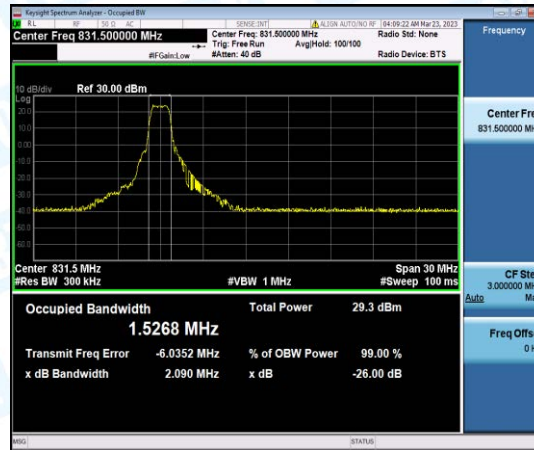
Band26-15MHz-16QAM-26865-6-0-Low-1.5268-2.090-PASS
