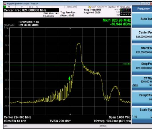
Band26-3MHz-16QAM-26805-1-0-Low--30.94-PASS
