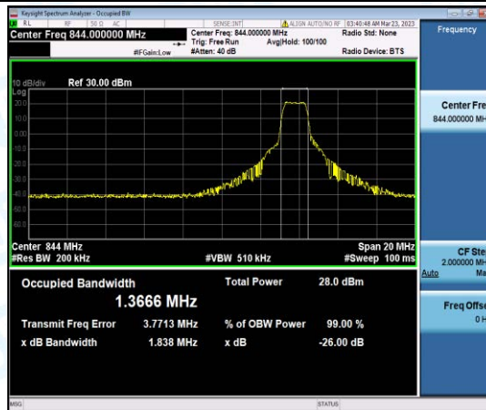
Band26-10MHz-16QAM-26990-6-0-High-1.3666-1.838-PASS
