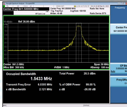
Band26-15MHz-QPSK-26965-6-0-High-1.5433-2.121-PASS
