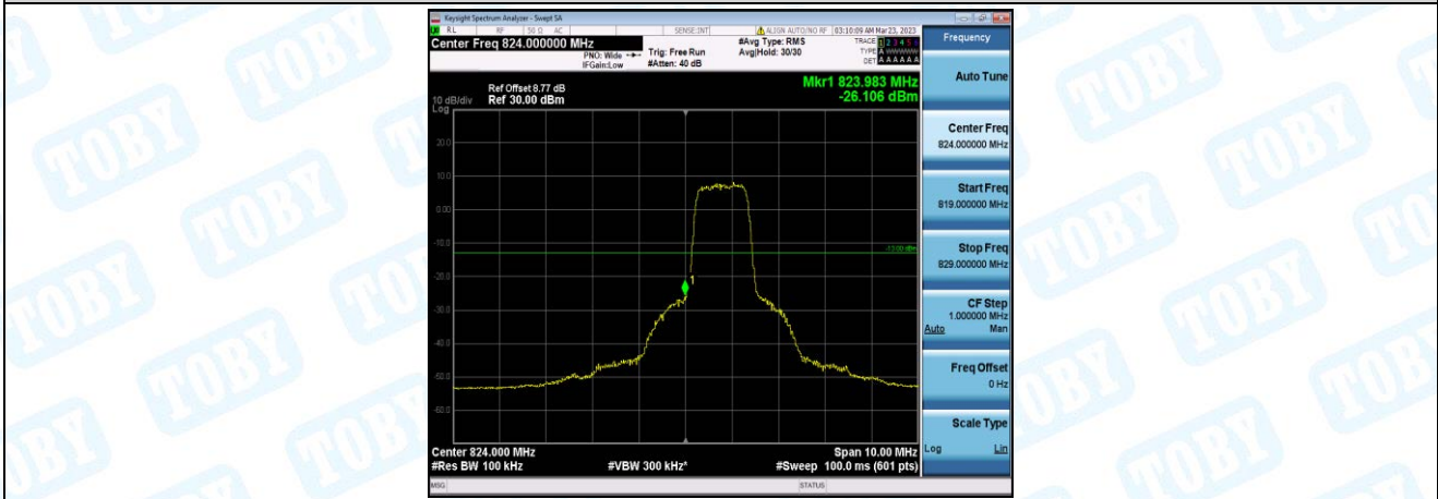
Band26-5MHz-16QAM-26815-6-0-Low--26.11-PASS
