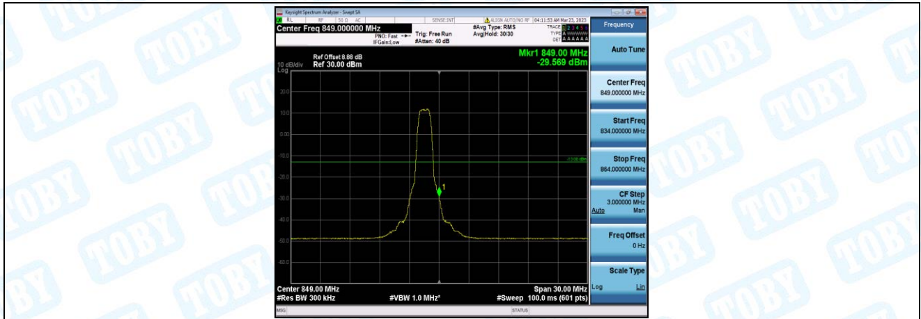
Band26-15MHz-QPSK-26965-6-0-High--29.57-PASS
