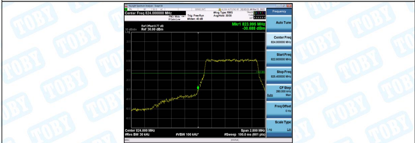
Band26-1.4MHz-QPSK-26797-6-0-Low--30.69-PASS
