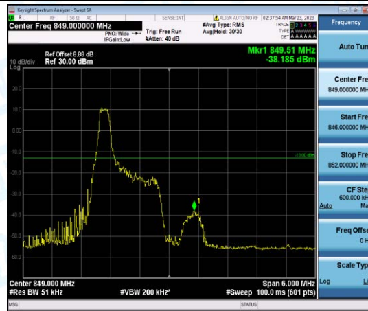
Band26-3MHz-16QAM-27025-1-0-High--38.18-PASS
