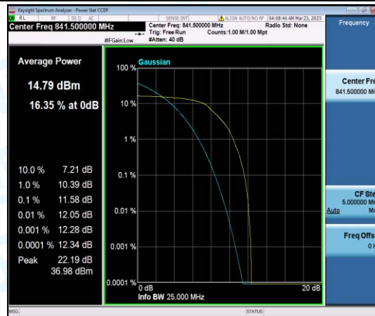
Band26-15MHz-16QAM-26965-6-0-High-11.58-13-PASS
