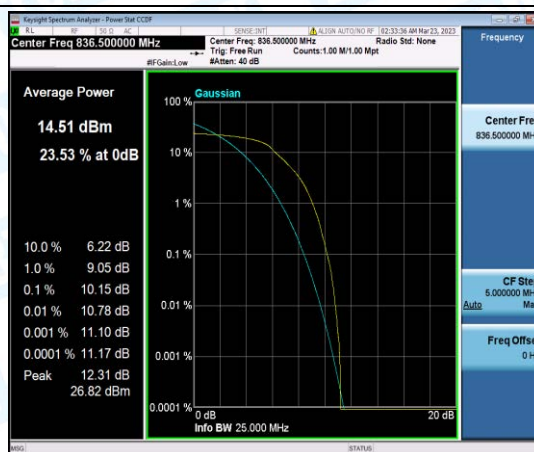
Band26-3MHz-16QAM-26915-6-0-Low-10.15-<=13-PASS
