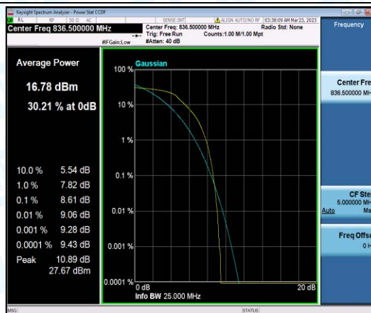
Band26-10MHz-QPSK-26915-6-0-Low-8.61-<=13-PASS
