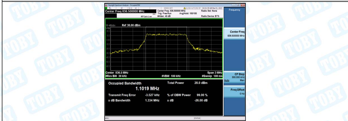
Band26-1.4MHz-QPSK-26915-6-0-Low-1.1019-1.334-PASS
