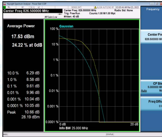
Band26-5MHz-QPSK-26815-1-0-Low-9.61-<=13-PASS
