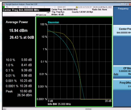
Band26-10MHz-QPSK-26990-6-0-High-9.39-<=13-PASS
