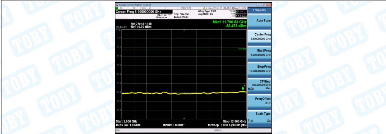
Band12-10MHz-16QAM-23130-1-0-High-5000-12000--58.47-PASS
