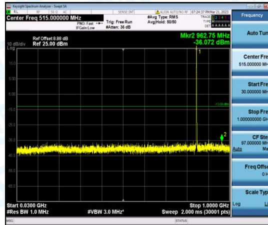
Band5-5MHz-16QAM-20625-1-0-High-30-1000--36.07-PASS
