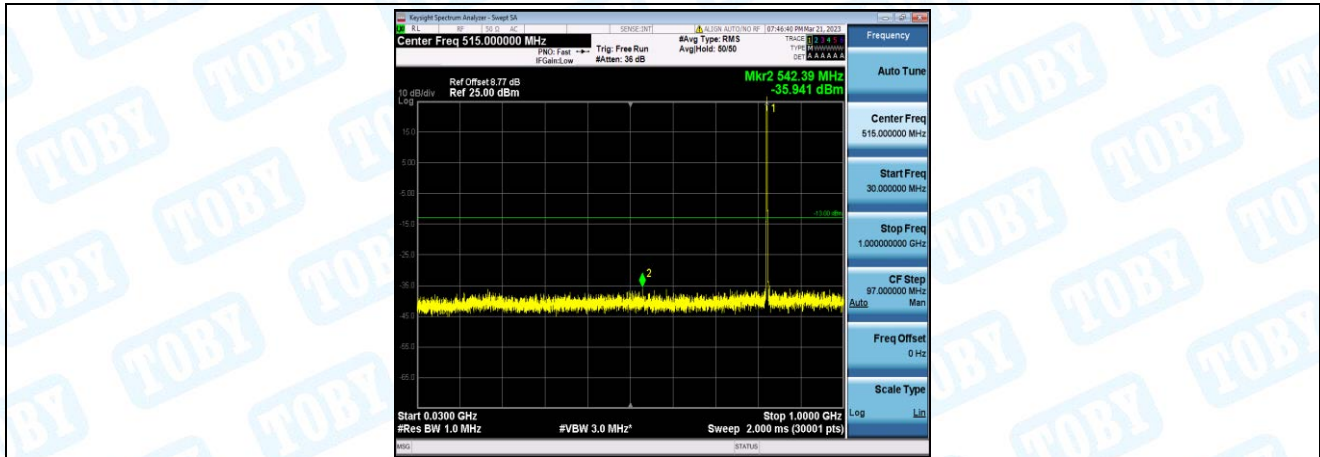
Band5-10MHz-16QAM-20450-1-0-Low-30-1000--35.94-PASS
