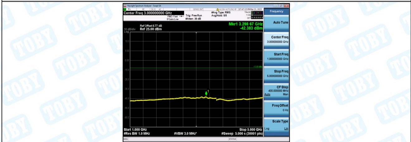
Band5-10MHz-16QAM-20450-1-0-Low-1000-5000--42.38-PASS
