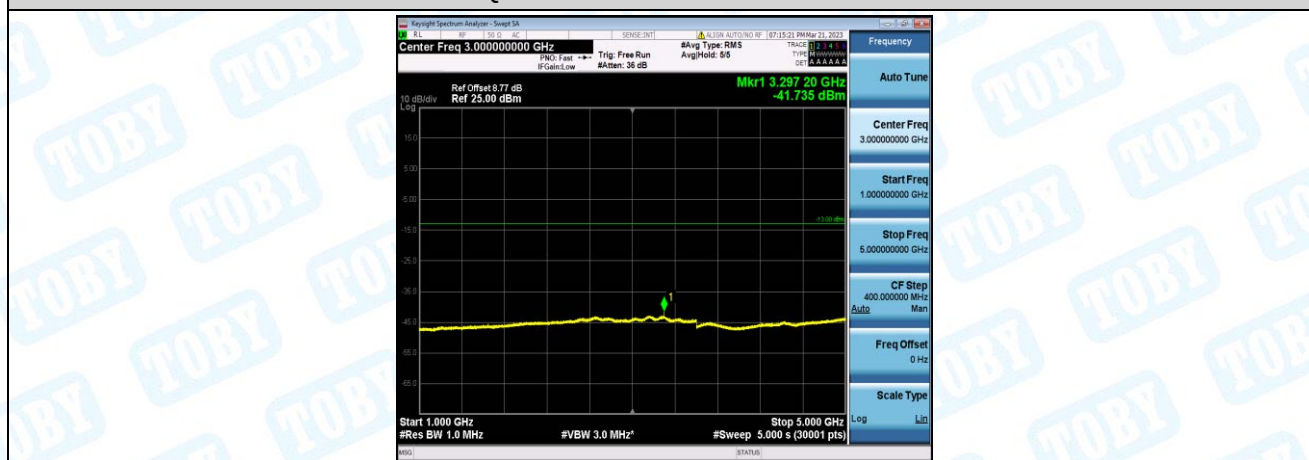
Band5-5MHz-QPSK-20425-1-0-Low-1000-5000--41.74-PASS
