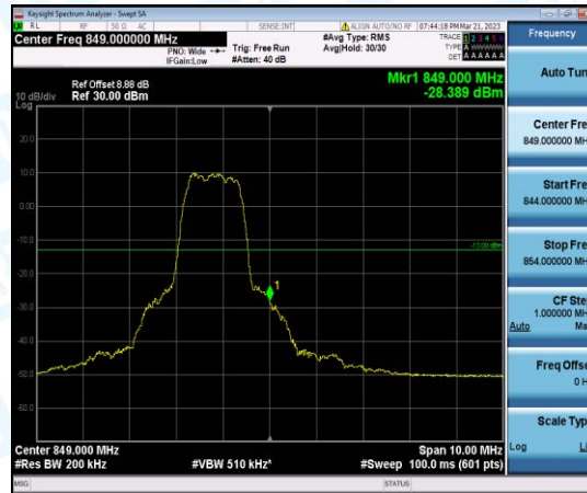
Band5-10MHz-QPSK-20600-6-0-High--28.39-PASS
