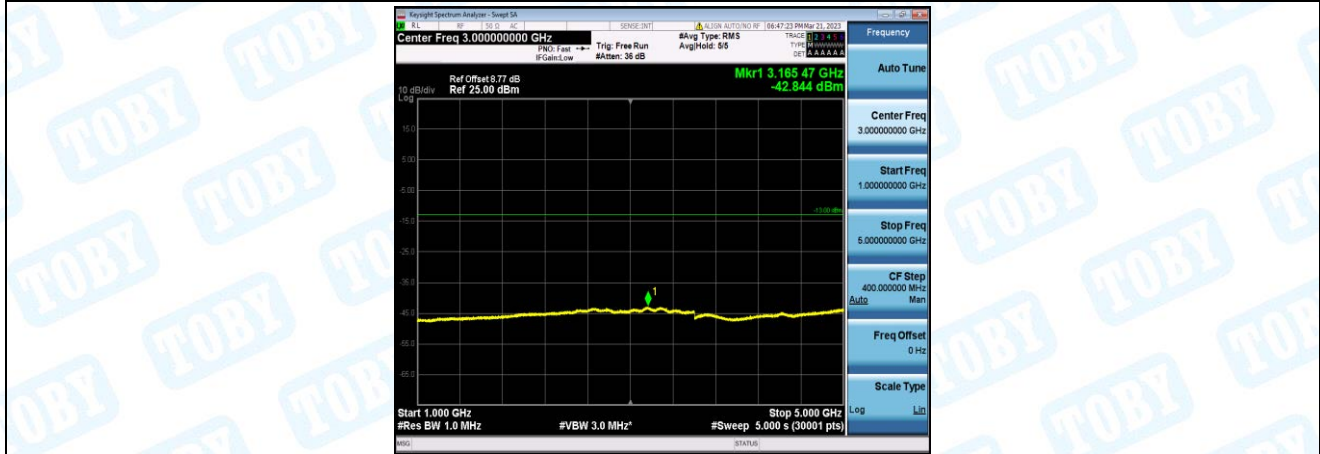
Band5-3MHz-QPSK-20525-1-0-Low-1000-5000--42.84-PASS
