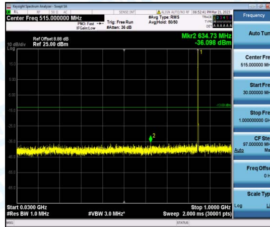
Band5-3MHz-16QAM-20635-1-0-High-30-1000--36.1-PASS
