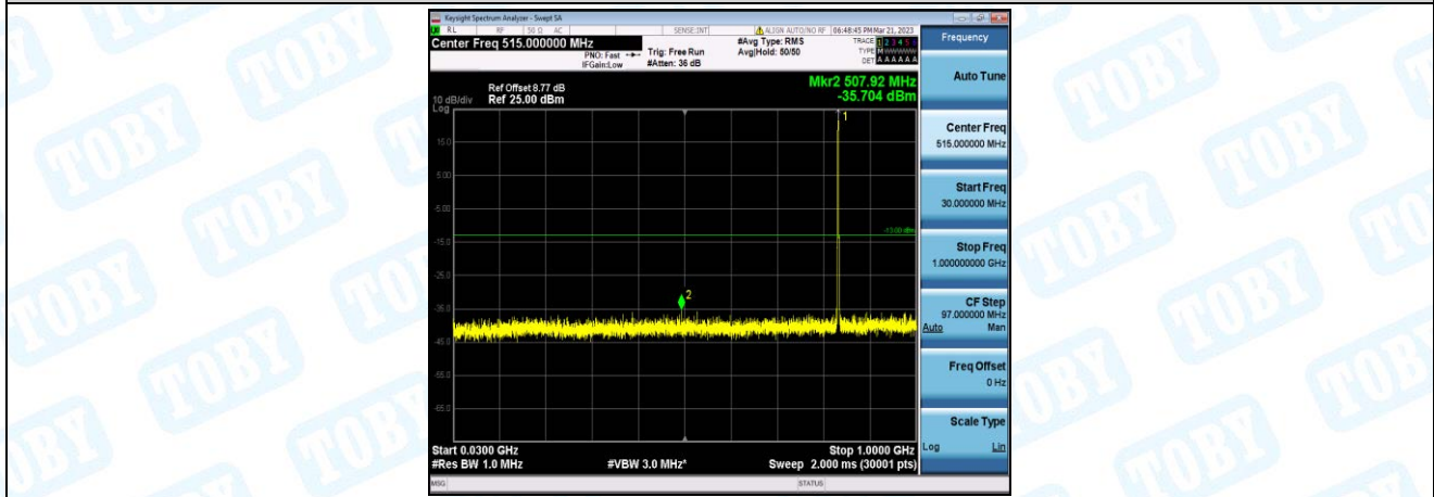
Band5-3MHz-16QAM-20525-1-0-Low-30-1000--35.7-PASS
