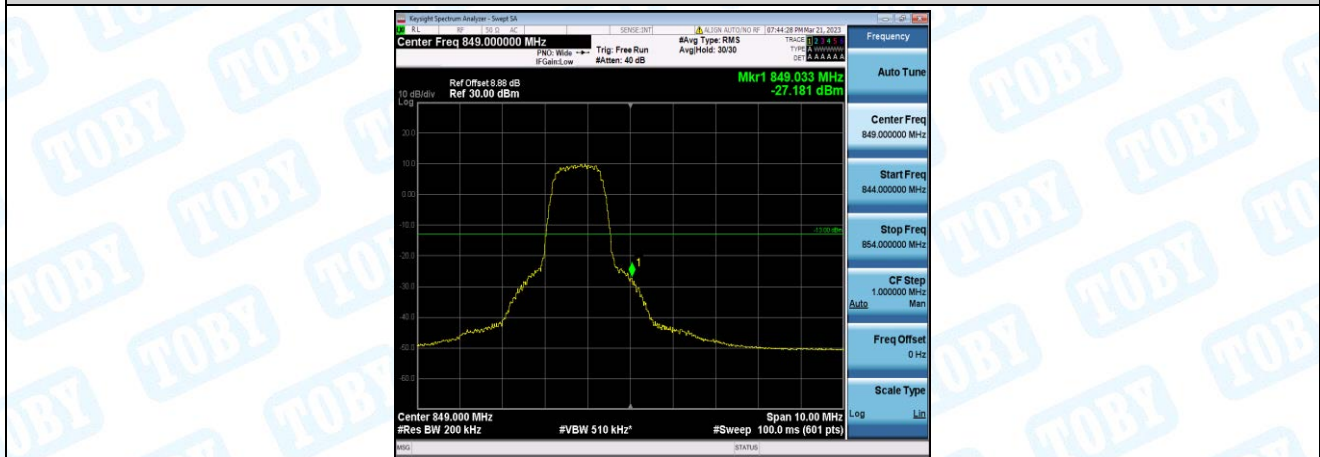
Band5-10MHz-16QAM-20600-6-0-High--27.18-PASS
