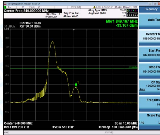
Band5-10MHz-QPSK-20600-1-0-High--33.11-PASS
