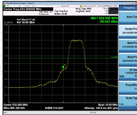
Band5-10MHz-QPSK-20450-6-0-Low--26.83-PASS
