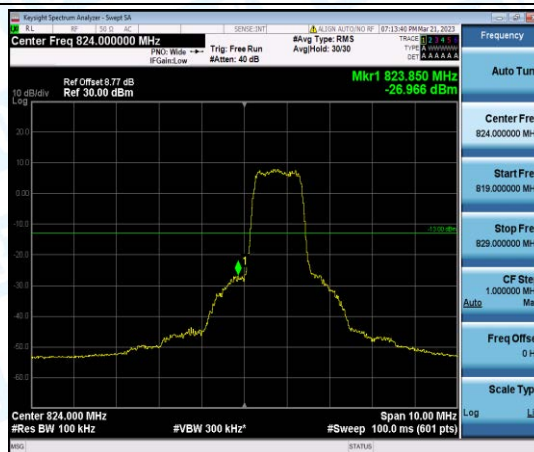
Band5-5MHz-16QAM-20425-6-0-Low--26.97-PASS
