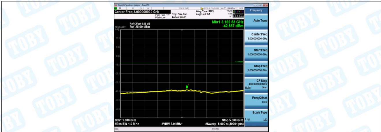
Band5-3MHz-16QAM-20635-1-0-High-1000-5000--42.66-PASS
