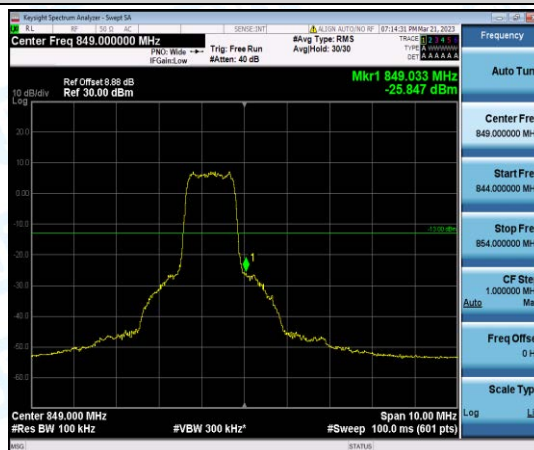
Band5-5MHz-16QAM-20625-6-0-High--25.85-PASS
