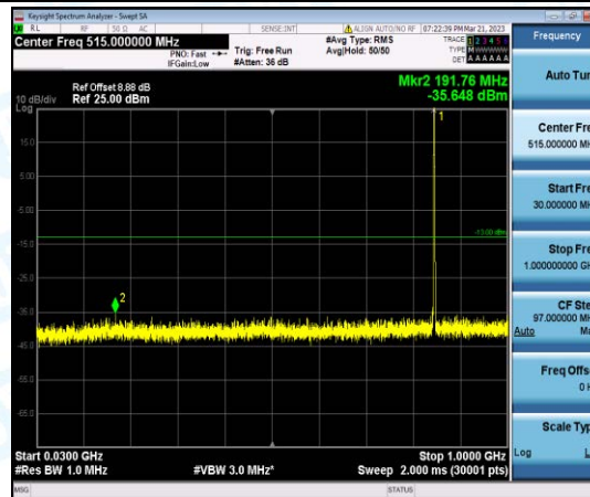
Band5-5MHz-QPSK-20625-1-0-High-30-1000--35.65-PASS
