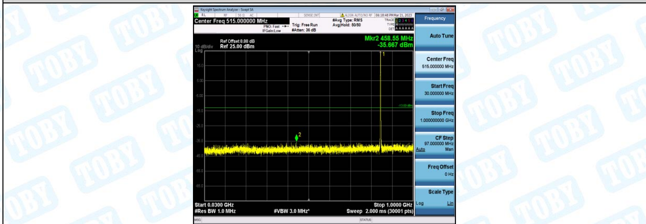
Band5-1.4MHz-QPSK-20643-1-0-High-30-1000--35.67-PASS
