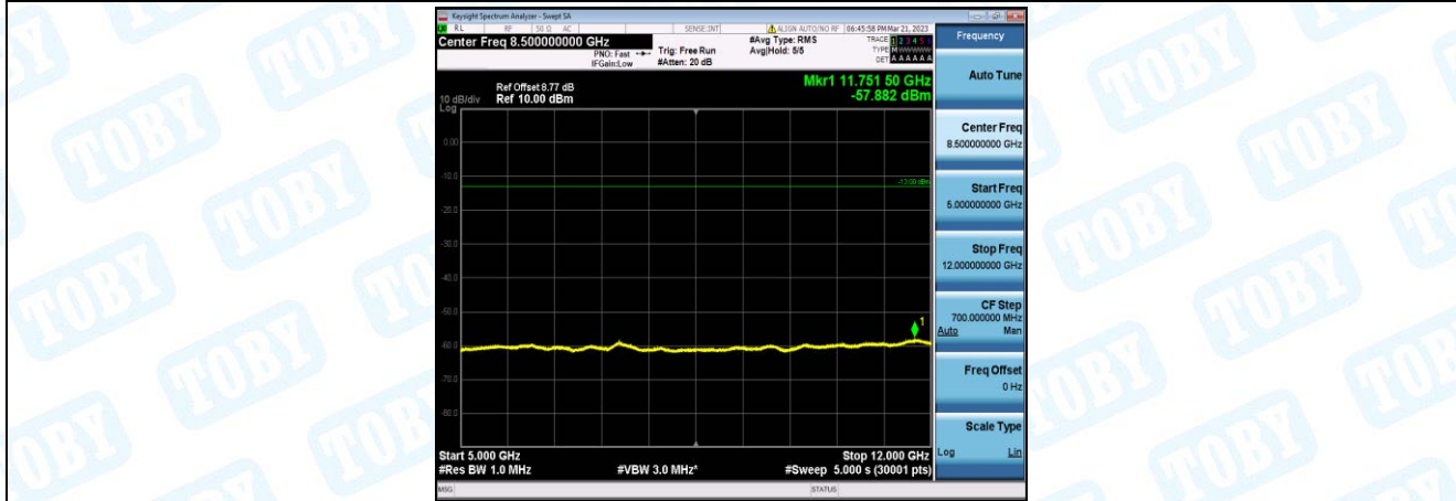
Band5-3MHz-16QAM-20415-1-0-Low-5000-12000--57.88-PASS
