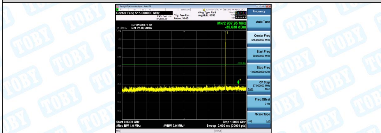
Band5-1.4MHz-16QAM-20525-1-0-Low-30-1000--35.64-PASS
