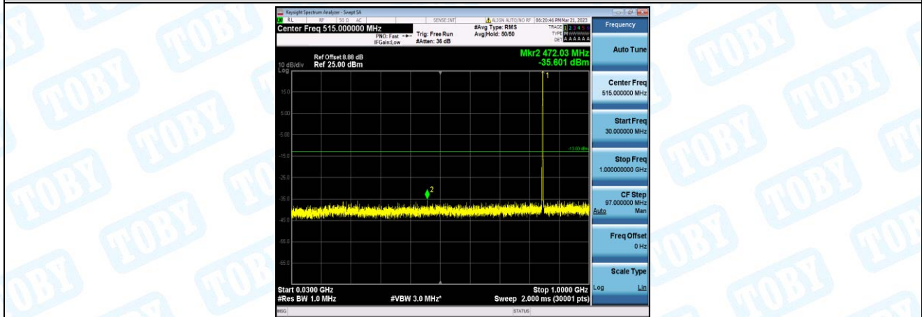
Band5-1.4MHz-16QAM-20643-1-0-High-30-1000--35.6-PASS
