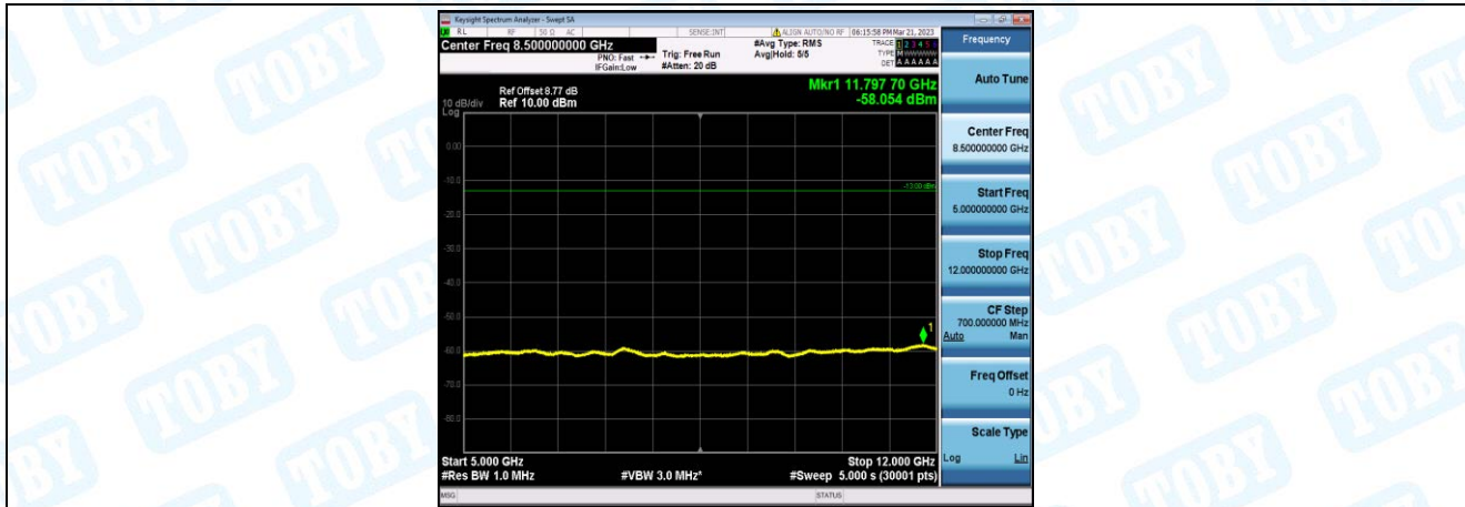
Band5-1.4MHz-QPSK-20525-1-0-Low-5000-12000--58.05-PASS
