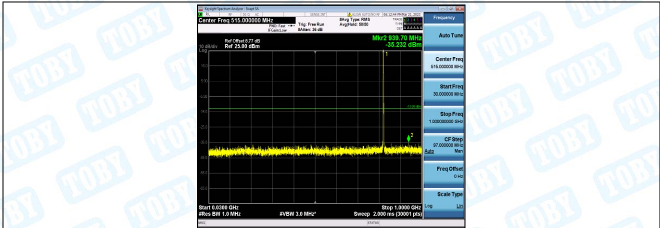
Band5-1.4MHz-16QAM-20407-1-0-Low-30-1000--35.23-PASS
