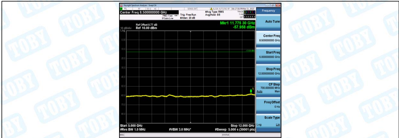
Band5-1.4MHz-16QAM-20525-1-0-Low-5000-12000--57.96-PASS
