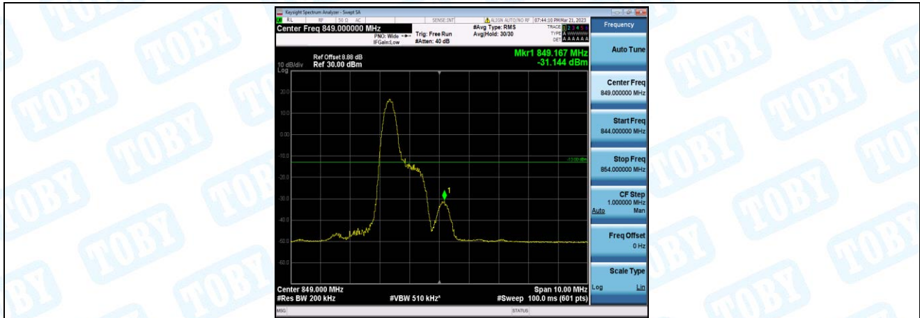
Band5-10MHz-16QAM-20600-1-0-High--31.14-PASS
