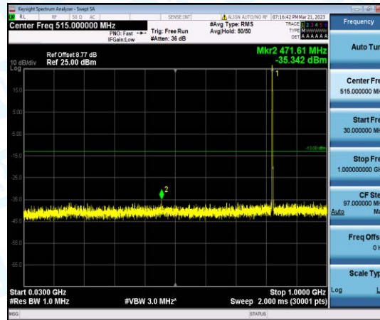
Band5-5MHz-16QAM-20425-1-0-Low-30-1000--35.34-PASS
