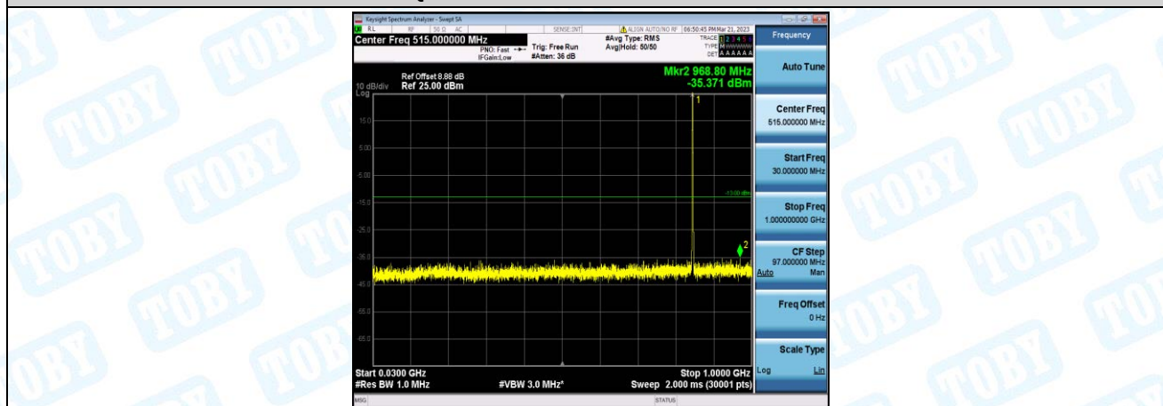
Band5-3MHz-QPSK-20635-1-0-High-30-1000--35.37-PASS
