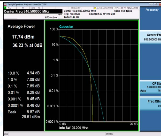
Band5-5MHz-QPSK-20625-6-0-High-7.89-<=13-PASS
