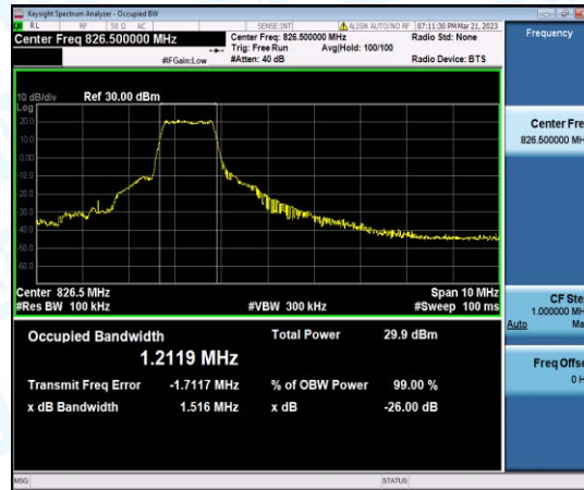
Band5-5MHz-QPSK-20425-6-0-Low-1.2119-1.516-PASS
