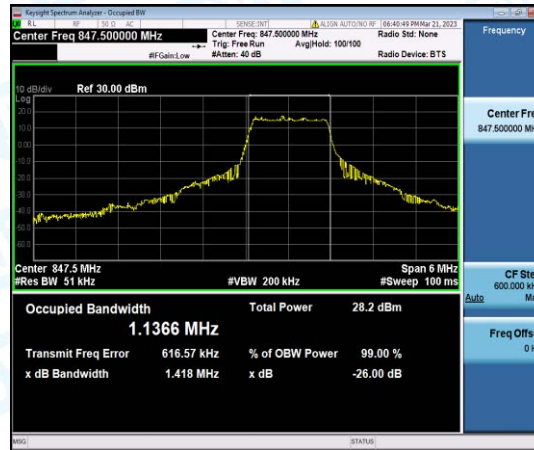
Band5-3MHz-QPSK-20635-6-0-High-1.1366-1.418-PASS
