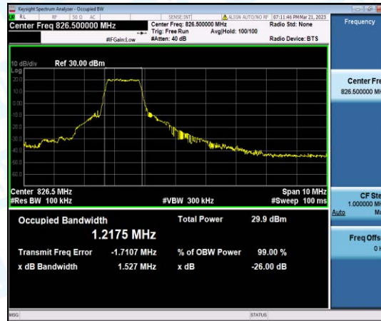
Band5-5MHz-16QAM-20425-6-0-Low-1.2175-1.527-PASS
