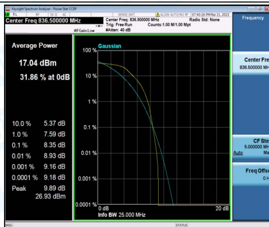
Band5-10MHz-16QAM-20525-6-0-Low-8.35-<=13-PASS
