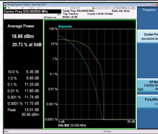
Band5-10MHz-16QAM-20450-1-0-Low-11.33-<=13-PASS
