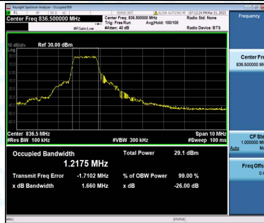
Band5-5MHz-16QAM-20525-6-0-Low-1.2175-1.660-PASS
