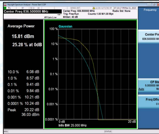
Band5-5MHz-QPSK-20525-6-0-Low-9.41-<=13-PASS
