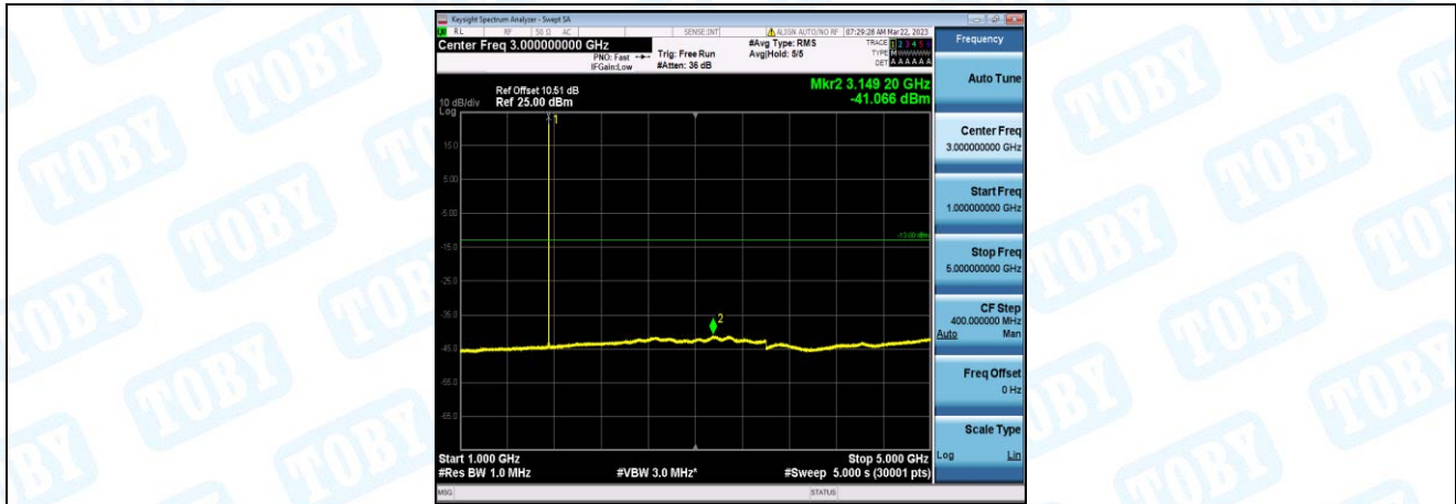
Band4-10MHz-16QAM-20350-1-0-High-1000-5000--41.07-PASS
