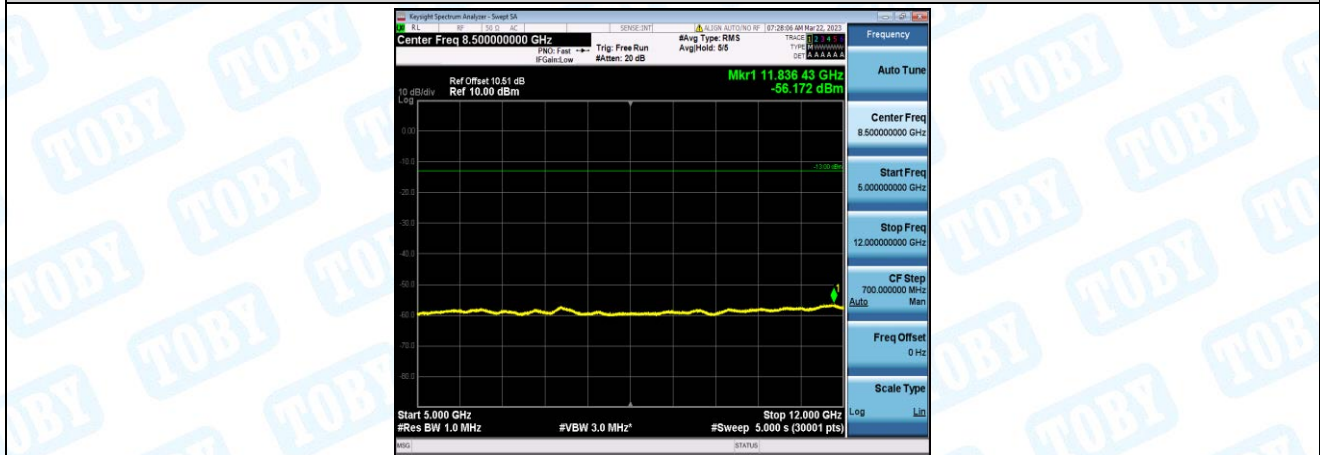
Band4-10MHz-QPSK-20350-1-0-High-5000-12000--56.17-PASS
