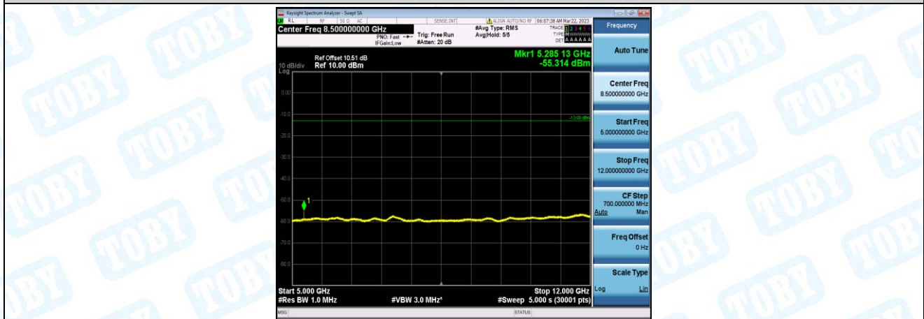
Band4-1.4MHz-QPSK-20393-1-0-High-5000-12000--55.31-PASS
