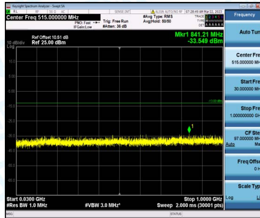
Band4-10MHz-16QAM-20350-1-0-High-30-1000--33.55-PASS
