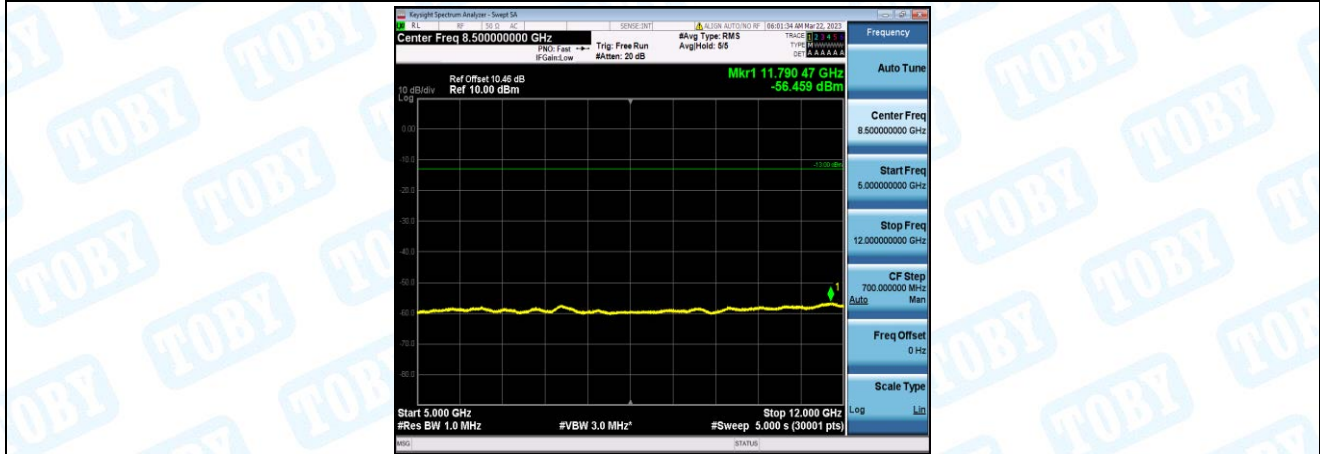
Band4-1.4MHz-16QAM-19957-1-0-Low-5000-12000--56.46-PASS
