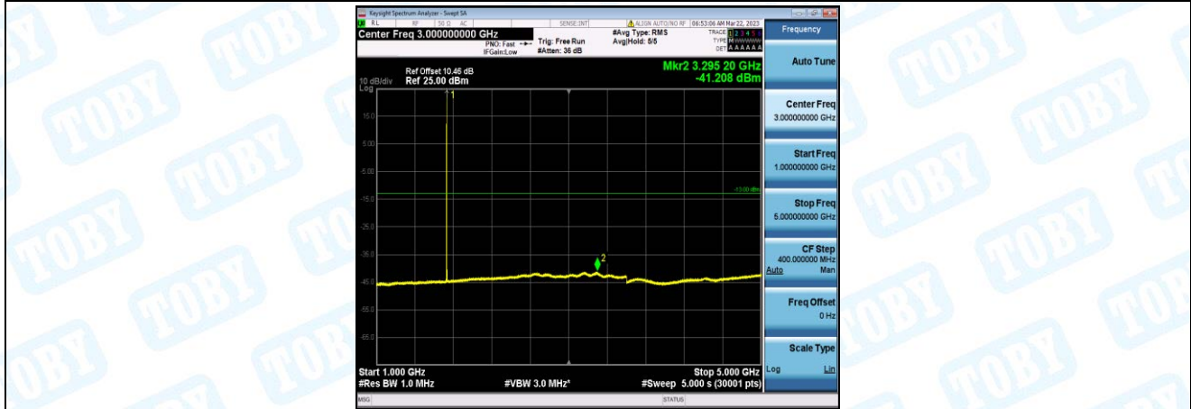
Band4-5MHz-QPSK-20175-1-0-Low-1000-5000--41.21-PASS
