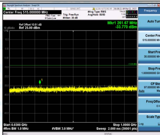
Band4-1.4MHz-16QAM-20393-1-0-High-30-1000--33.77-PASS
