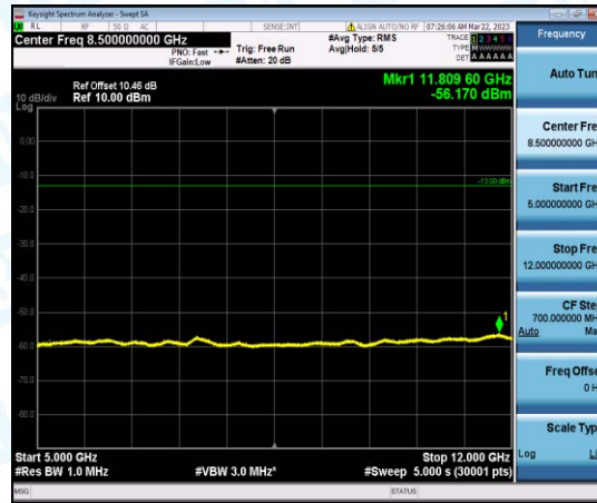
Band4-10MHz-16QAM-20175-1-0-Low-5000-12000--56.17-PASS
