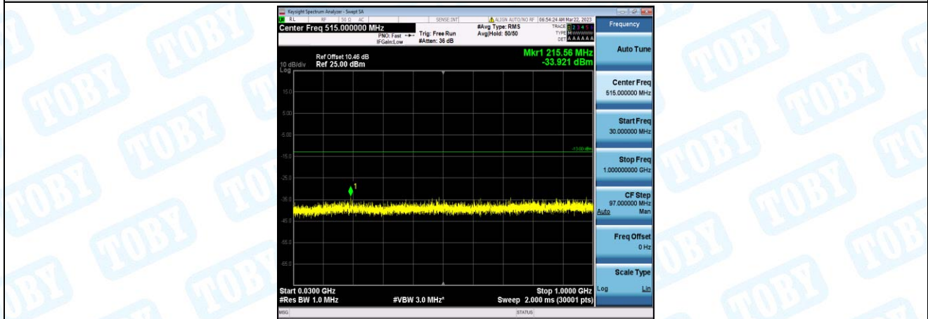
Band4-5MHz-16QAM-20175-1-0-Low-30-1000--33.92-PASS
