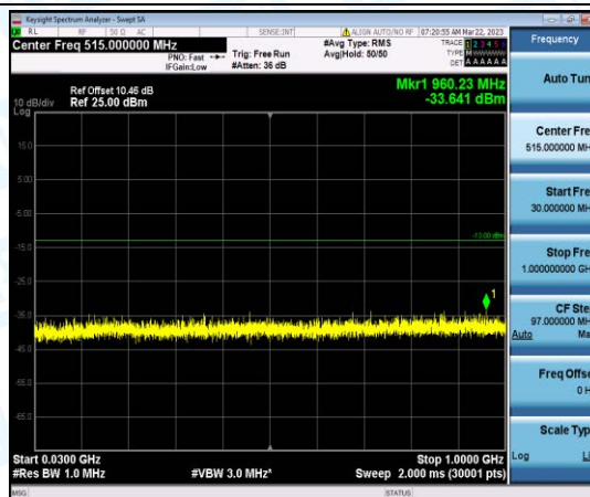
Band4-10MHz-16QAM-20000-1-0-Low-30-1000--33.64-PASS
