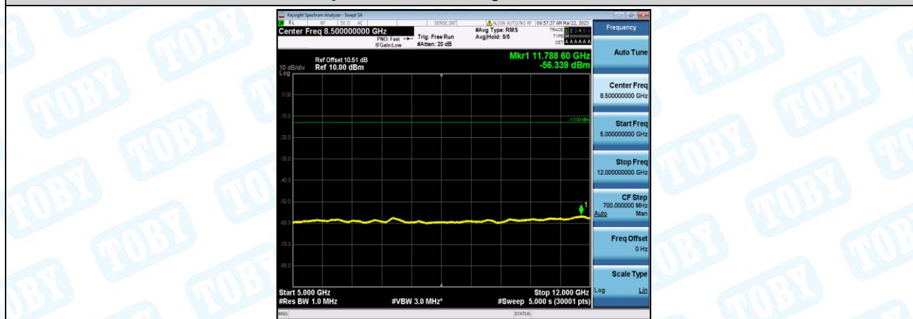
Band4-5MHz-QPSK-20375-1-0-High-5000-12000--56.34-PASS
