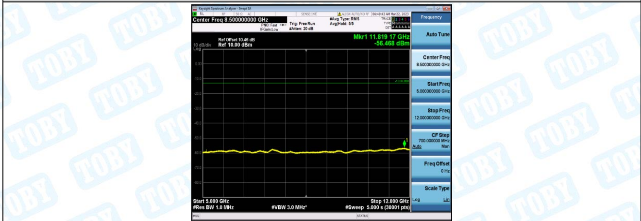
Band4-5MHz-QPSK-19975-1-0-Low-5000-12000--56.47-PASS
