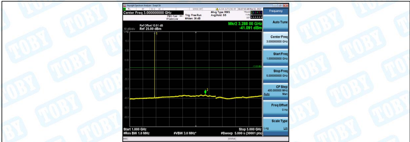
Band4-1.4MHz-QPSK-20393-1-0-High-1000-5000--41.09-PASS
