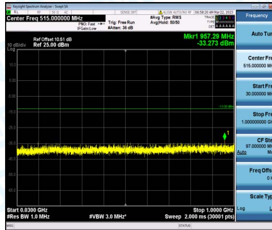
Band4-5MHz-16QAM-20375-1-0-High-30-1000--33.27-PASS
