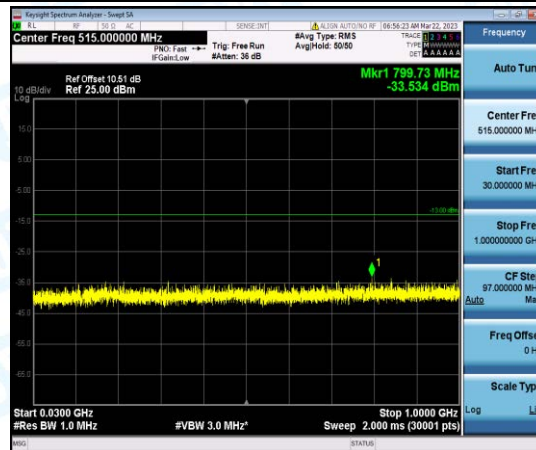
Band4-5MHz-QPSK-20375-1-0-High-30-1000--33.53-PASS
