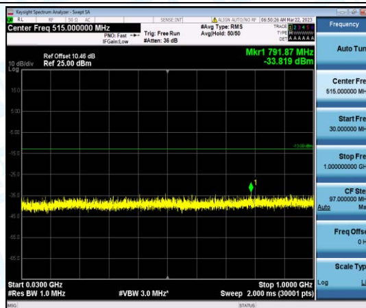
Band4-5MHz-16QAM-19975-1-0-Low-30-1000--33.82-PASS
