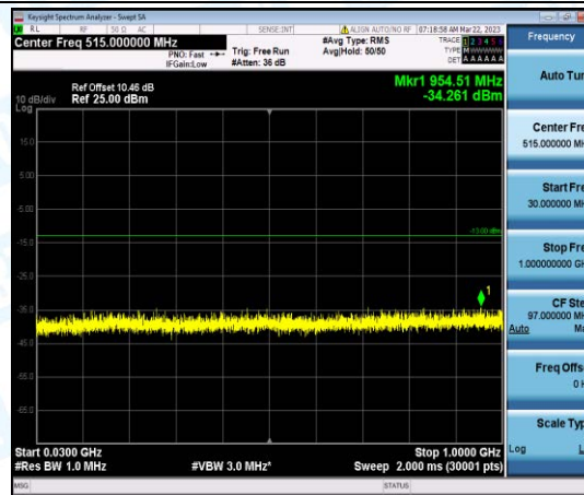
Band4-10MHz-QPSK-20000-1-0-Low-30-1000--34.26-PASS
