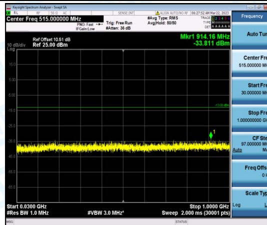
Band4-3MHz-16QAM-20385-1-0-High-30-1000--33.81-PASS
