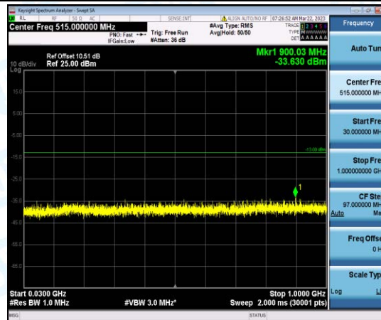
Band4-10MHz-QPSK-20350-1-0-High-30-1000--33.63-PASS
