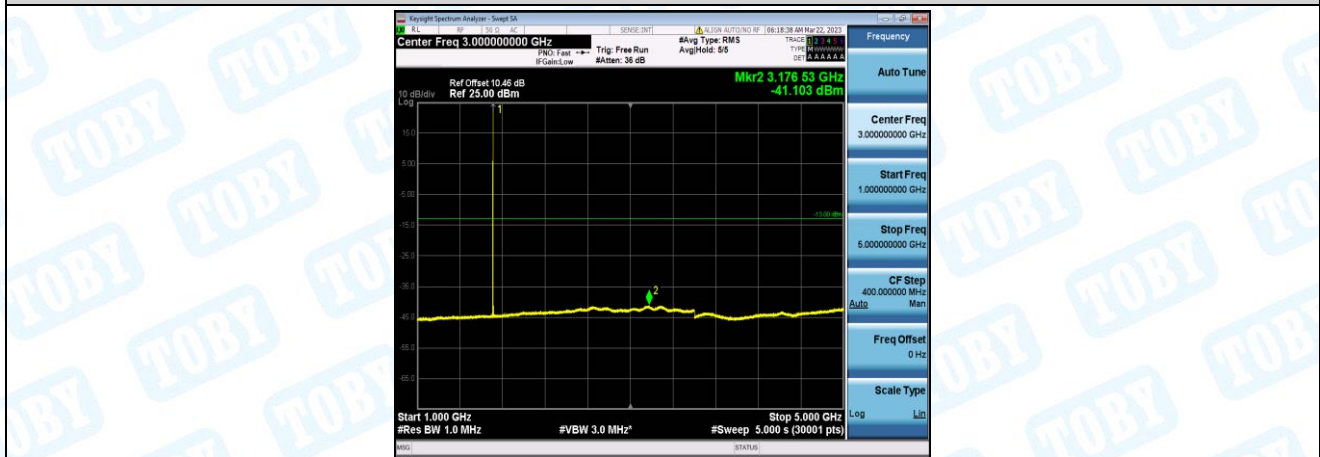
Band4-3MHz-QPSK-19965-1-0-Low-1000-5000--41.1-PASS
