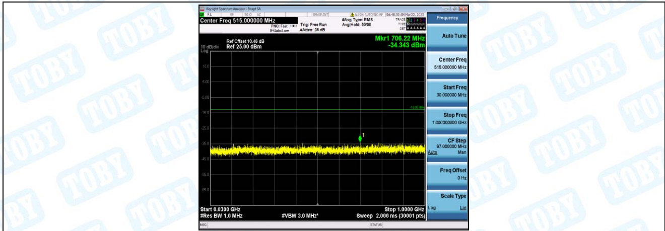
Band4-5MHz-QPSK-19975-1-0-Low-30-1000--34.34-PASS
