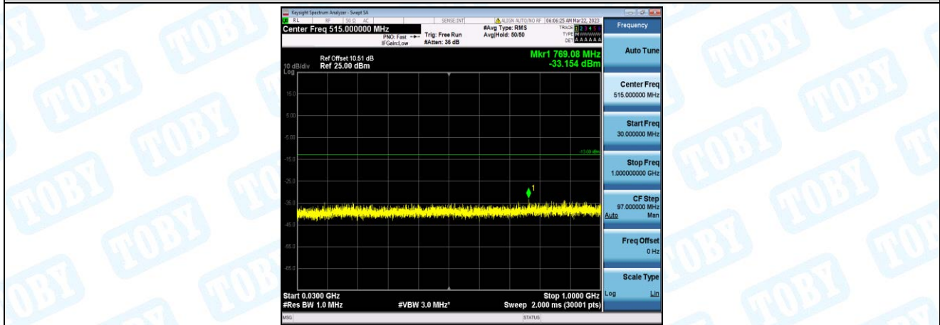
Band4-1.4MHz-QPSK-20393-1-0-High-30-1000--33.15-PASS
