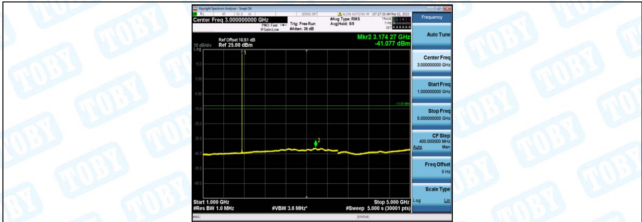
Band4-10MHz-QPSK-20350-1-0-High-1000-5000--41.08-PASS
