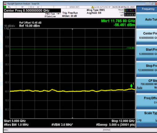
Band4-5MHz-16QAM-20175-1-0-Low-5000-12000--56.46-PASS
