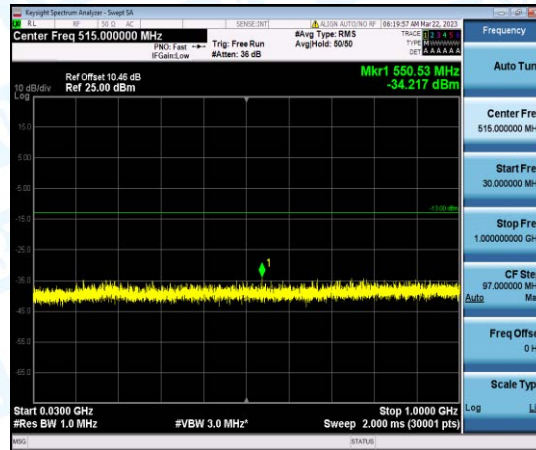
Band4-3MHz-16QAM-19965-1-0-Low-30-1000--34.22-PASS
