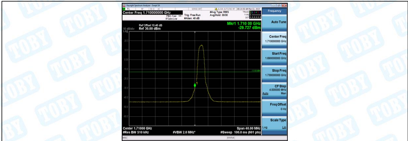
Band4-20MHz-16QAM-20050-6-0-Low--29.73-PASS
