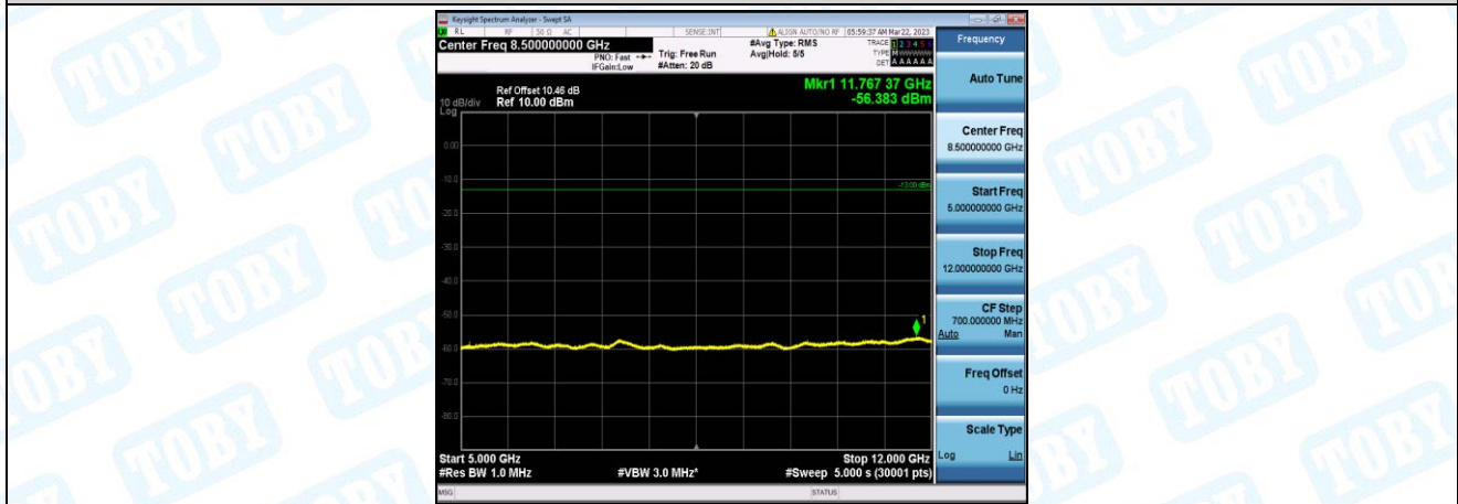
Band4-1.4MHz-QPSK-19957-1-0-Low-5000-12000--56.38-PASS
