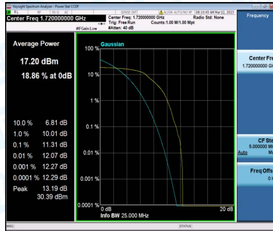
Band4-20MHz-QPSK-20050-6-0-Low-11.31-<=13-PASS
