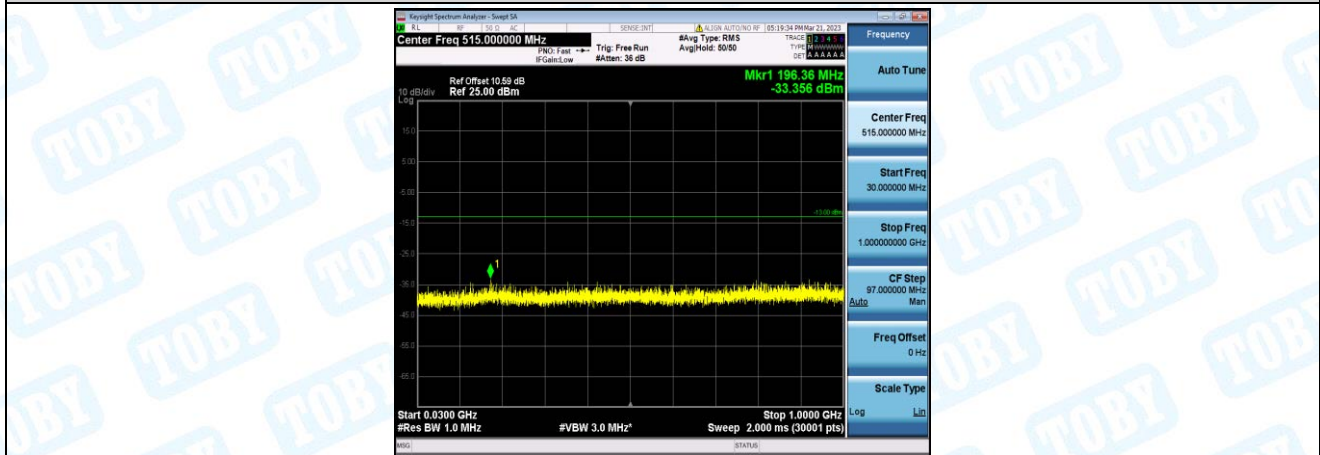
Band2-15MHz-16QAM-18900-1-0-Low-30-1000--33.36-PASS
