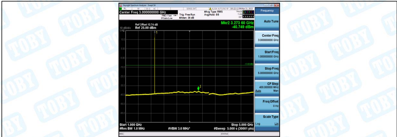
Band2-15MHz-QPSK-19150-1-0-High-1000-5000--40.75-PASS
