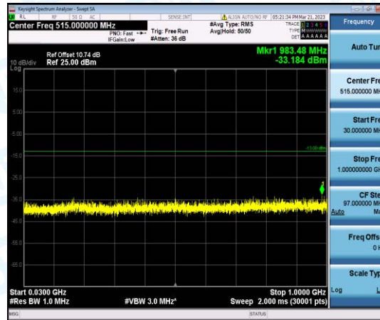
Band2-15MHz-QPSK-19150-1-0-High-30-1000--33.18-PASS
