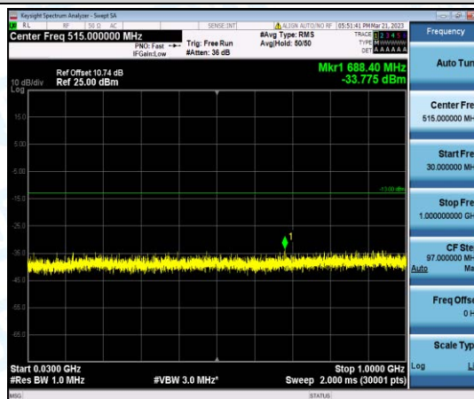
Band2-20MHz-16QAM-19100-1-0-High-30-1000--33.78-PASS
