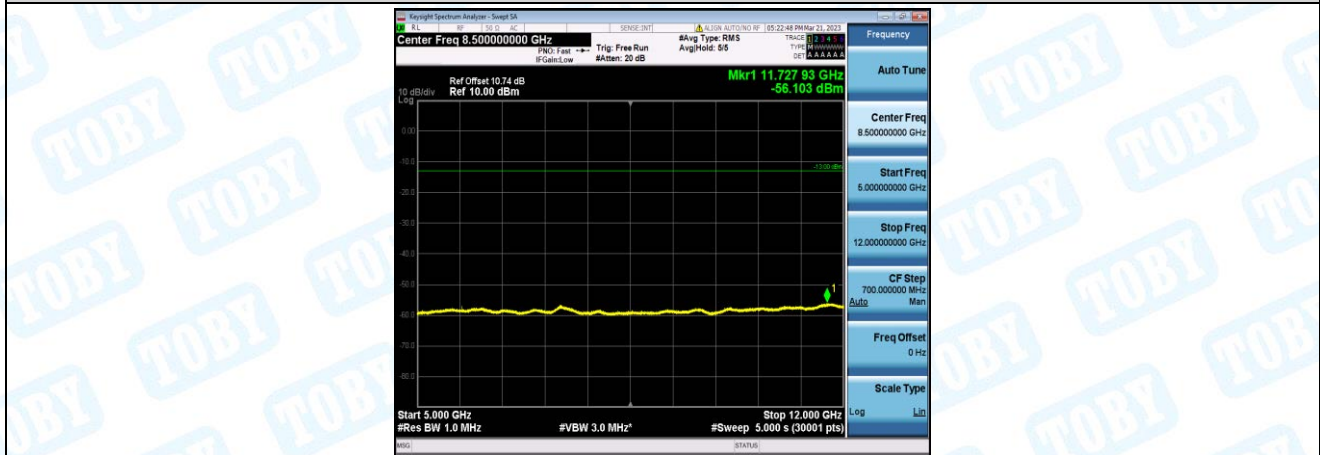
Band2-15MHz-QPSK-19150-1-0-High-5000-12000--56.1-PASS
