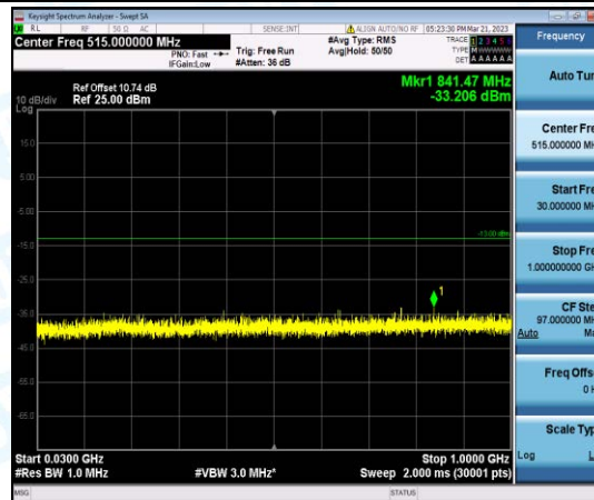
Band2-15MHz-16QAM-19150-1-0-High-30-1000--33.21-PASS
