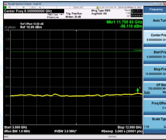
Band2-20MHz-QPSK-18900-1-0-Low-5000-12000--56.11-PASS
