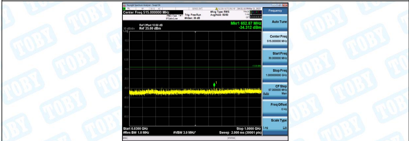
Band2-10MHz-16QAM-18900-1-0-Low-30-1000--34.31-PASS
