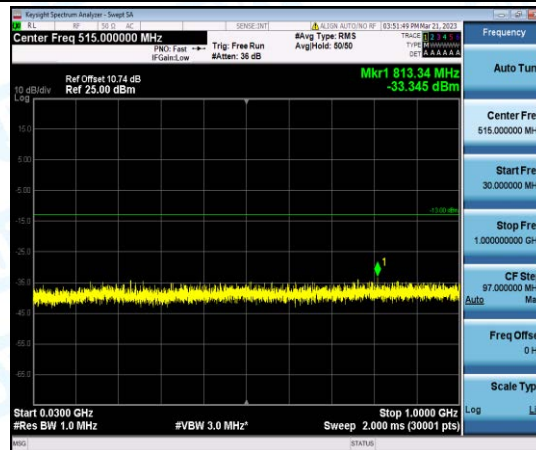
Band2-3MHz-QPSK-19185-1-0-High-30-1000--33.35-PASS
