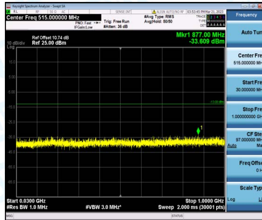
Band2-3MHz-16QAM-19185-1-0-High-30-1000--33.61-PASS
