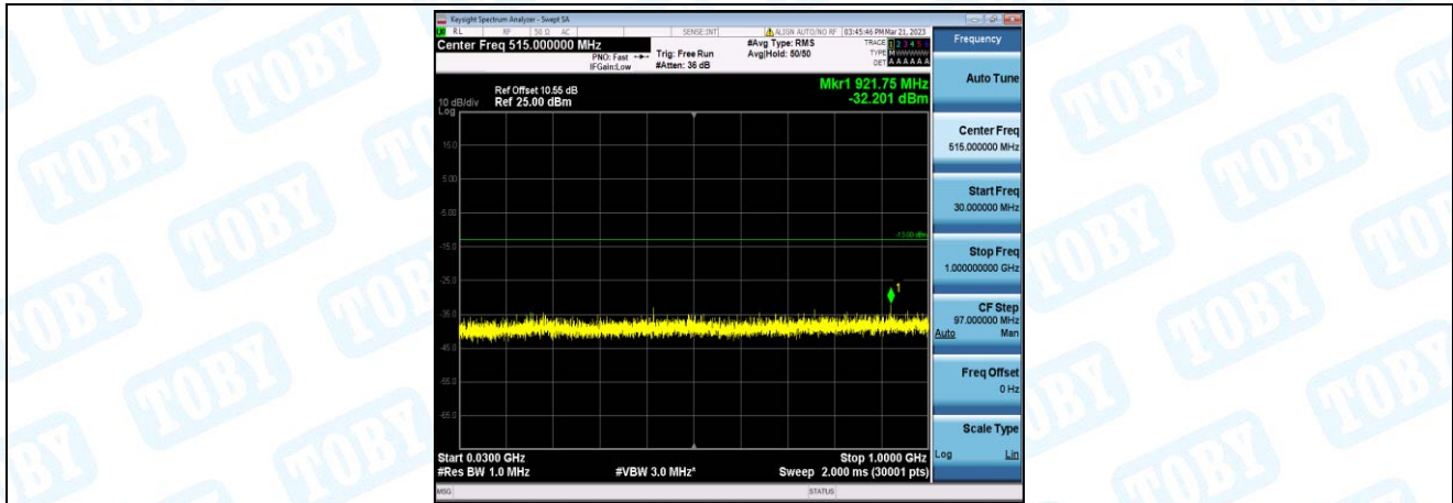
Band2-3MHz-16QAM-18615-1-0-Low-30-1000--32.2-PASS
