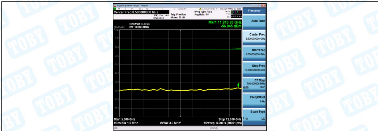
Band2-10MHz-16QAM-18900-1-0-Low-5000-12000--56.05-PASS
