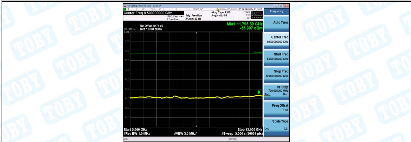
Band2-3MHz-16QAM-19185-1-0-High-5000-12000--55.99-PASS
