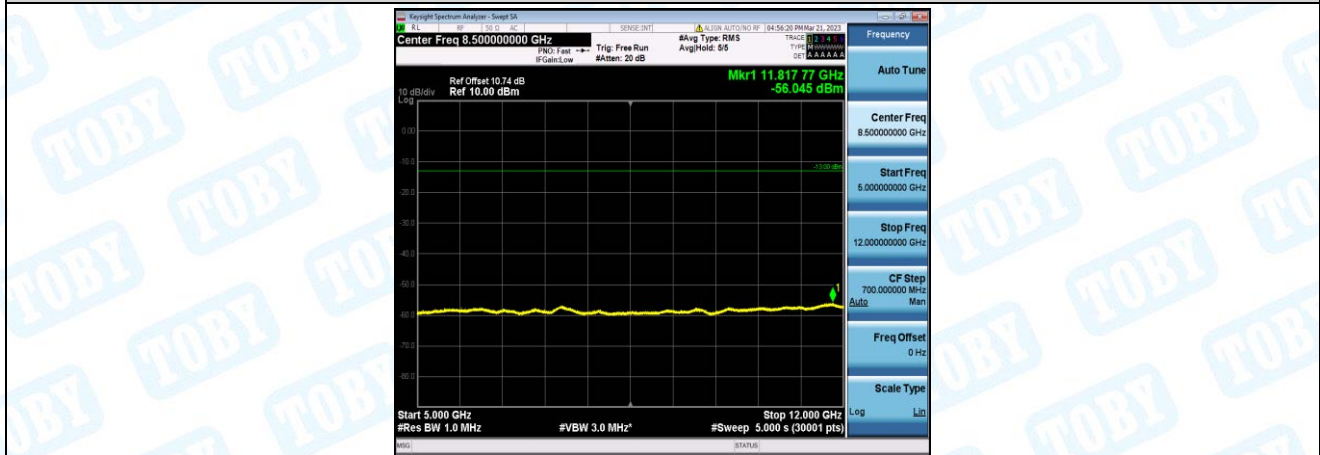
Band2-10MHz-16QAM-19150-1-0-High-5000-12000--56.05-PASS
