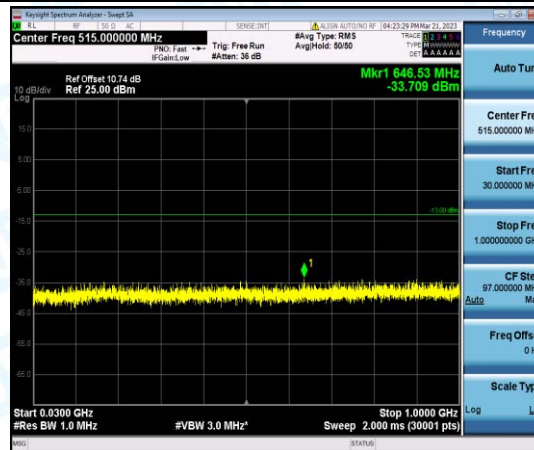
Band2-5MHz-QPSK-19175-1-0-High-30-1000--33.71-PASS
