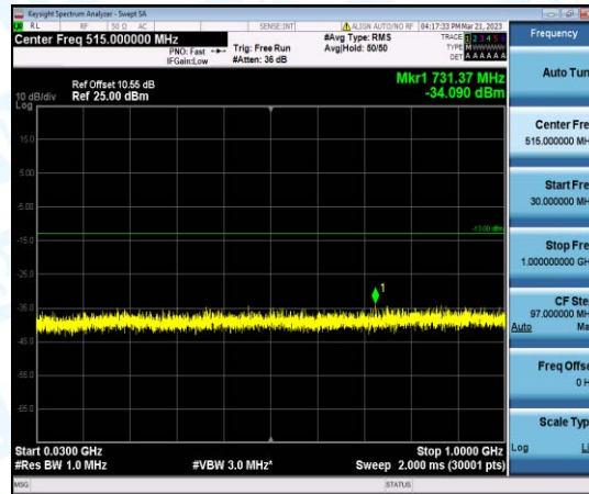
Band2-5MHz-16QAM-18625-1-0-Low-30-1000--34.09-PASS
