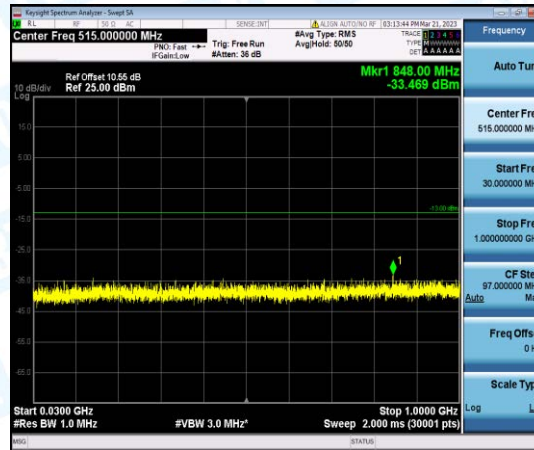
Band2-1.4MHz-16QAM-18607-1-0-Low-30-1000--33.47-PASS
