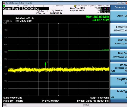
Band2-10MHz-16QAM-18650-1-0-Low-30-1000--34.04-PASS
