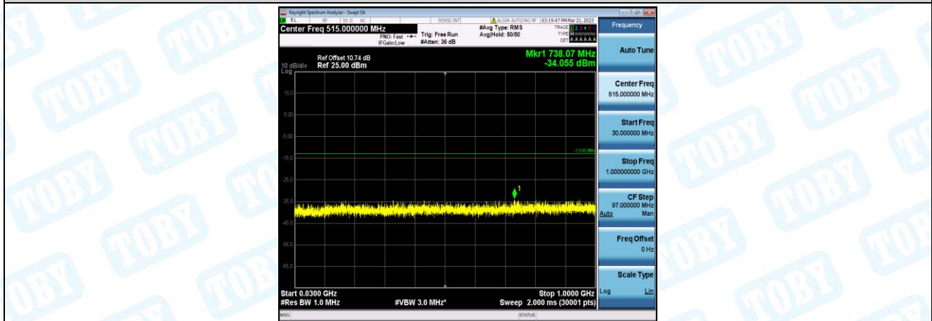
Band2-1.4MHz-QPSK-19193-1-0-High-30-1000--34.06-PASS
