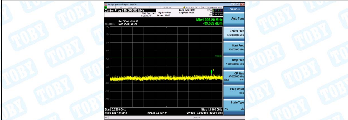
Band2-5MHz-16QAM-18900-1-0-Low-30-1000--33.59-PASS
