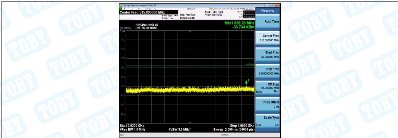
Band2-3MHz-QPSK-18615-1-0-Low-30-1000--33.73-PASS
