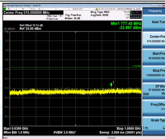
Band2-10MHz-QPSK-19150-1-0-High-30-1000--33.9-PASS
