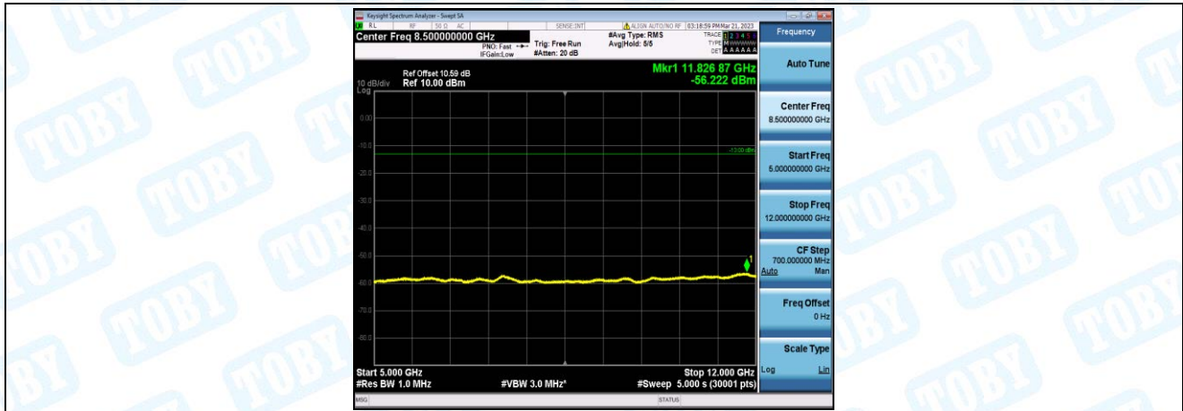
Band2-1.4MHz-16QAM-18900-1-0-Low-5000-12000--56.22-PASS
