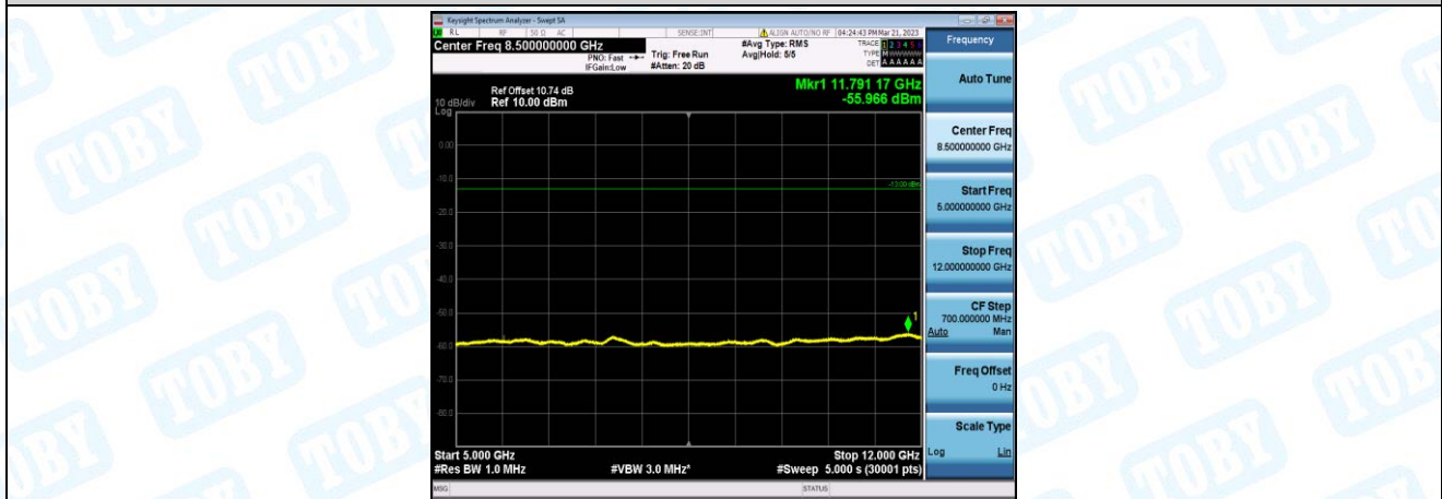
Band2-5MHz-QPSK-19175-1-0-High-5000-12000--55.97-PASS
