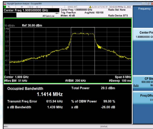
Band2-3MHz-16QAM-19185-6-0-High-1.1414-1.439-PASS
