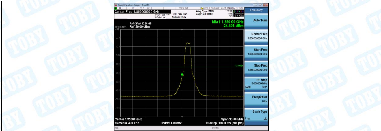
Band2-15MHz-QPSK-18675-6-0-Low--24.41-PASS
