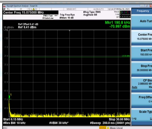
Band12-Stand-Alone-NaN-QPSK-23095-1@47-3.75kHz-0.15-30-0.15~30MHz@-71dBm--23-PASS
