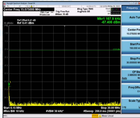
Band12-Stand-Alone-NaN-QPSK-23095-1@0-3.75kHz-0.15-30-0.15~30MHz@-67.41dBm--23-PASS
