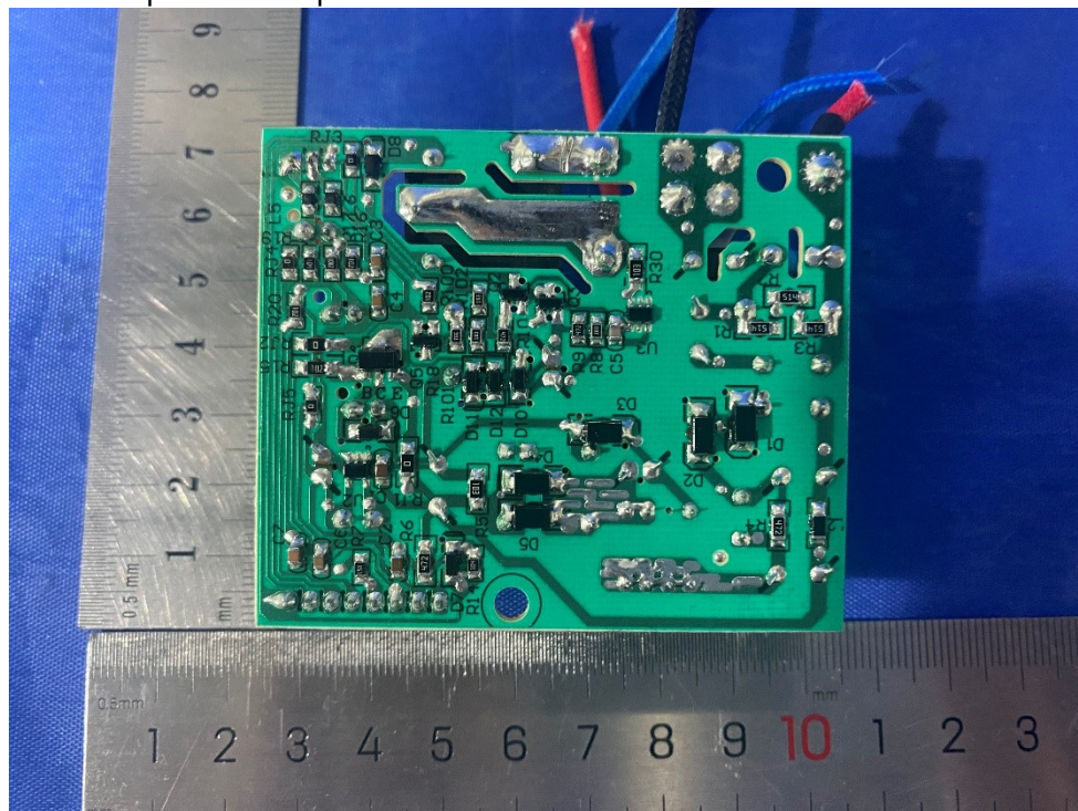
Photo 14: power board part-2
