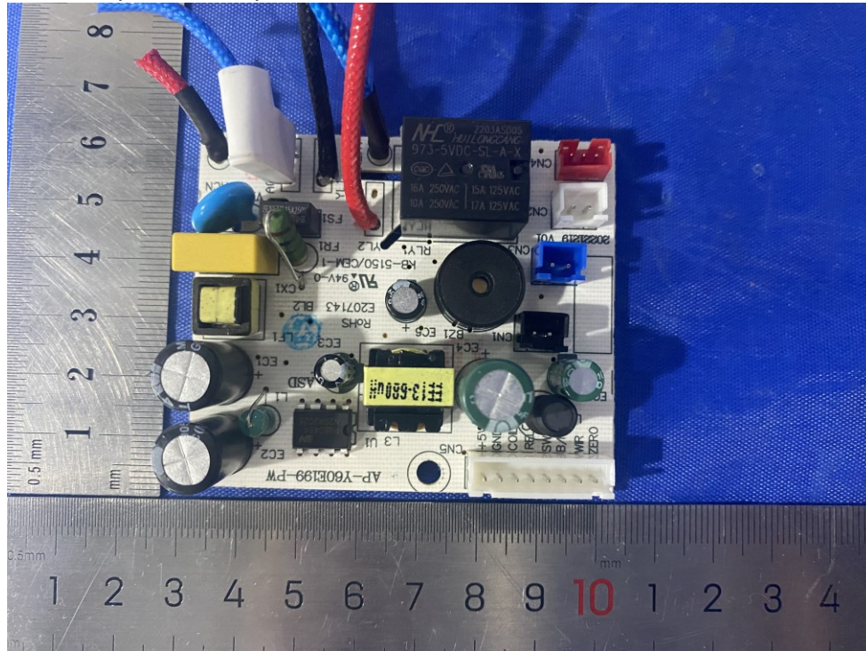
Photo 13: power board part-1
