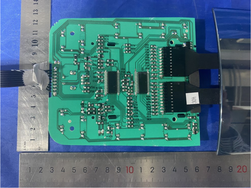
Photo 15: display board part-2
