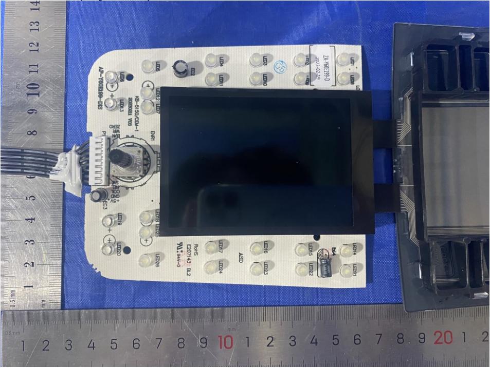
Photo 14:display board part-1
