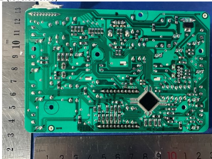
Photo 6 control board (reverse side)
