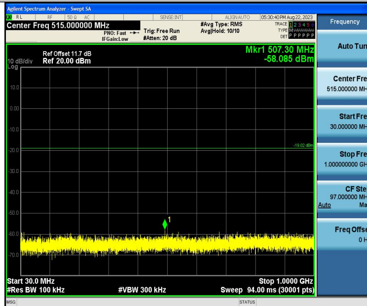
BLE_1M-Ant1-2480-30~1000-PASS
