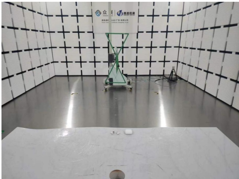
Radiated Emissions
