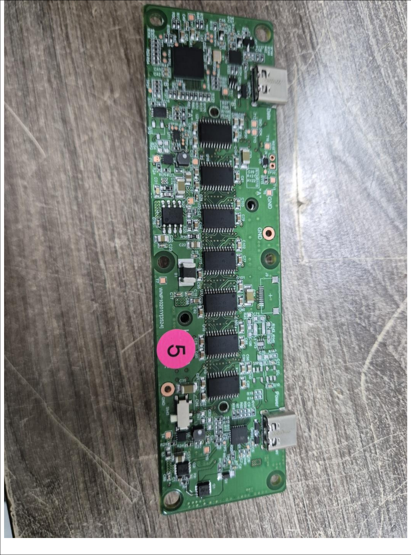
Main Board Front
