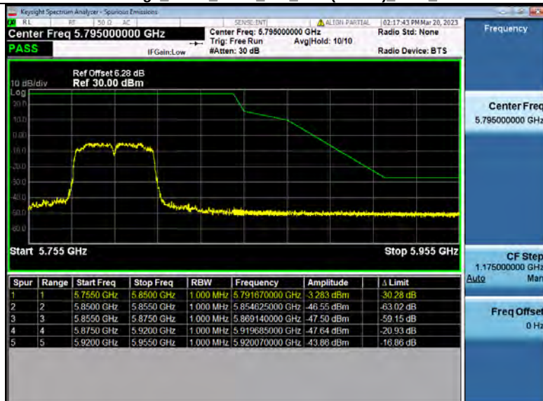
Bandedge_NVNT_ANT2_802_11ac(VHT40) 5795_40M
