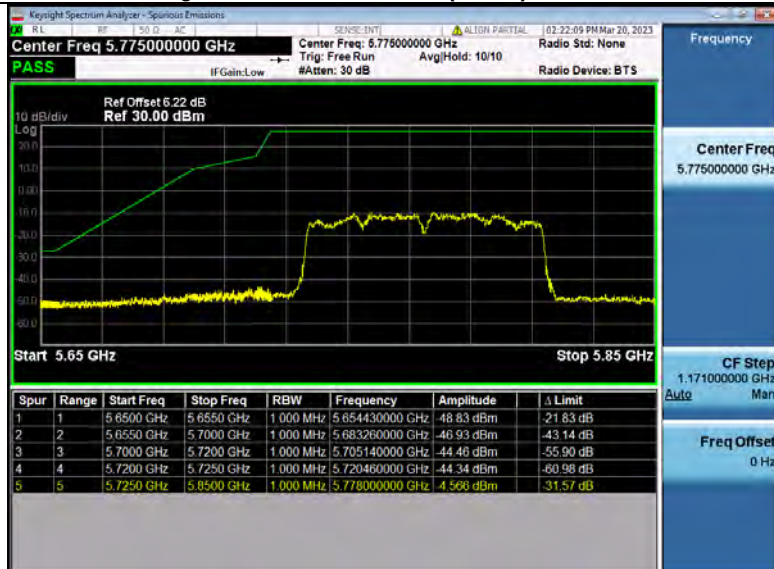
Bandedge_NVNT_ANT2_802_11ac(VHT80) 5775_80M_low
