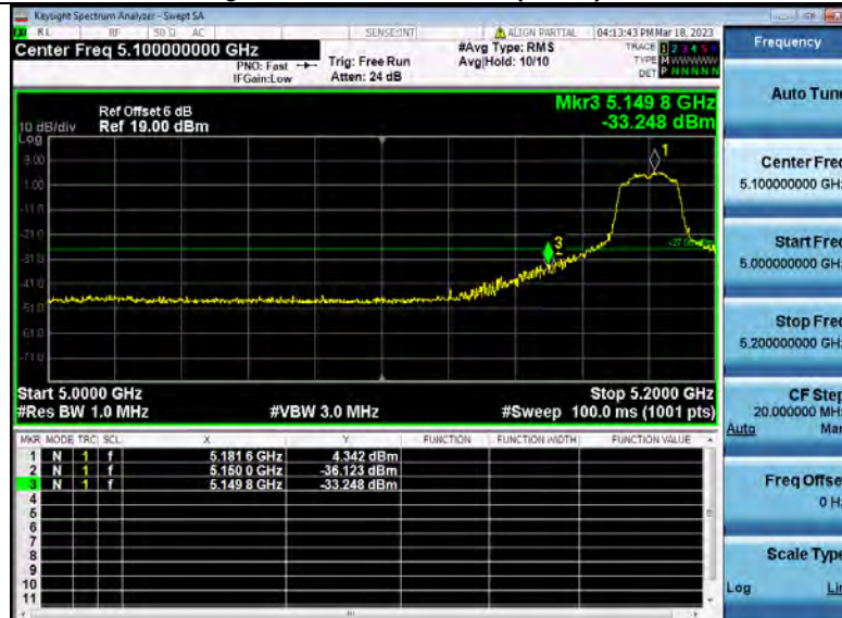
Bandedge_NVNT_ANT1_802_11ac(VHT20)_5180_20M
