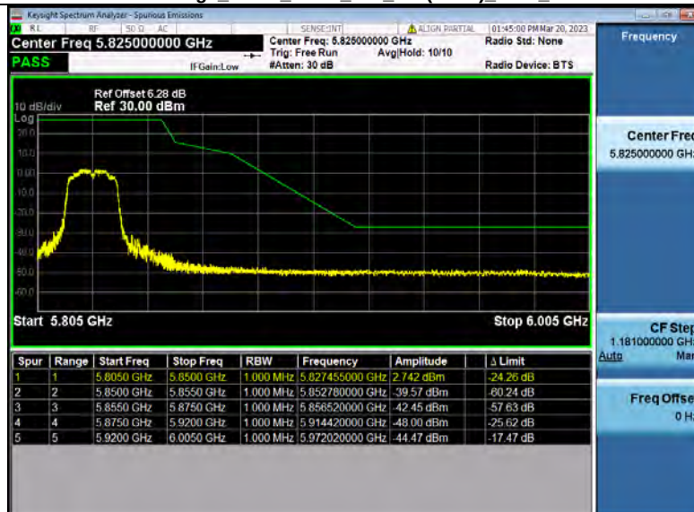
Bandedge_NVNT_ANT2_802_11n(HT20)_5825_20M
