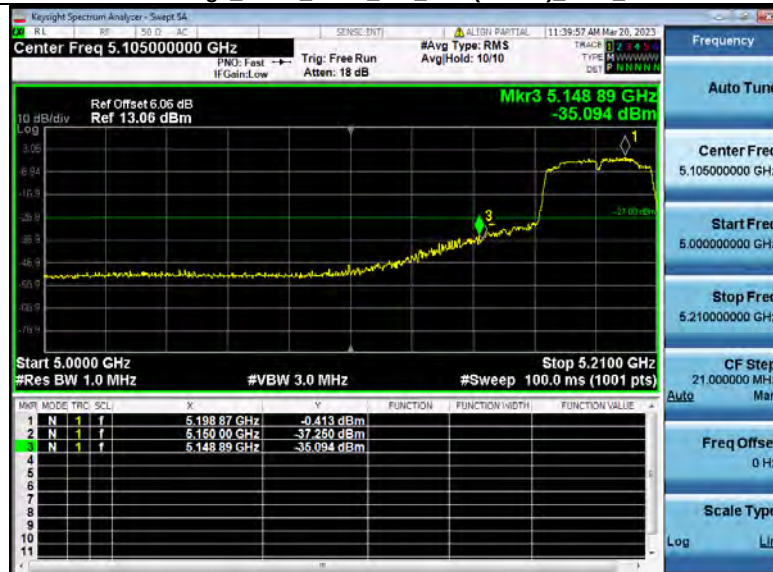
Bandedge_NVNT_ANT2_802_11ac(VHT40) 5190_40M
