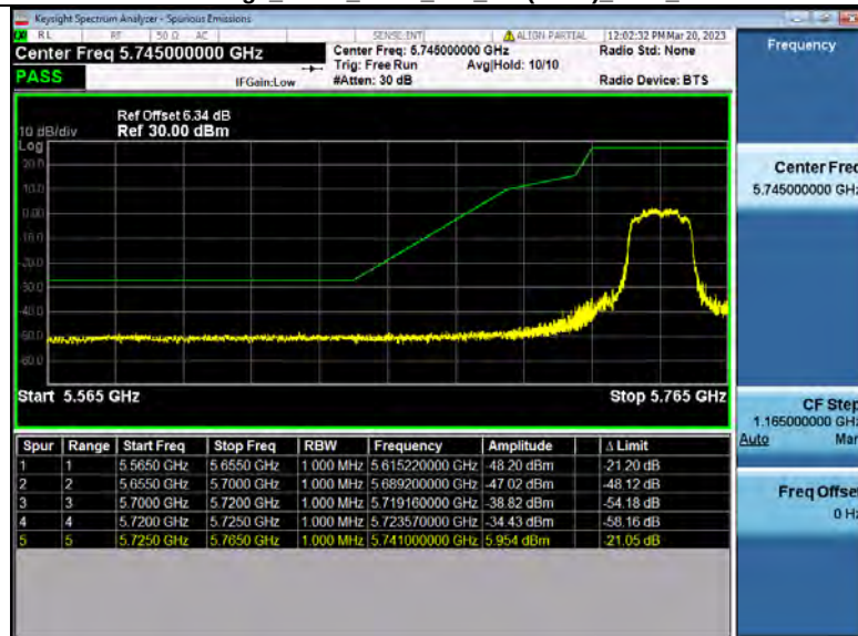
Bandedge_NVNT_ANT2_802_11n(HT20)_5745_20M
