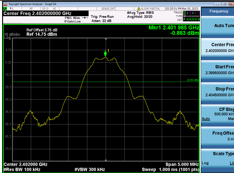
2 Bandedge NVNT_ANT1_1Mbps_2402
