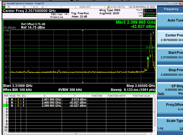
2 Bandedge NVNT_ANT1_1Mbps_2402
