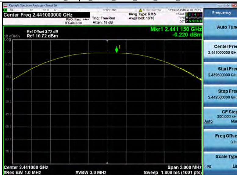
Peak Output Power_NVNT_ANT1_1-DH5_2441
