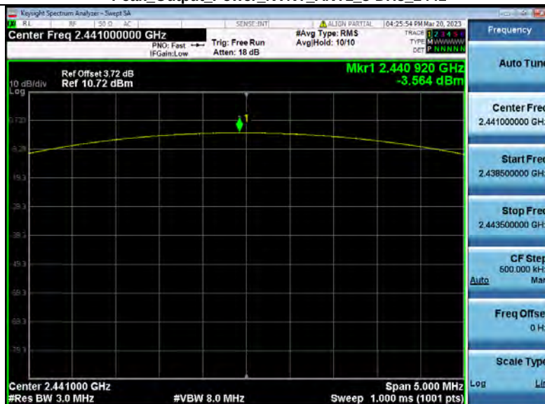
Peak_Output_Power_NVNT_ANT1_3-DH5_2441
