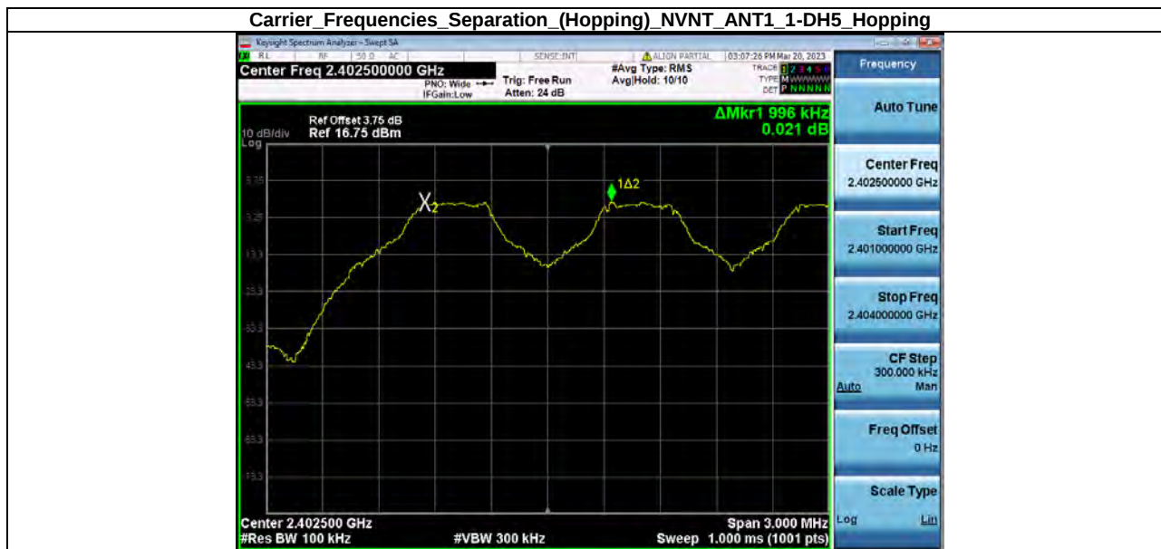
Carrier_Frequencies_Separation_(Hopping)_NVNT_ANT1_1-DH5_Hopping
