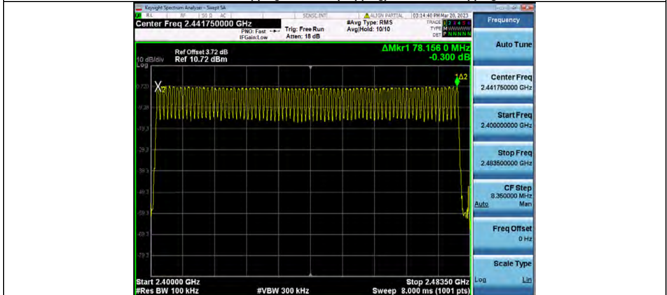
Number_of_Hopping_Channel_(Hopping)_BT_1-DH5_Hopping
