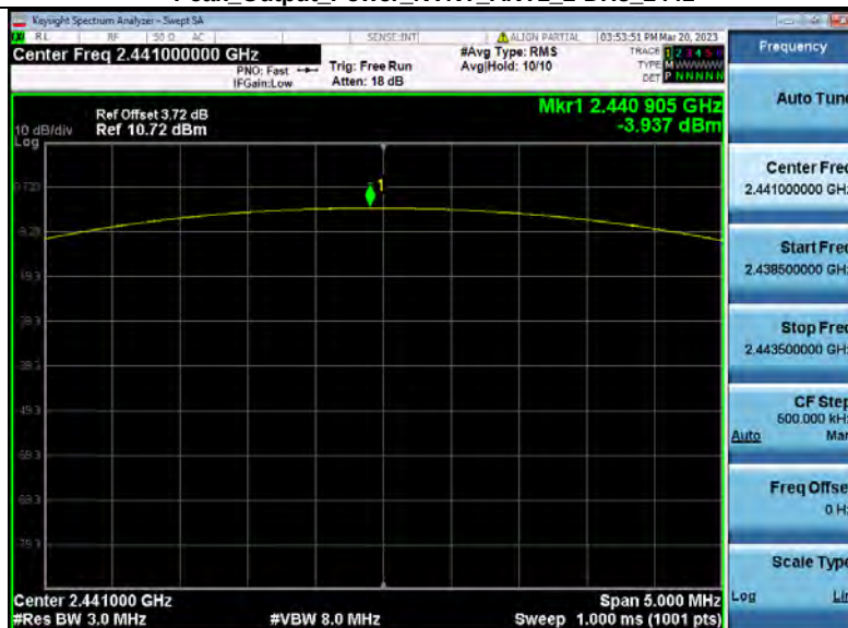
Peak_Output_Power_NVNT_ANT1_2-DH5_2441
