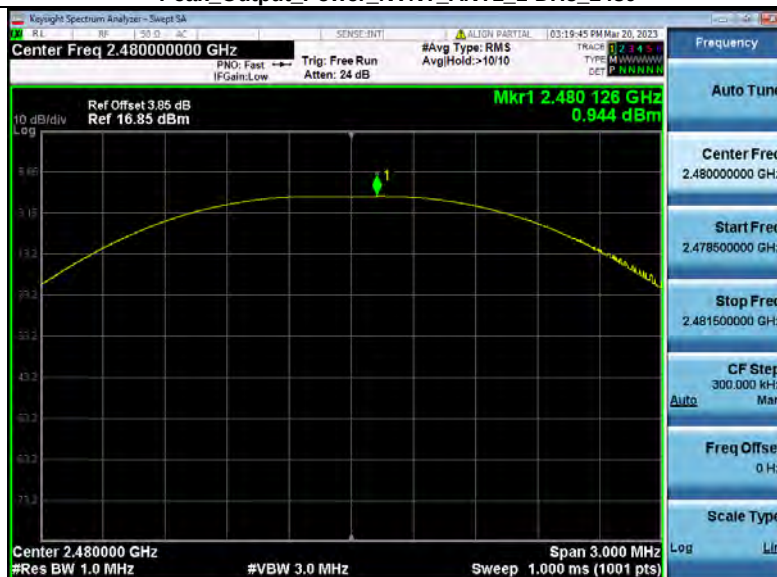
Peak_Output_Power_NVNT_ANT1_1-DH5_2480
