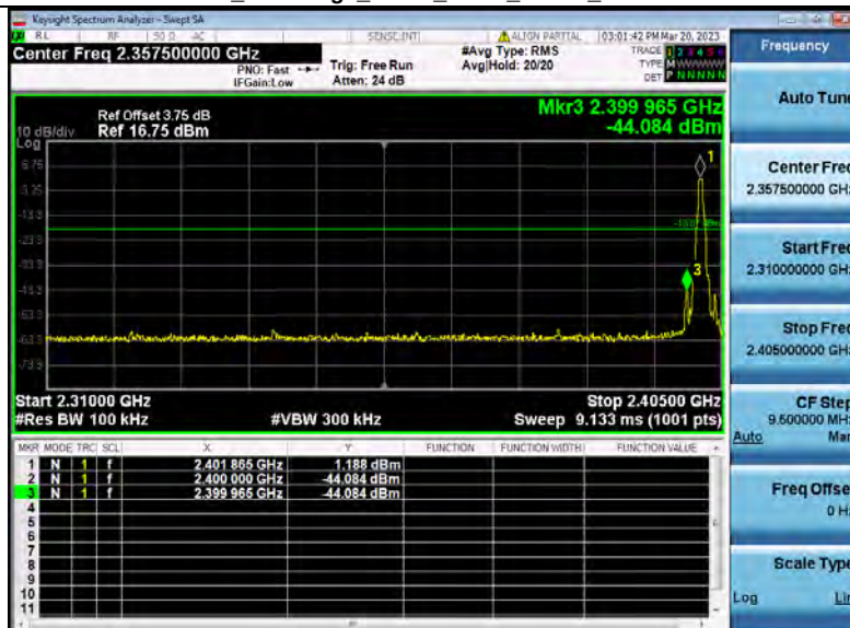
2 Bandedge_NVNT_ANT1_1-DH5_2402
