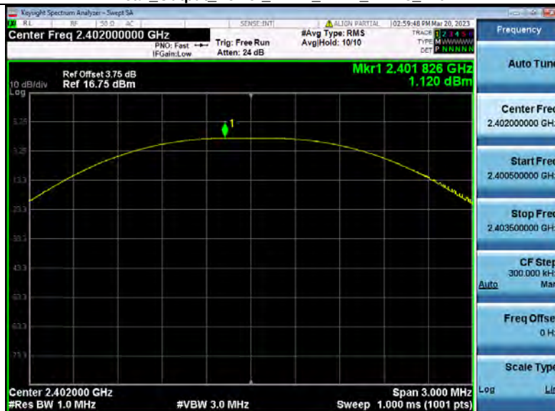
Peak Output Power_NVNT_ANT1_1-DH5_2402
