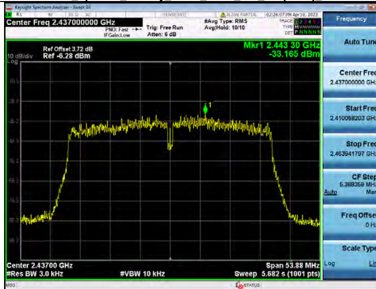
Power Spectral Density NVNT_ANT1_802_11n(HT40)_2437
