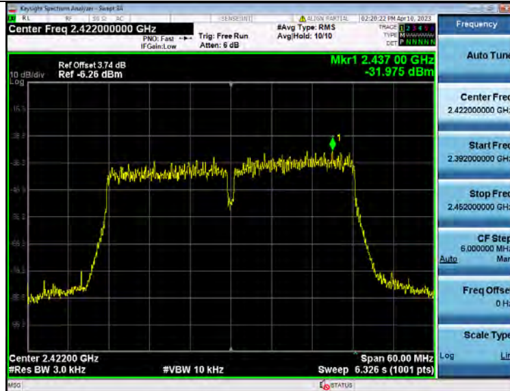
Power Spectral Density NVNT_ANT1_802_11n(HT40)_2422
