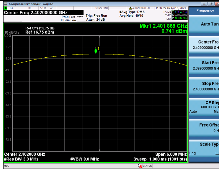
Peak_Output_Power_NVNT_ANT1_1Mbps_2402
