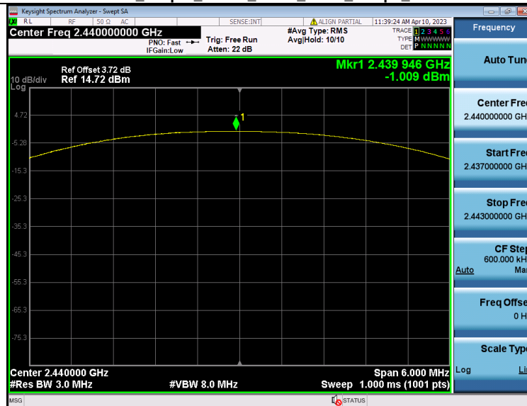
Peak_Output_Power_NVNT_ANT1_1Mbps_2440
