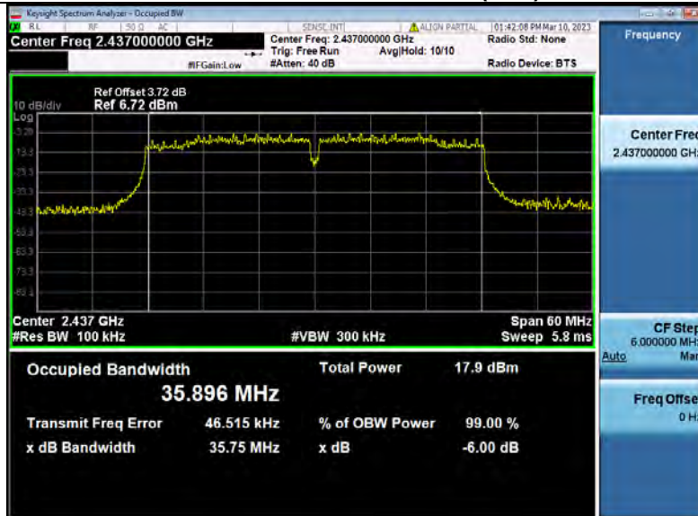
-6dB_Bandwidth_NVNT_ANT1_802_11n(HT40)_2437
