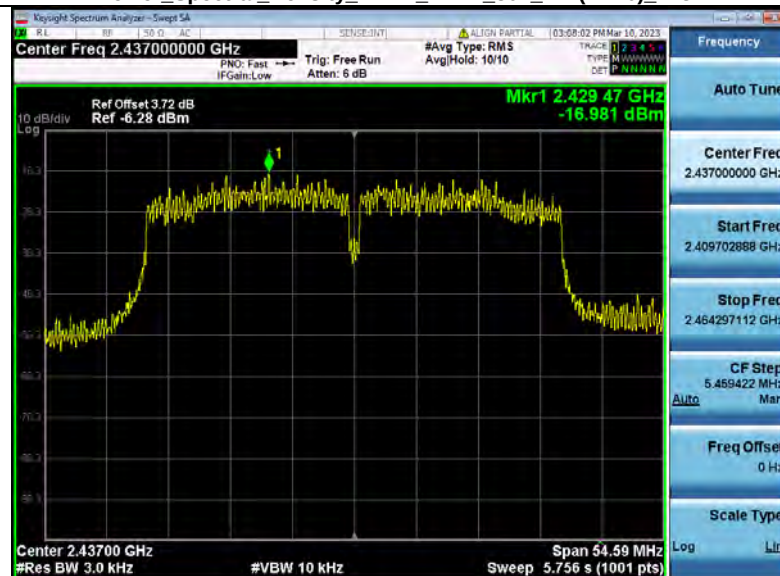
Power_Spectral_Density_NVNT_ANT2_802_11n(HT40)_2437
