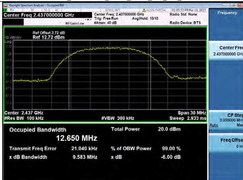
-6dB_Bandwidth_NVNT_ANT1_802_11b_2437
