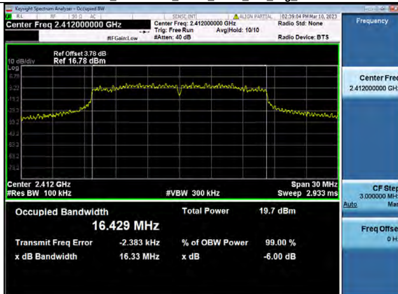
-6dB_Bandwidth_NVNT_ANT2_802_11g_2412
