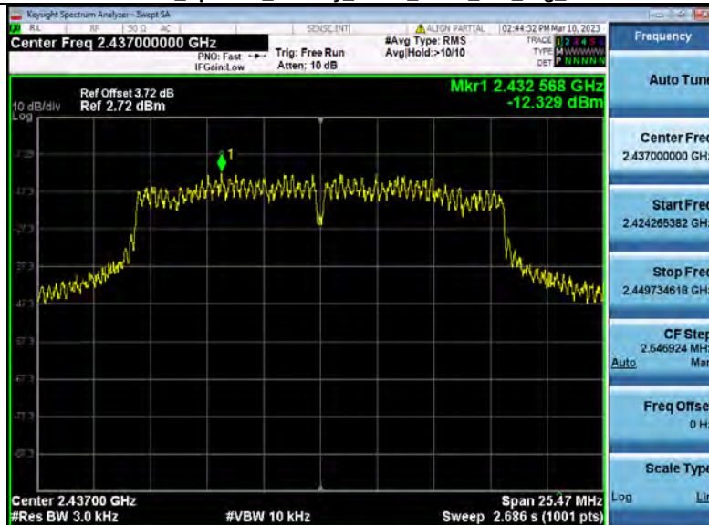
Power_Spectral_Density_NVNT_ANT2_802_11g_2437
