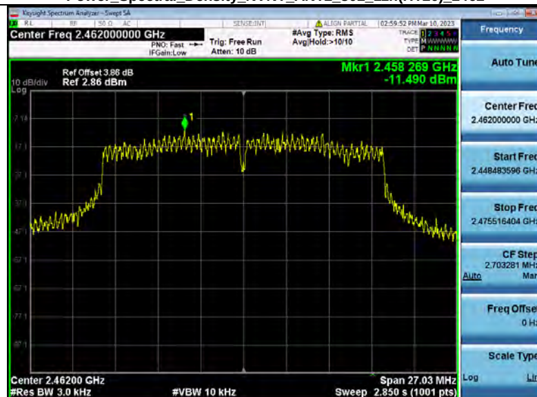
Power_Spectral_Density_NVNT_ANT2_802_11n(HT20)_2462
