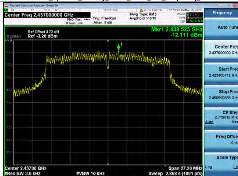
Power_Spectral_Density_NVNT_ANT2_802_11n(HT20)_2437
