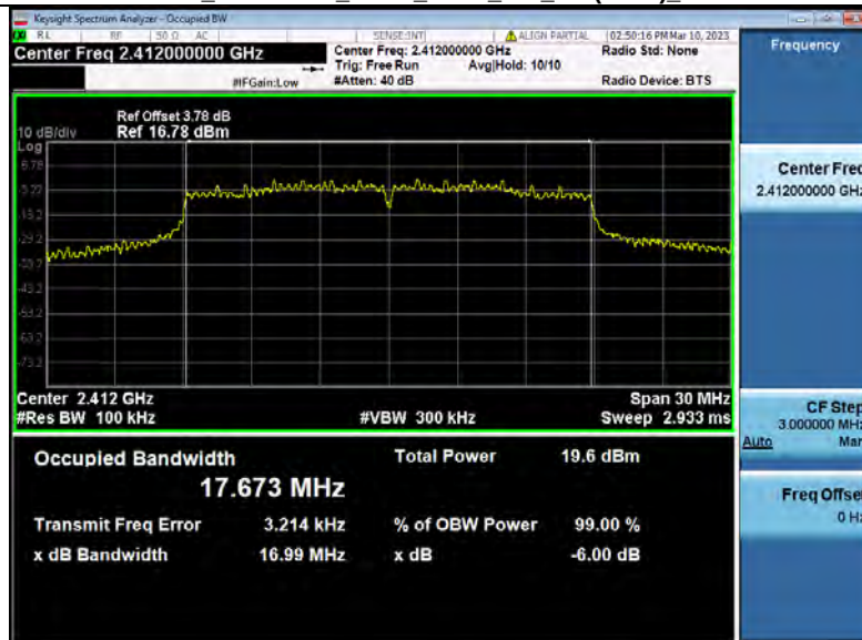
-6dB_Bandwidth_NVNT_ANT2_802_11n(HT20)_2412
