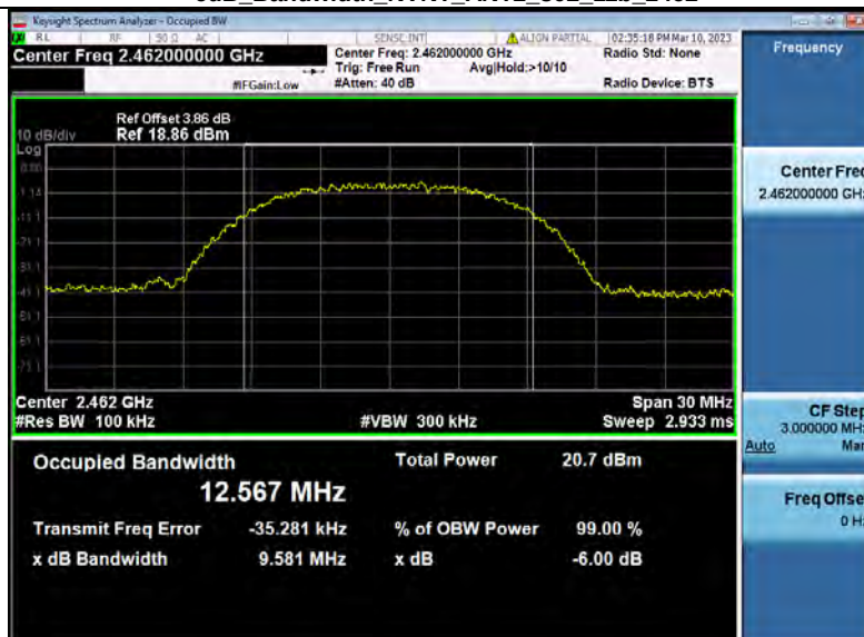
-6dB_Bandwidth_NVNT_ANT2_802_11b_2462
