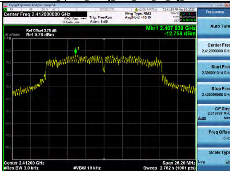
Power_Spectral_Density_NVNT_ANT2_802_11g_2412
