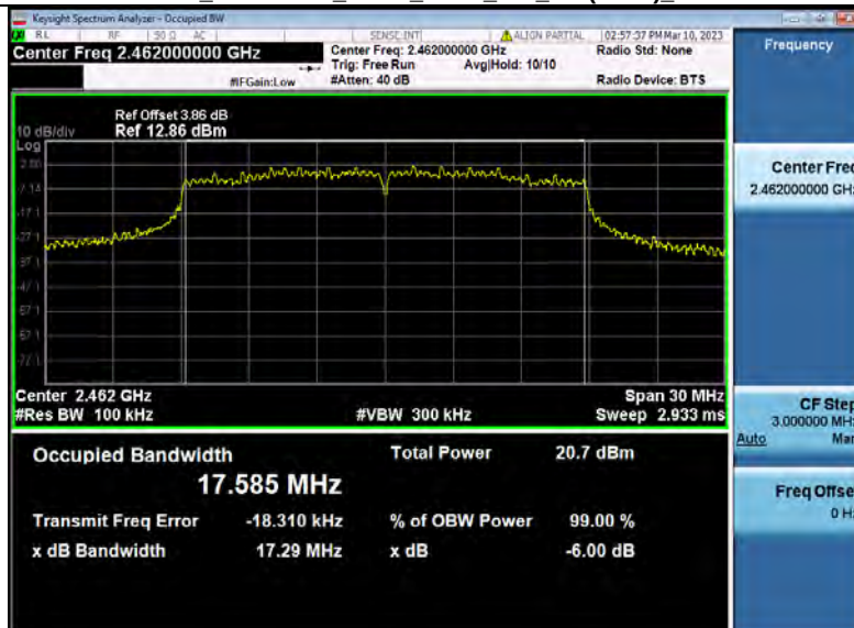
-6dB_Bandwidth_NVNT_ANT2_802_11n(HT20)_2462
