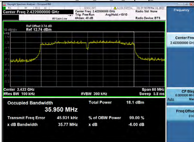
-6dB_Bandwidth_NVNT_ANT1_802_11n(HT40)_2422
