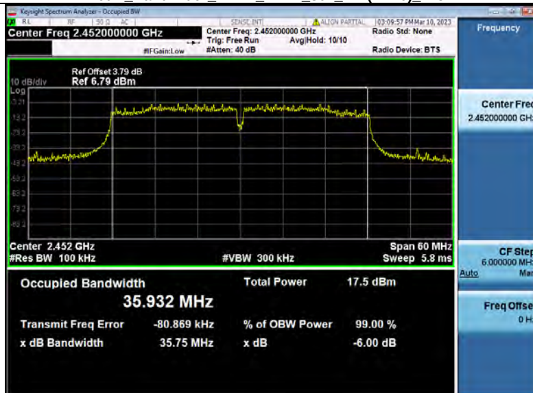
-6dB_Bandwidth_NVNT_ANT2_802_11n(HT40)_2452
