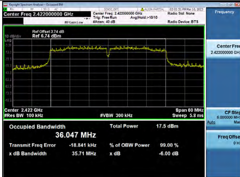
-6dB_Bandwidth_NVNT_ANT2_802_11n(HT40)_2422
