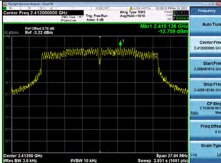
Power_Spectral_Density_NVNT_ANT1_802_11n(HT20)_2412
