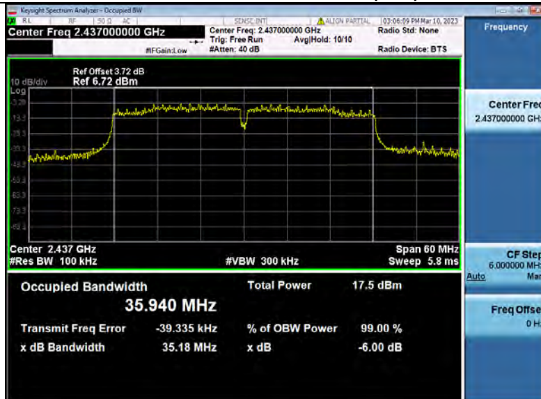
-6dB_Bandwidth_NVNT_ANT2_802_11n(HT40)_2437
