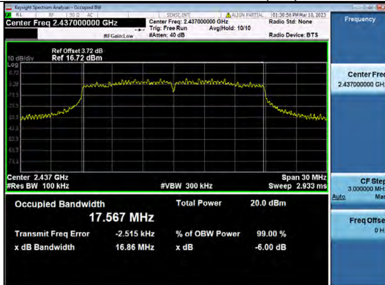
-6dB_Bandwidth_NVNT_ANT1_802_11n(HT20)_2437
