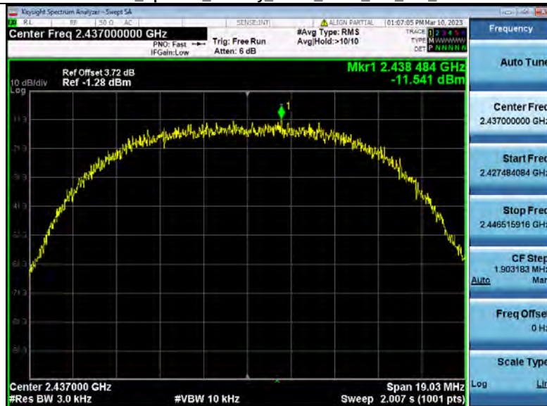
Power_Spectral_Density_NVNT_ANT1_802_11b_2437
