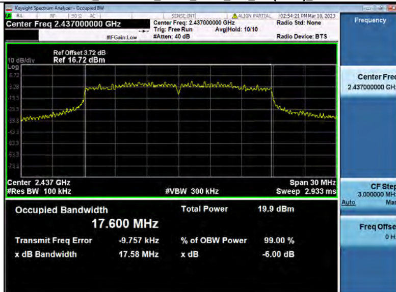
-6dB_Bandwidth_NVNT_ANT2_802_11n(HT20)_2437
