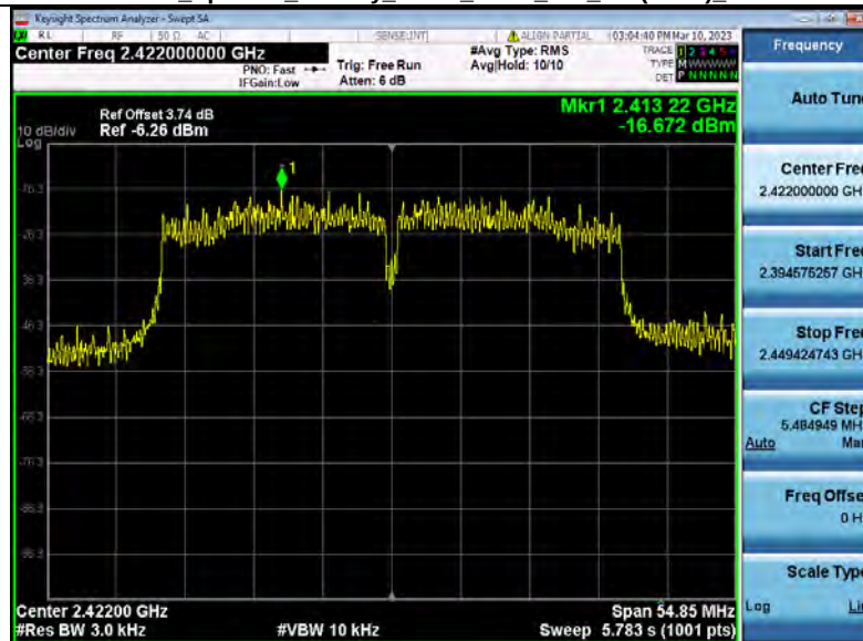
Power_Spectral_Density_NVNT_ANT2_802_11n(HT40)_2422
