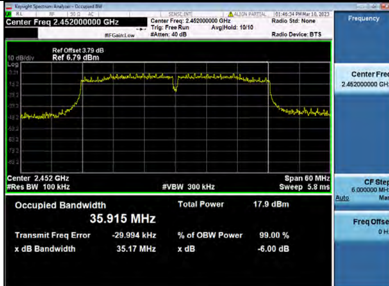
-6dB_Bandwidth_NVNT_ANT1_802_11n(HT40)_2452
