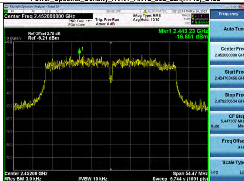
Power_Spectral_Density_NVNT_ANT2_802_11n(HT40)_2452
