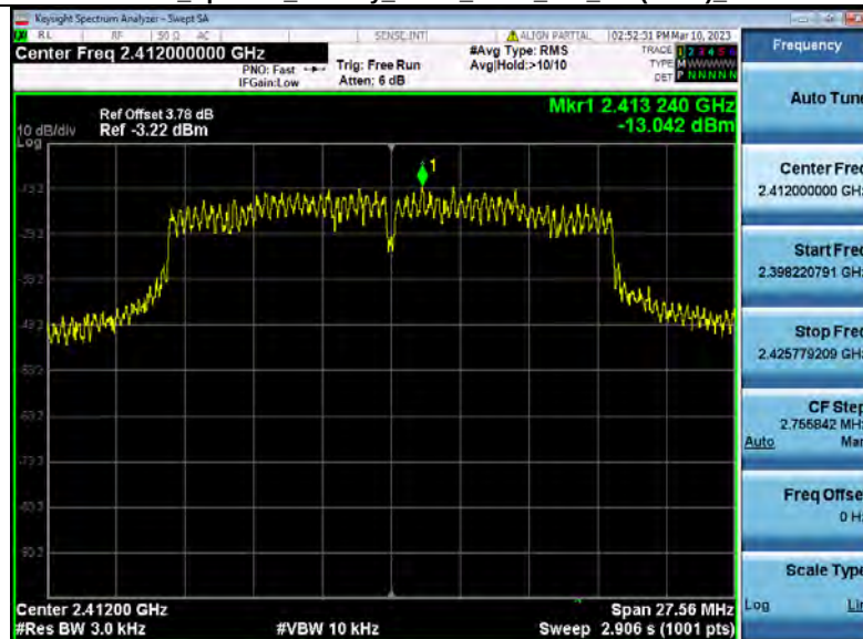
Power_Spectral_Density_NVNT_ANT2_802_11n(HT20)_2412
