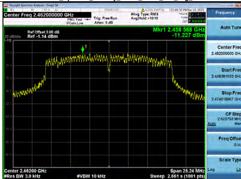
Power_Spectral_Density_NVNT_ANT2_802_11g_2462
