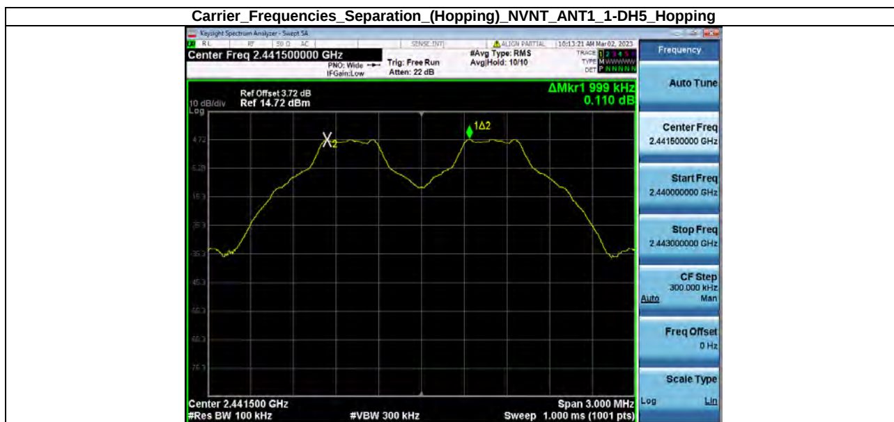
Carrier_Frequencies_Separation_(Hopping)_NVNT_ANT1_1-DH5_Hopping
