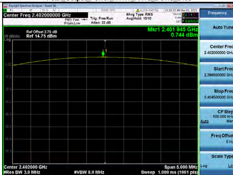
Peak_Output_Power_NVNT_ANT1_2-DH5_2402
