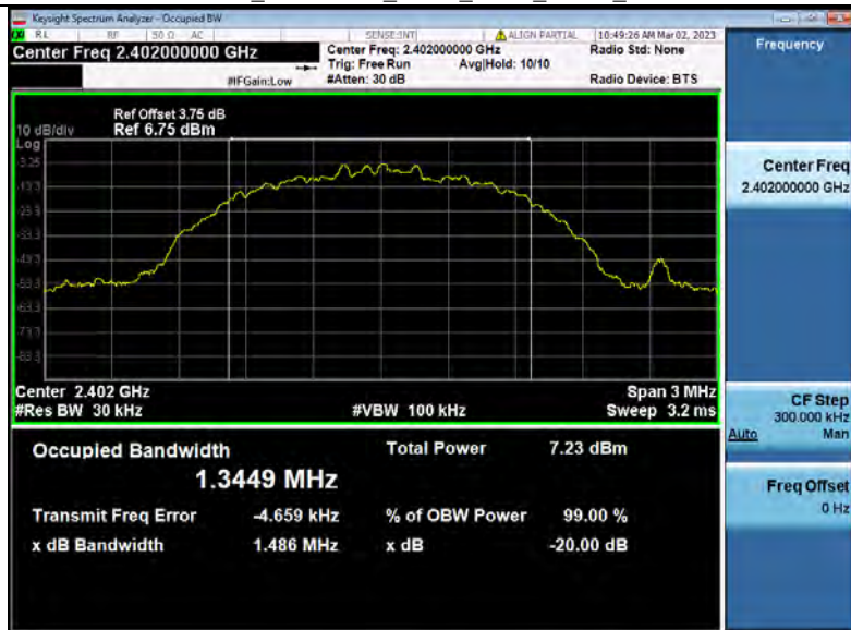
-20dB Bandwidth_NVNT_ANT1_3-DH5_2402
