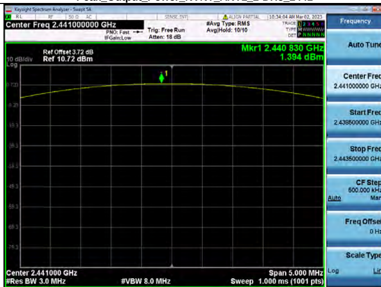
Peak_Output_Power_NVNT_ANT1_2-DH5_2441
