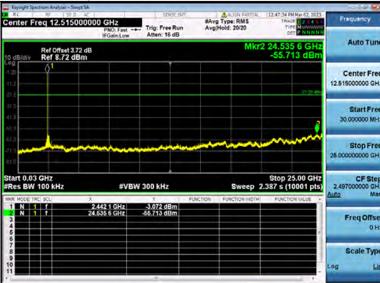
2_Spurious_Emissions_NVNT_ANT1_3-DH5_2441
