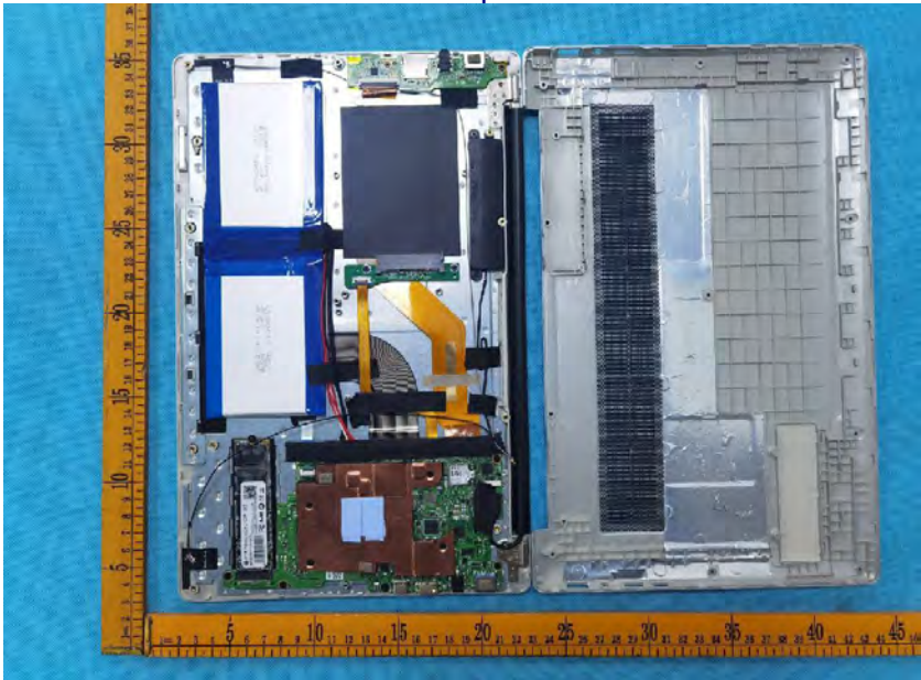
Internal photos
