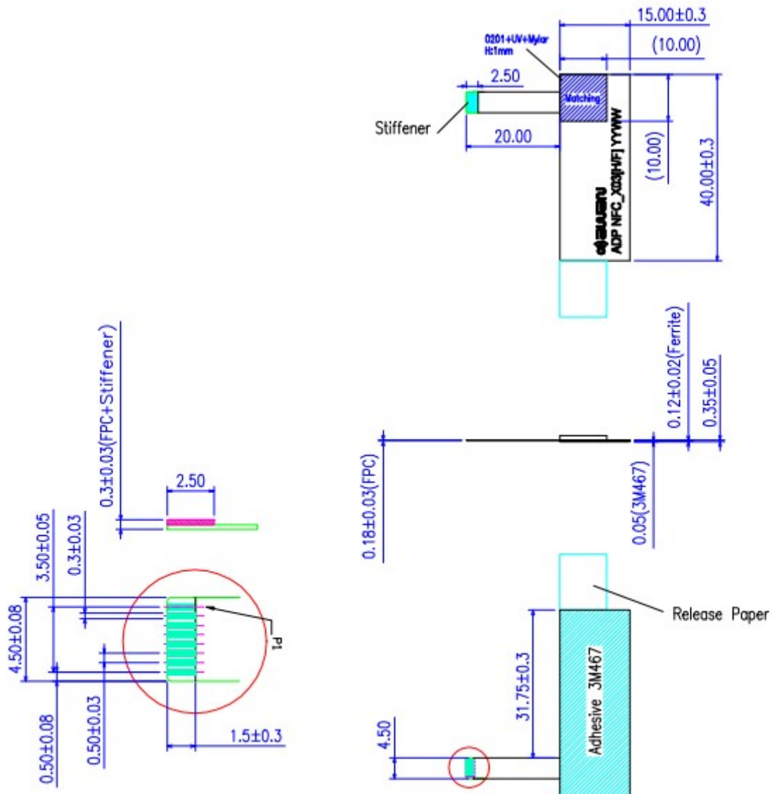
8 Pin Connector
