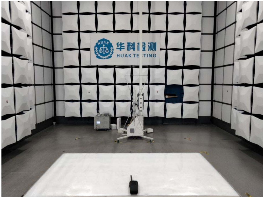
Helen 228 Radiated Emissions
